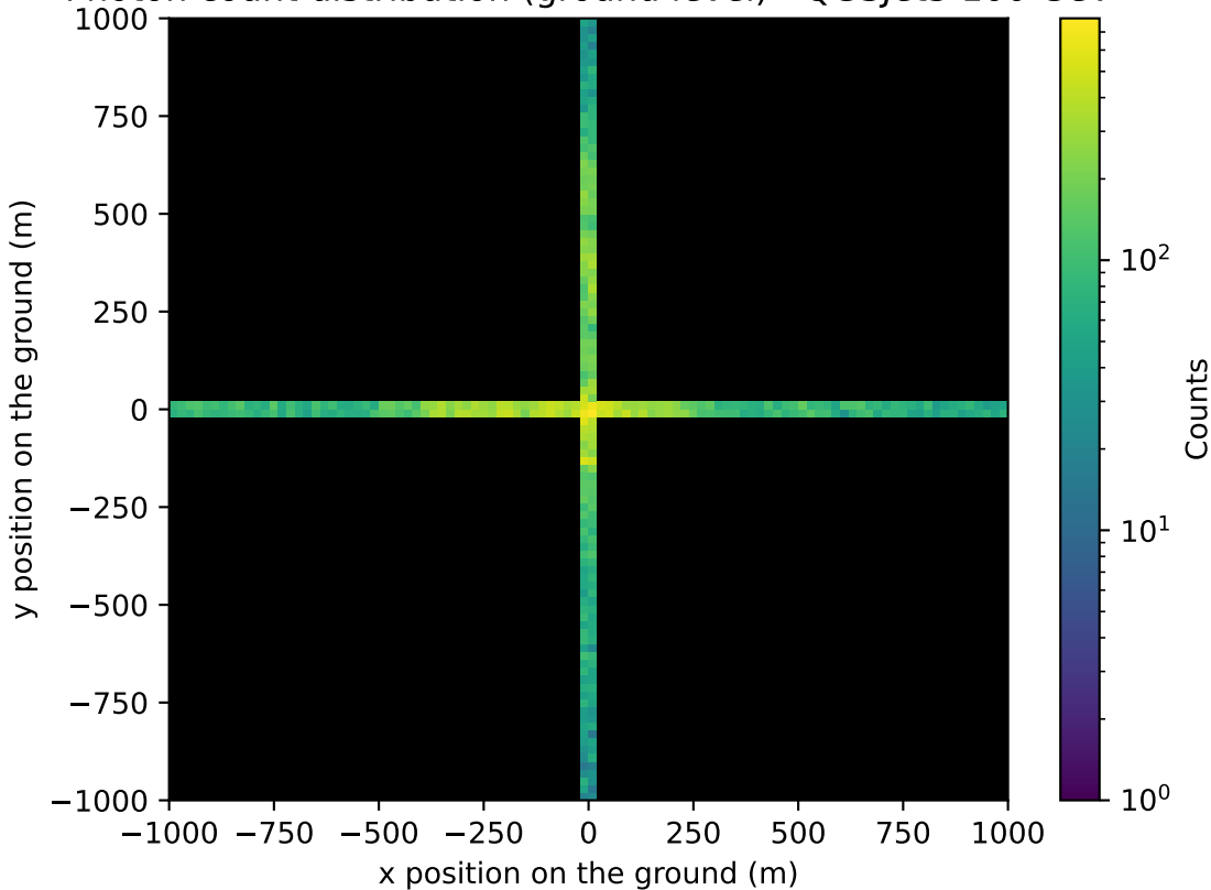
Photon count distribution (ground level) - QGSJet3 100 GeV
