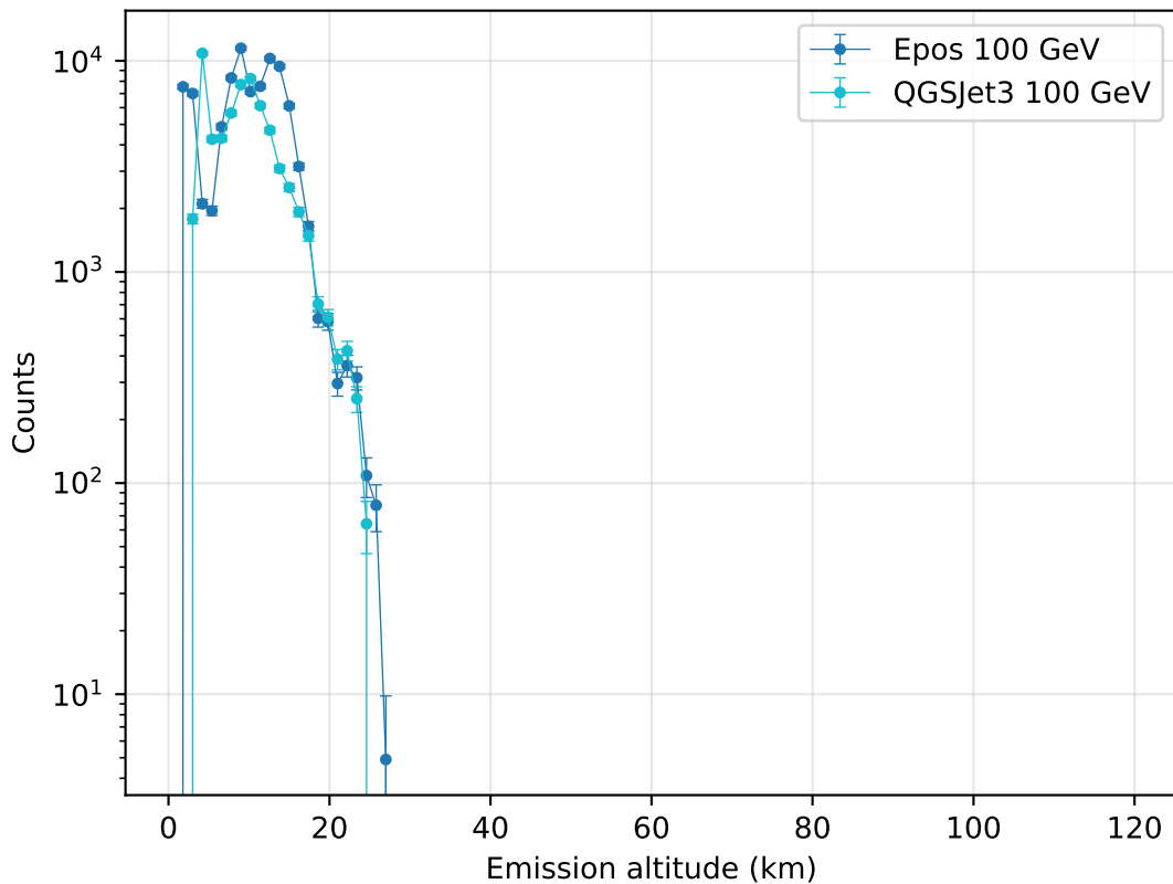
Photon emission altitude distribution
