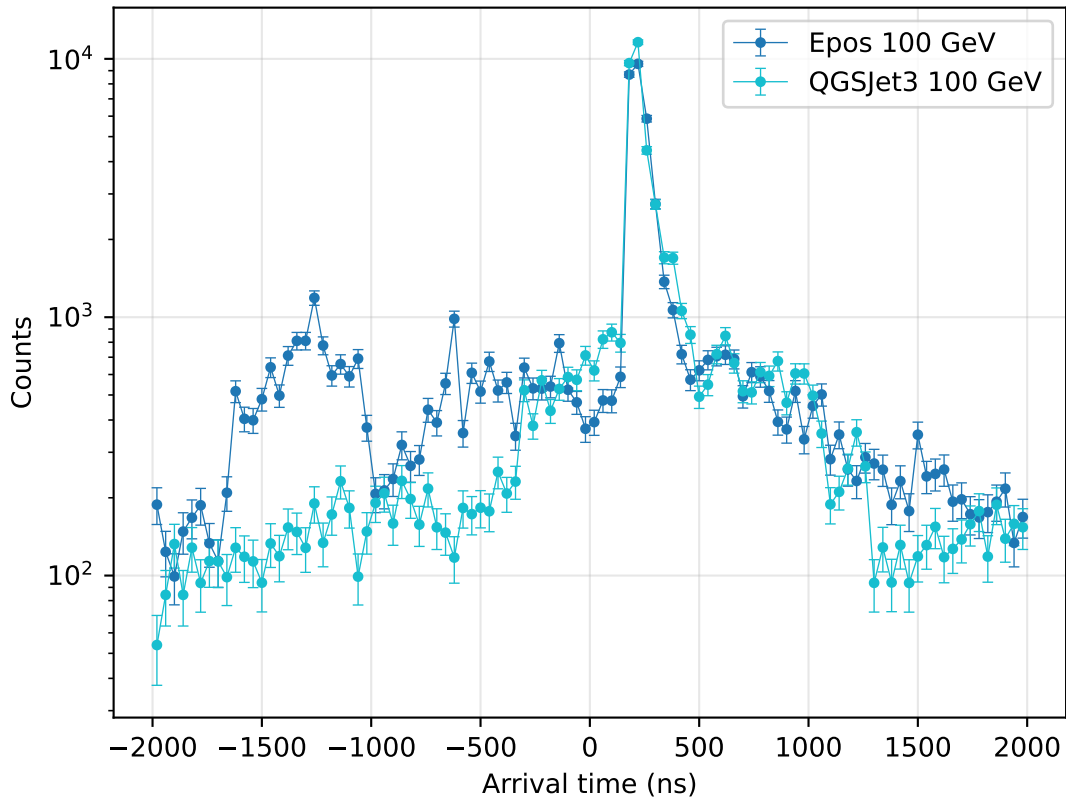
Photon arrival time distribution
