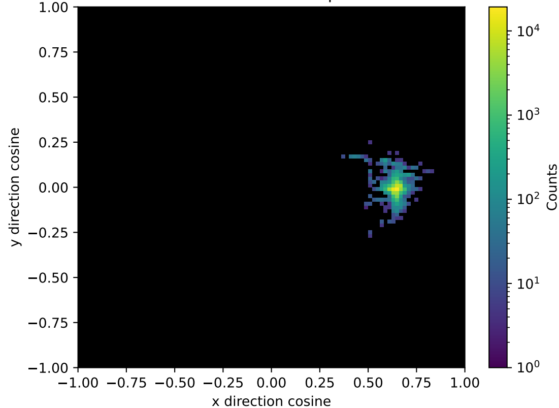
Photon arrival direction - Epos 100 GeV
