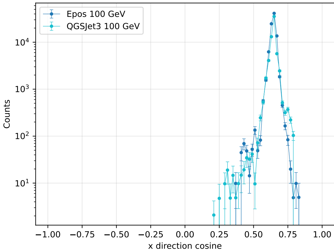
Photon direction cosine x distribution
