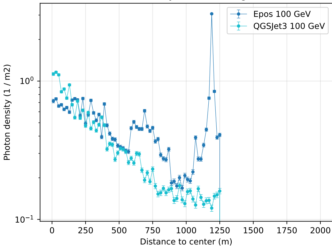
Photon lateral density distribution (ground level)
