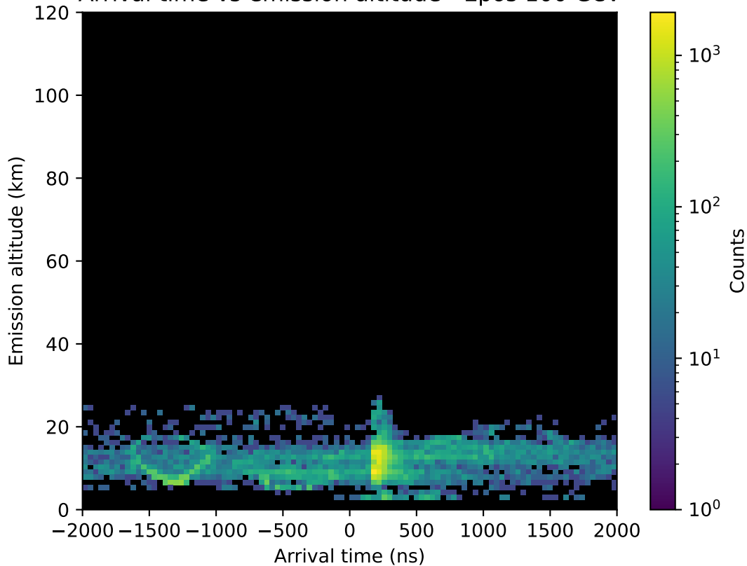
Arrival time vs emission altitude - Epos 100 GeV
