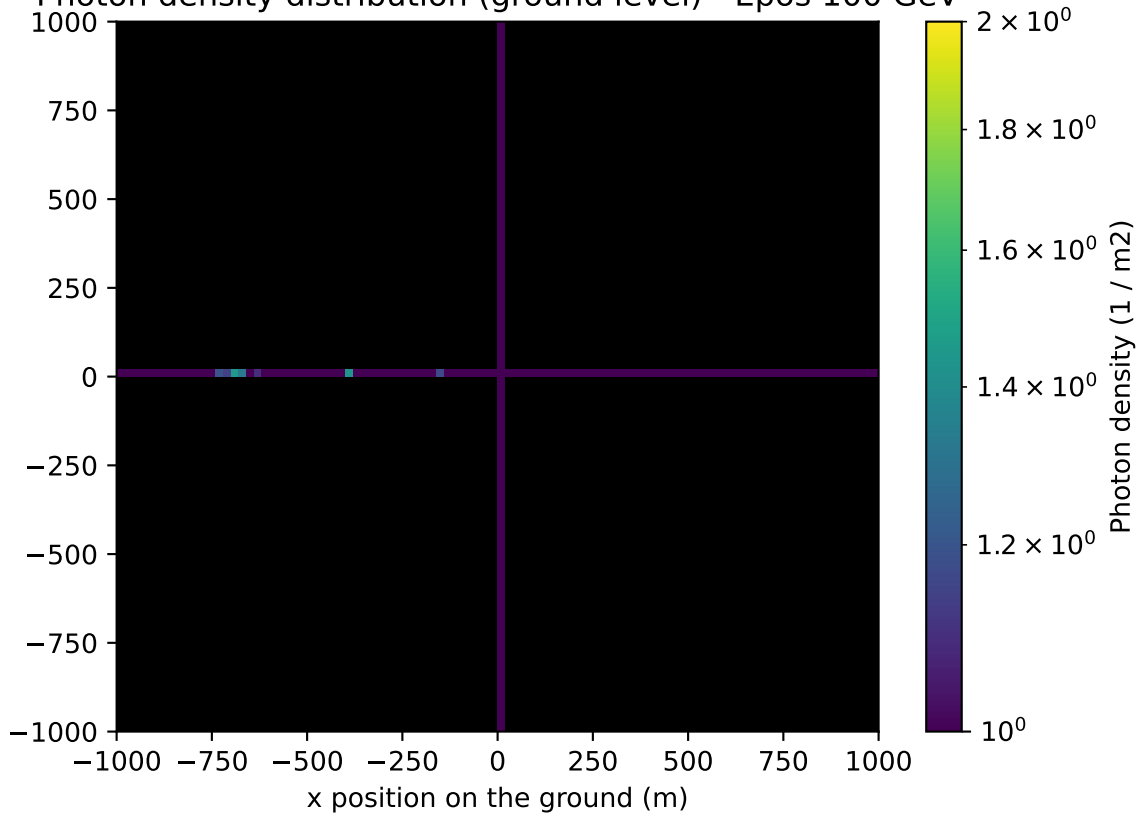
Photon density distribution (ground level) - Epos 100 GeV
