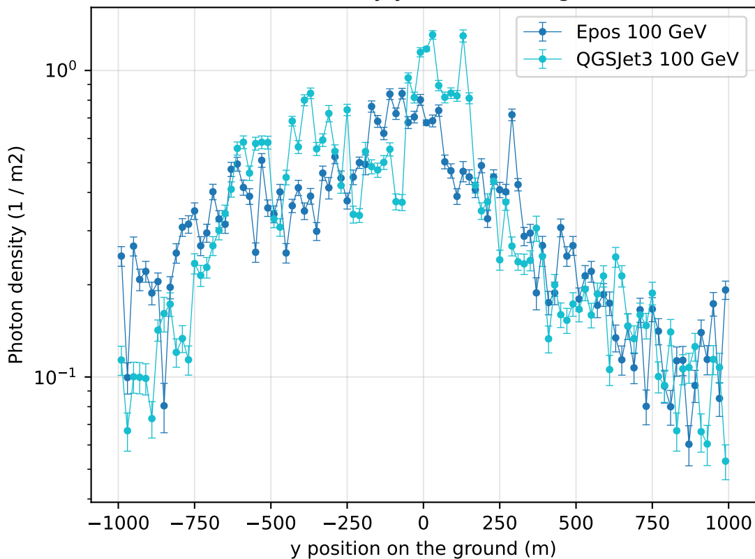
Photon lateral density y distribution (ground level)
