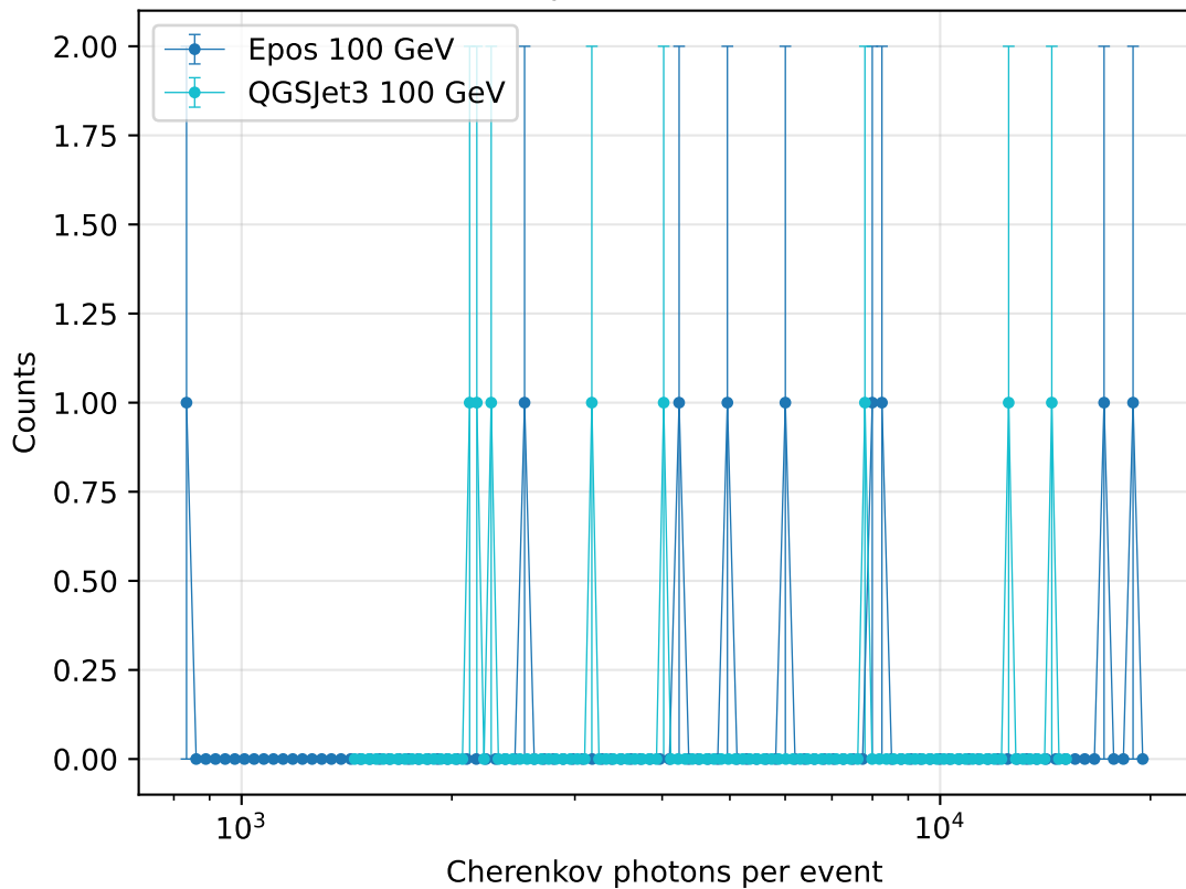
Photons per event distribution
