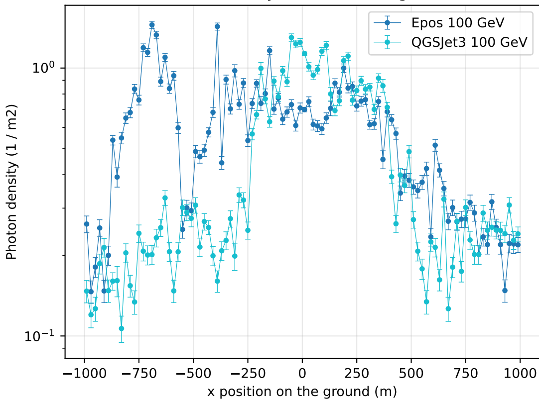
Photon lateral density x distribution (ground level)
