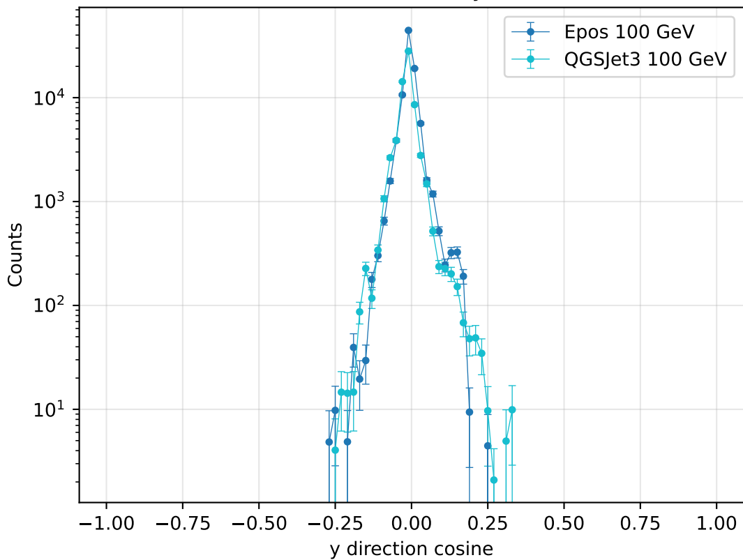
Photon direction cosine y distribution
