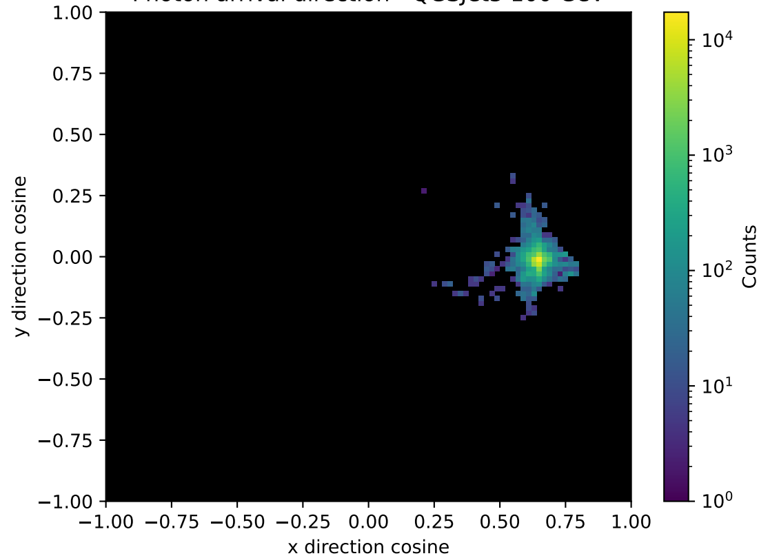
Photon arrival direction - QGSJet3 100 GeV
