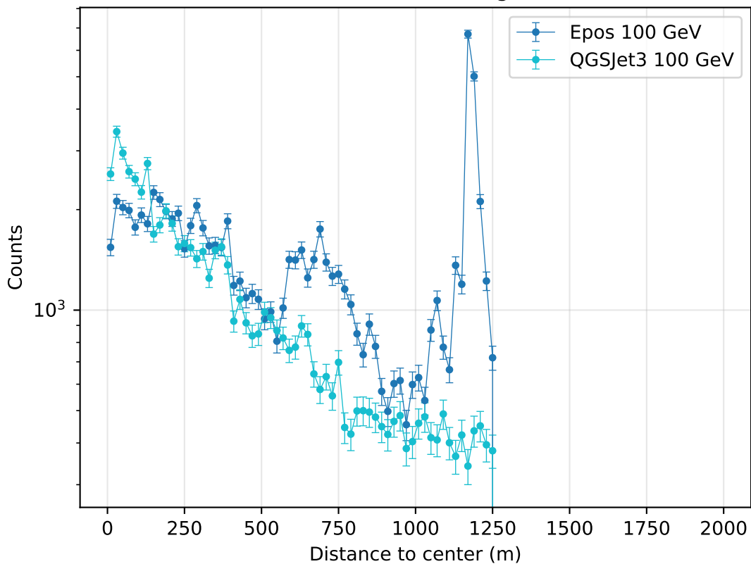
Photon lateral distribution (ground level)
