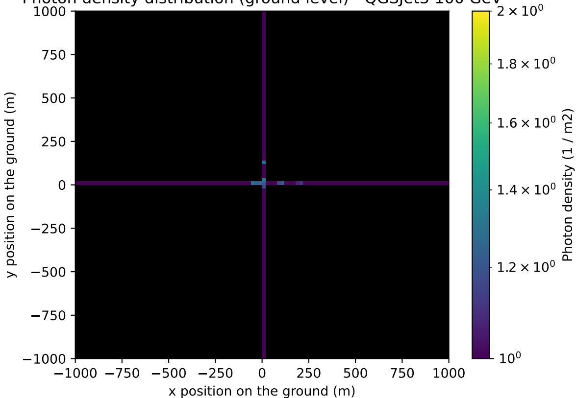
Photon density distribution (ground level) - QGSJet3 100 GeV
