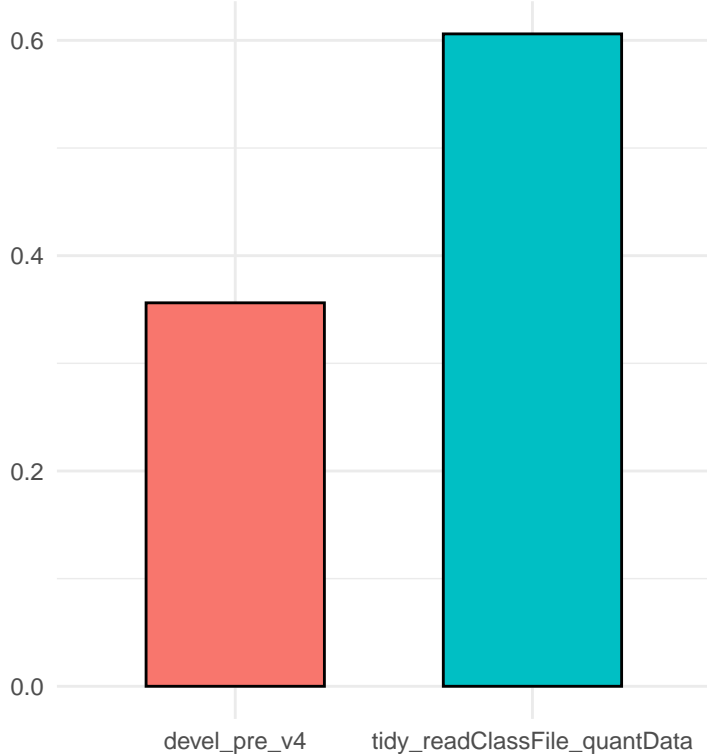
Runtime_Min
