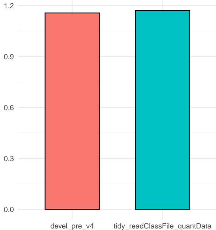
Memory_GB
