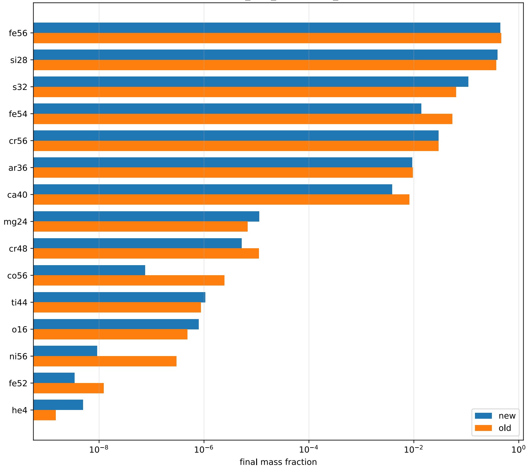
approx21_plus_co56 zsplits_3GK
