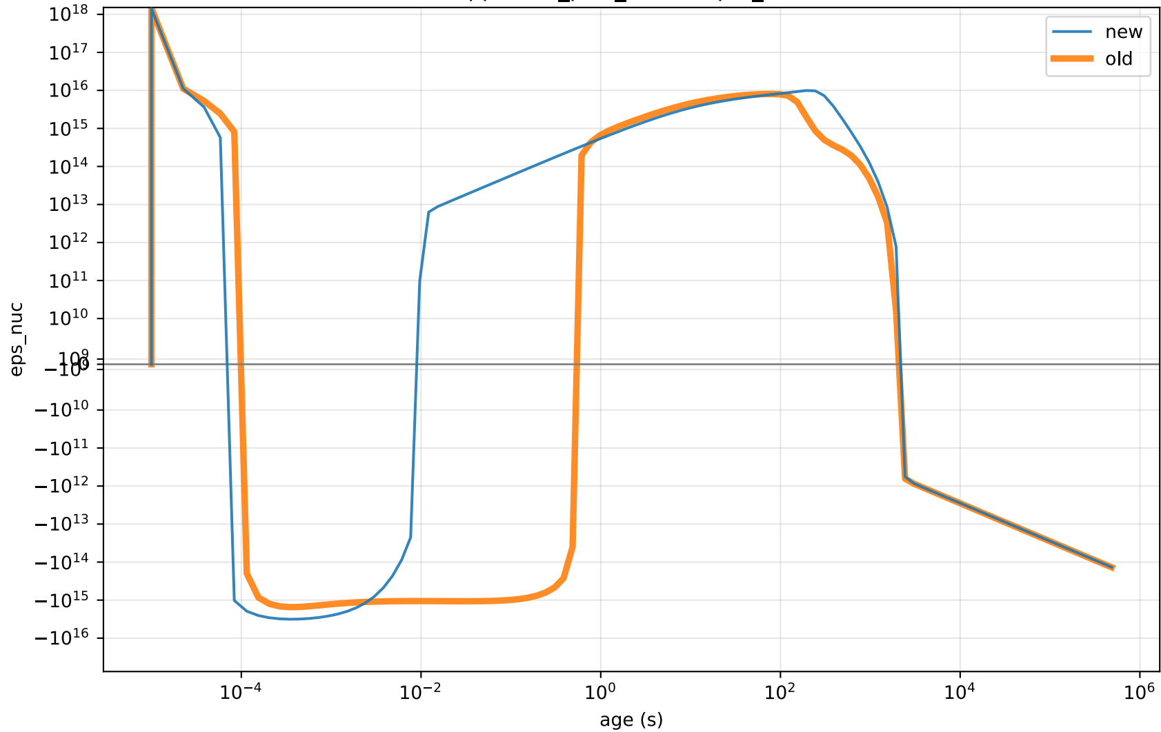
approx21_plus_co56 zsplitt_6GK
