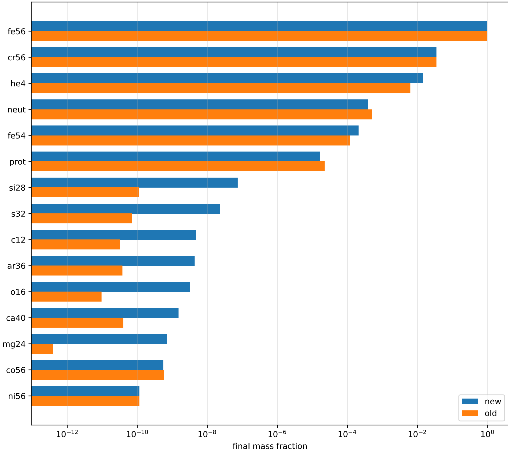
approx21_plus_co56 zsplitted_6GK
