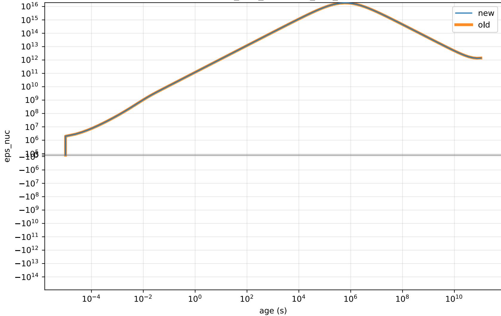
approx21_plus_co56 c12_o16_1GK
