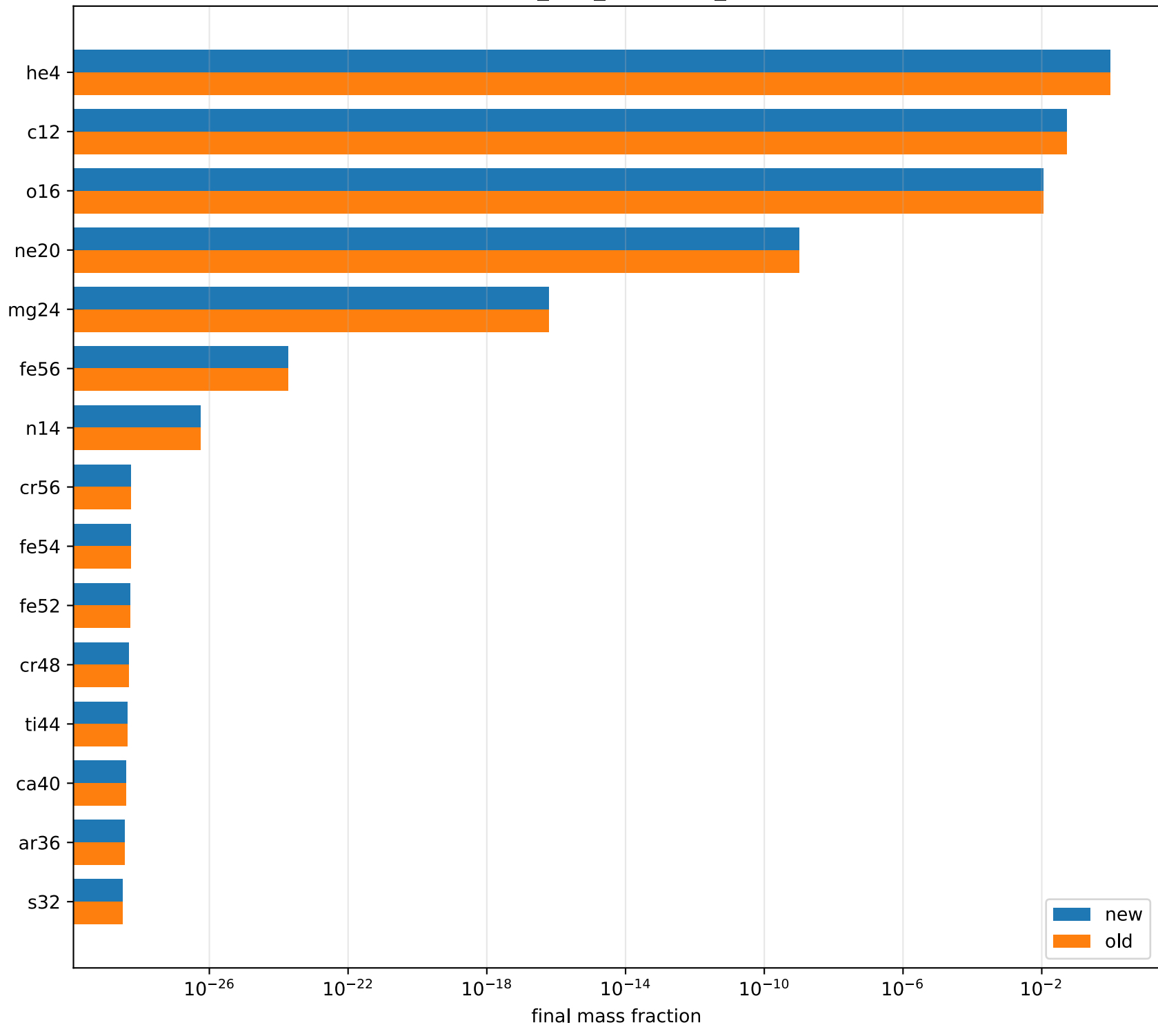
approx21_plus_co56 he4_0p1GK
