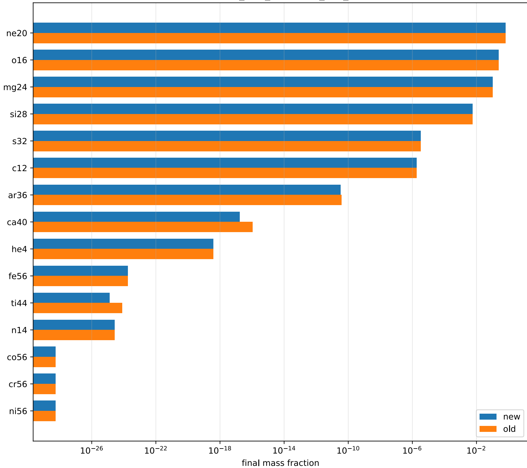
approx21_plus_co56 c12_o16_1GK
