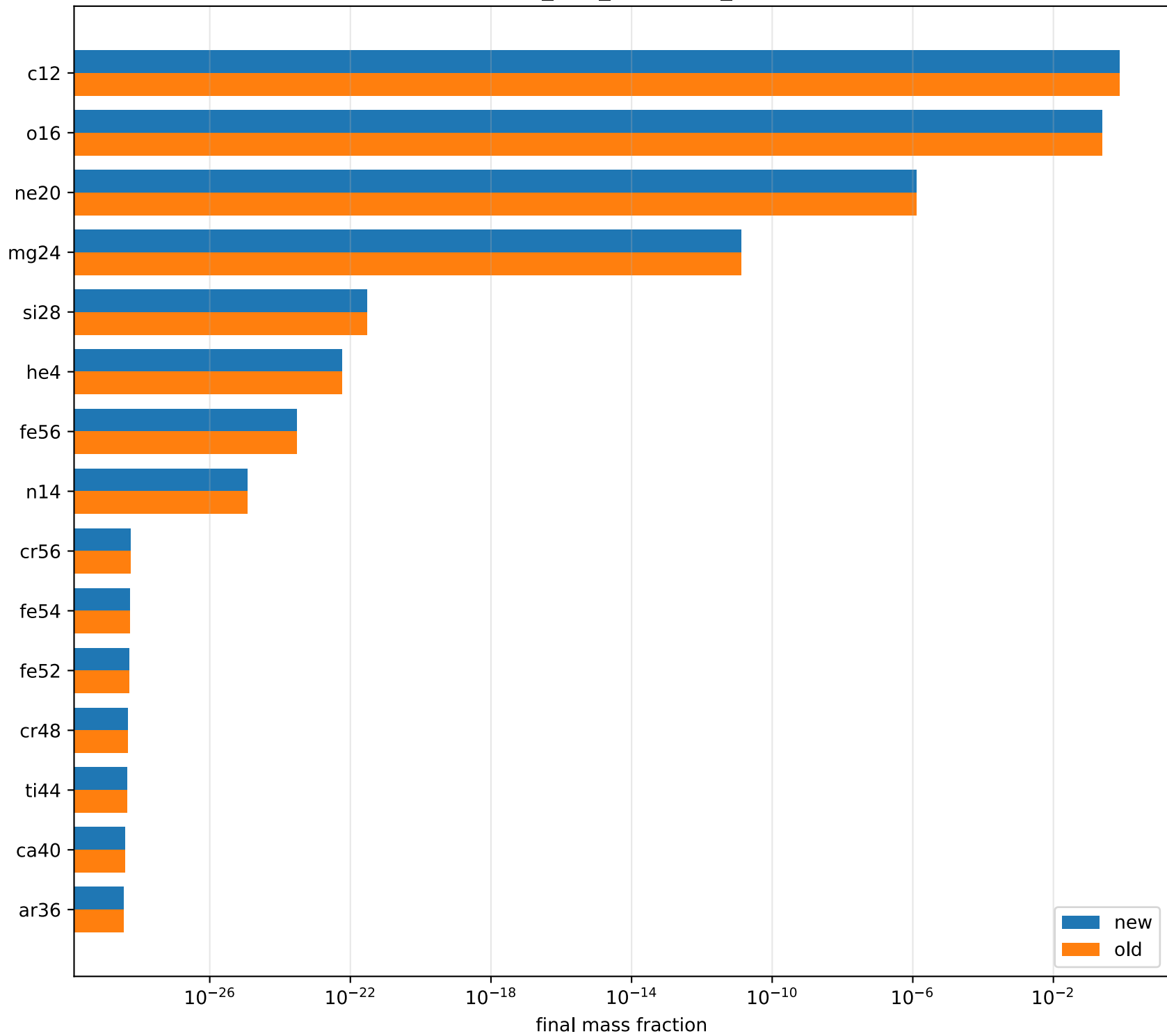
approx21_plus_co56 he4_0p2GK
