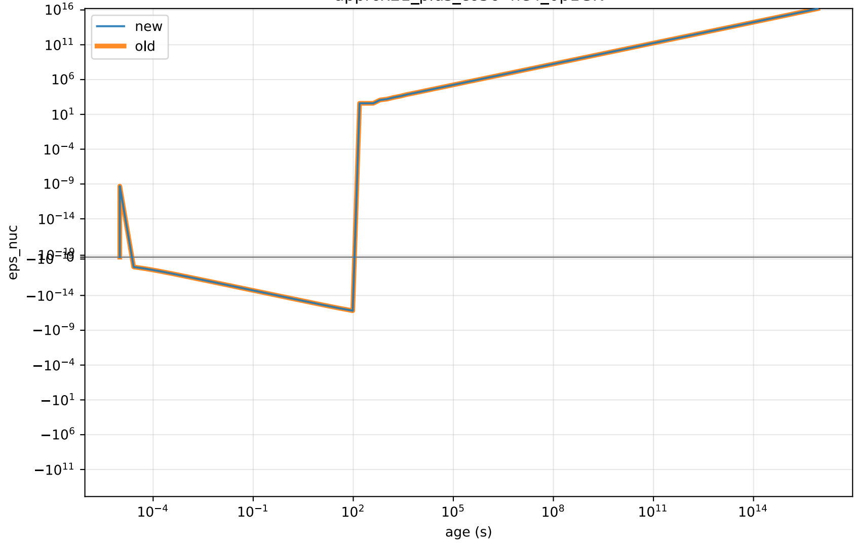
approx21_plus_co56 he4_0p1GK
