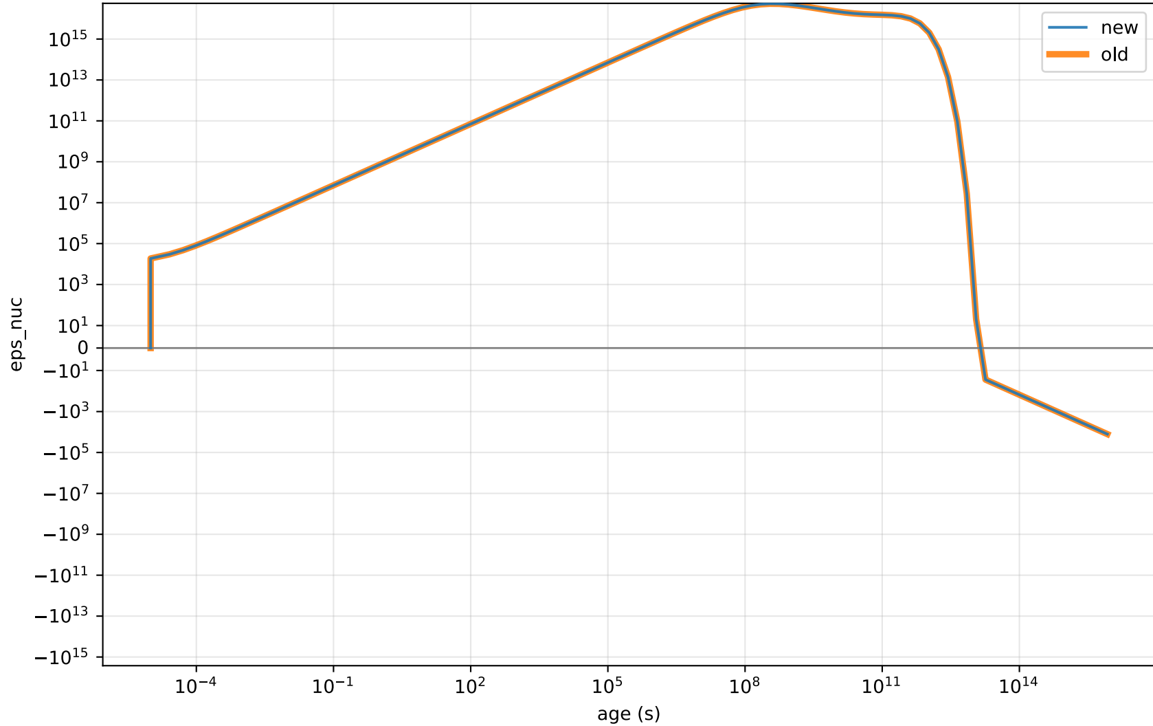
approx21_plus_co56 he4_0p2GK
