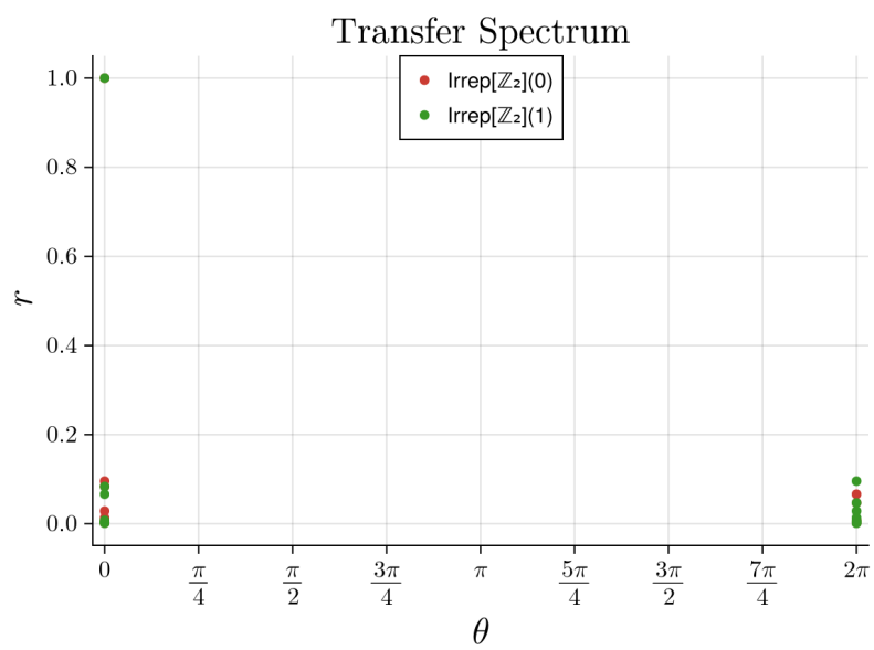
Figure 2: CairoMakie transfer plots
