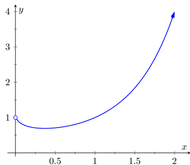
Figure 2.6.17 A plot of y = x^x
