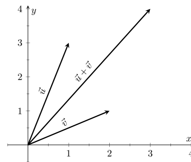
Figure 11.2.9 Graphing the sum of vectors in Example 11.2.8
