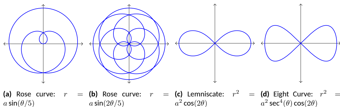
Figure 10.4.22 Special Curves
