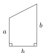
Figure 5.5.8 The area of a trapezoid
