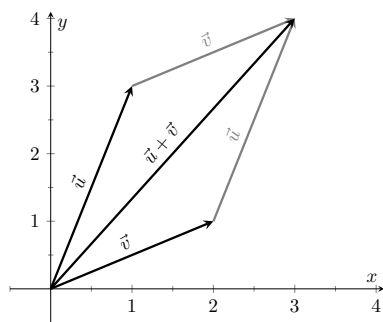
Figure 11.2.10 Illustrating how to add vectors using the Head to Tail Rule and Parallelogram Law
