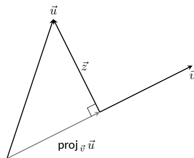
Figure 11.3.18 Illustrating the orthogonal projection
