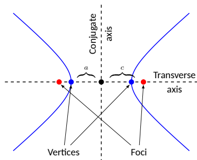
Figure 10.1.24 Labeling the significant features of a hyperbola
