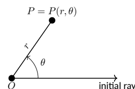
Figure 10.4.1 Illustrating polar coordinates
