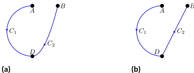
Figure 15.1.11 Illustrating properties of line integrals
