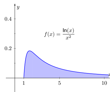
Figure 6.8.9 A graph of f(x) = \frac{\ln(x)}{x^2} in Example 6.8.8
