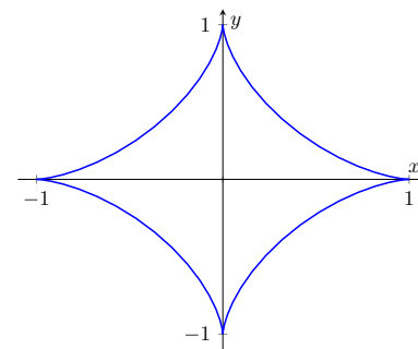
Figure 10.3.8 A graph of an astroid
