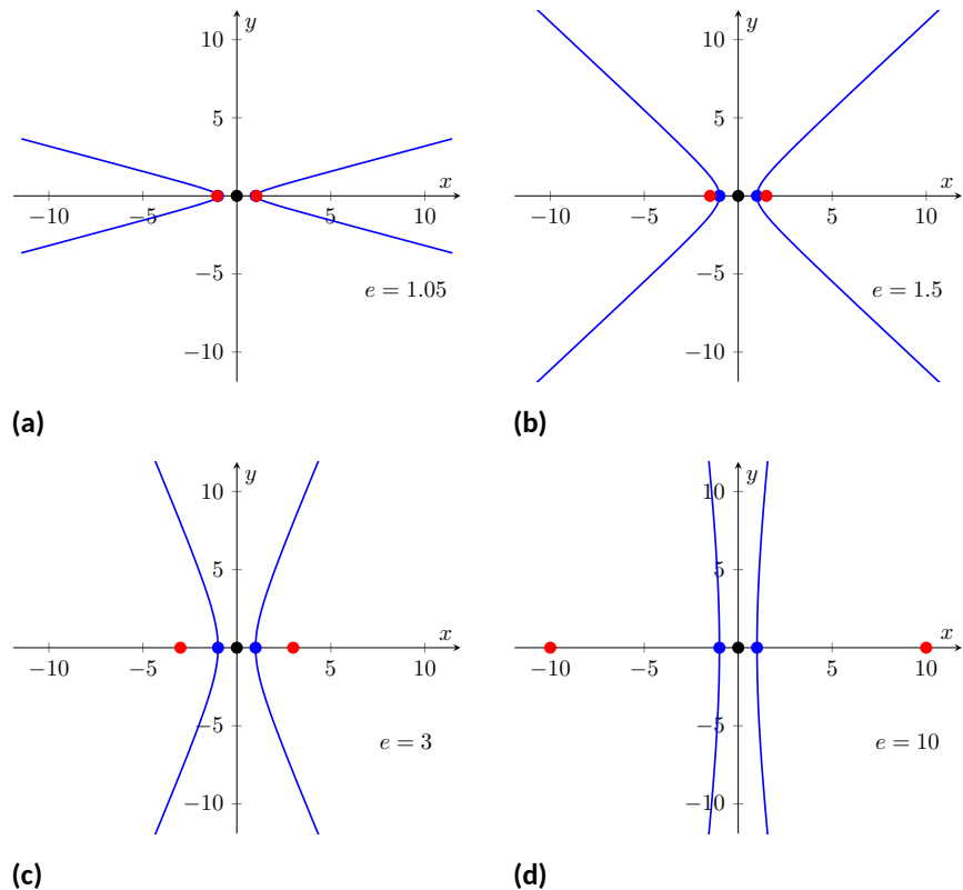
Figure 10.1.33 Understanding the eccentricity of a hyperbola
