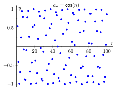
Figure 9.1.13 Scatter plot for the sequence in Item 2 of Example 9.1.11
