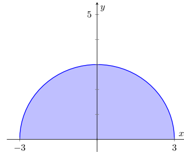
Figure 5.2.14 f(x) = \sqrt{9 - x^2}
