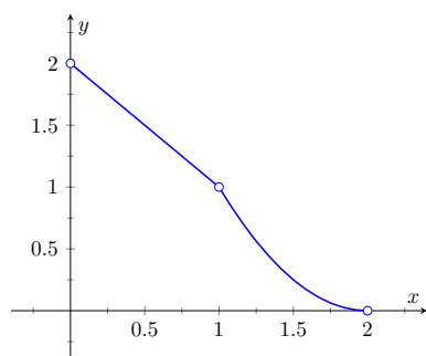
Figure 1.4.6 A graph of f from Example 1.4.5
