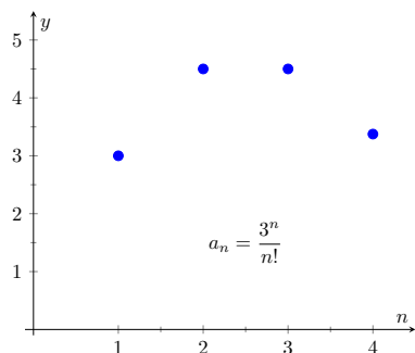
Figure 9.1.4 Plotting the sequence in Item 1 of Example 9.1.3
