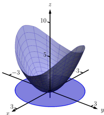
Figure 15.5.6 The surface parametrized in Example 15.5.5
