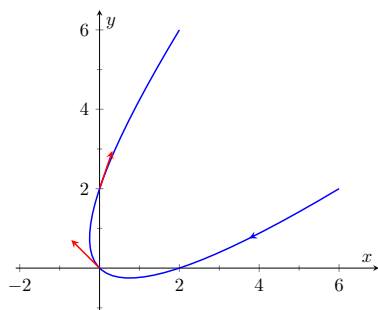
Figure 12.4.5 Plotting unit tangent vectors in Example 12.4.4
