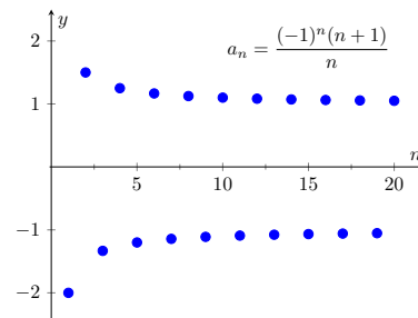
Figure 9.1.17 A plot of a sequence in Example 9.1.16, part 2
