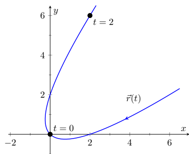
Figure 12.4.16 Graphing \vec{r}(t) in Example 12.4.15
