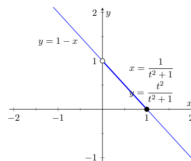
Figure 10.2.16 Graphing parametric and rectangular equations for a graph in Example 10.2.15
