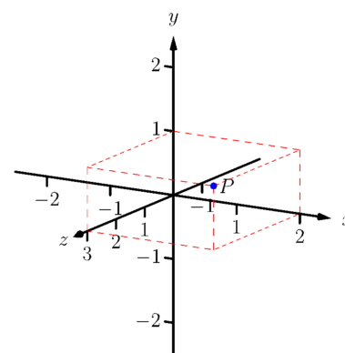
Figure 11.1.1 Plotting the point P = (2, 1, 3) in space
