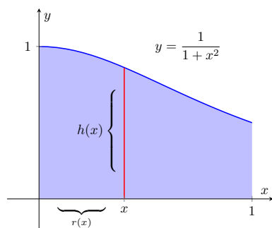
Figure 7.3.5 Graphing a region in Example 7.3.4
