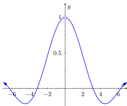
Figure 1.1.1 \sin(x)/x
