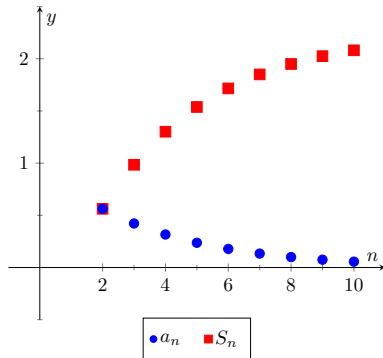
Figure 9.2.7 Scatter plots for the series in Item 1
