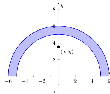
Figure 14.4.22 Illustrating the region R in Example 14.4.21
