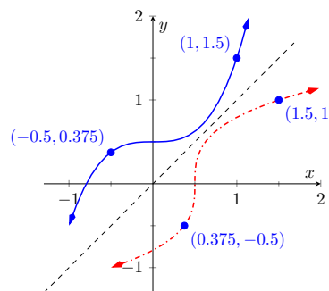
Figure 2.7.1 A function f along with its inverse f^{-1} . (Note how it does not matter which function we refer to as f ; the other is f^{-1} .)
