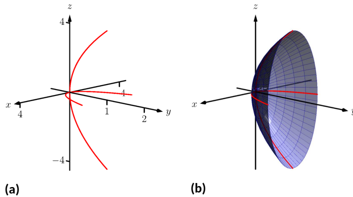
Figure 11.1.27 Sketching an elliptic paraboloid
