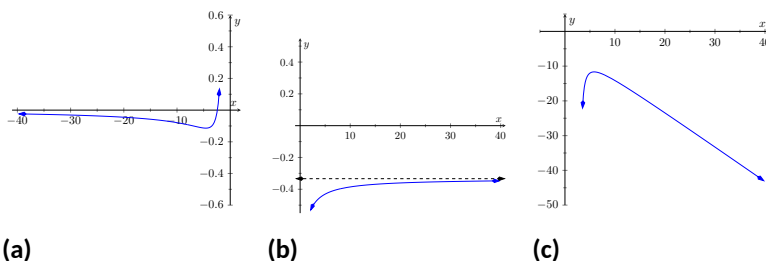
Figure 1.6.19 Visualizing the functions in Example 1.6.18
