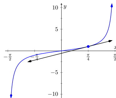
Figure 2.4.11 A graph of y = \tan(x) along with its tangent line at x = \pi/4
