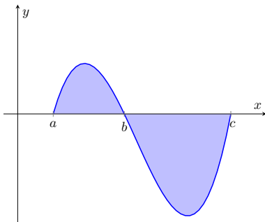
Figure 5.2.11 A graph of a function in Example 5.2.10
