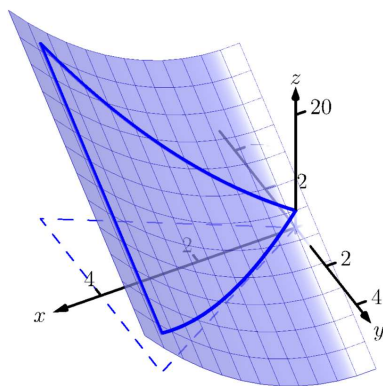
Figure 14.5.9 Graphing the surface in Example 14.5.8
