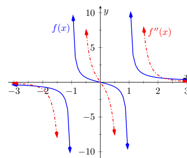
Figure 3.4.16 A graph of f(x) and f''(x) in Example 3.4.14
