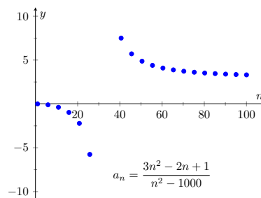
Figure 9.1.12 Scatter plot for the sequence in Item 1 of Example 9.1.11
