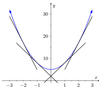
Figure 3.4.4 A function f with a concave up graph. Notice how the slopes of the tangent lines, when looking from left to right, are increasing. (The slope values pictured are -12 , -6 , 6 and 12 ).
