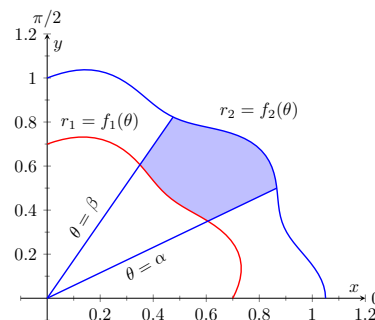
Figure 10.5.11 Illustrating area bound between two polar curves
