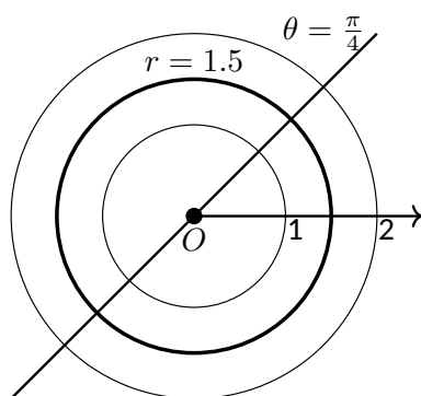
Figure 10.4.9 Plotting standard polar plots
