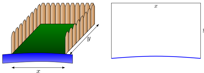
Figure 4.3.5 A sketch of the enclosure in Example 4.3.4
