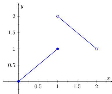
Figure 1.4.3 A graph of f in Example 1.4.2
