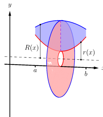
Figure 7.2.12 Establishing the Washer Method; see also Figure 7.2.11
