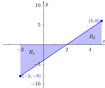
Figure 5.2.13 f(x) = 2x - 4
