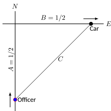
Figure 4.2.5 A sketch of a police car (at bottom) attempting to measure the speed of a car (at right) in Example 4.2.4
