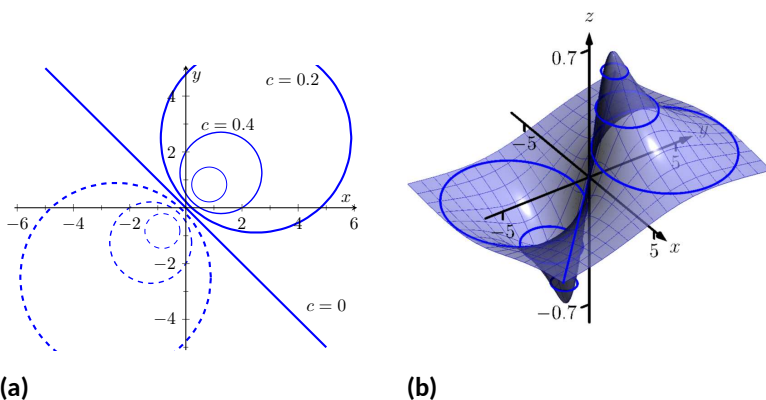
Figure 13.1.10 Graphing the level curves in Example 13.1.9
