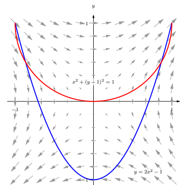
Figure 15.3.6 Paths through a vector field in Example 15.3.5
