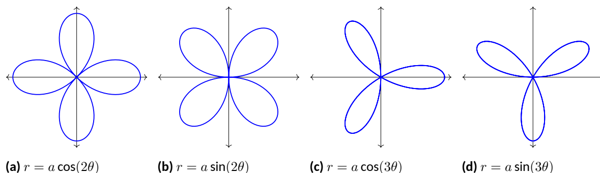
Figure 10.4.21 Rose curves
