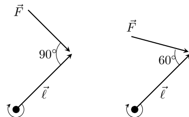
Figure 11.4.17 Showing a force being applied to a lever in Example 11.4.16
