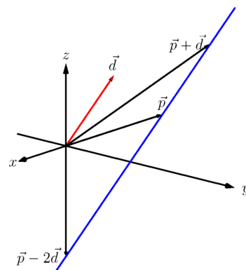
Figure 11.5.1 Defining a line in space
