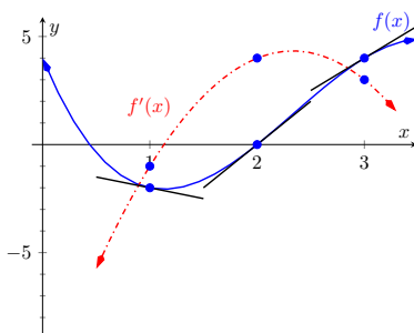
Figure 2.2.9 Graphs of f and f' in Example 2.2.7
