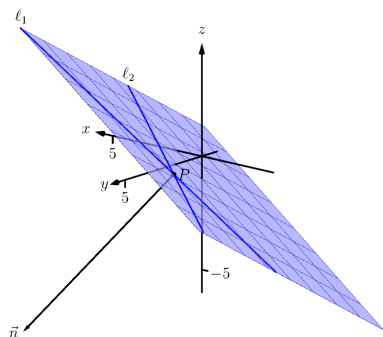
Figure 11.6.6 Sketching the plane in Example 11.6.5
