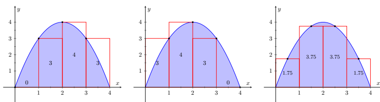
(a) using the Left Hand Rule
