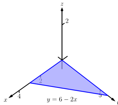
Figure 14.6.8 The region D used in Example 14.6.7
