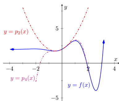
Figure 9.7.3 Plotting f , p_2 and p_4
