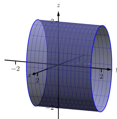
Figure 15.5.13 The cylinder parametrized in Example 15.5.12
