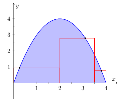
Figure 5.3.14 An example of a general Riemann sum to approximate \int_0^4 (4x - x^2) dx
