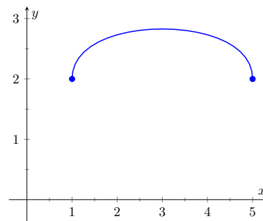
Figure 1.5.11 A graph of f(x) = \sqrt{x-1} + \sqrt{5-x}
