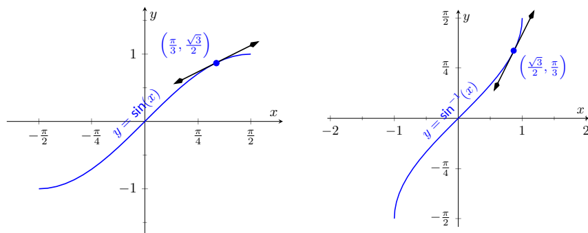
Figure 2.7.7 Graphs of \sin(x) and \sin^{-1}(x) along with corresponding tangent lines
