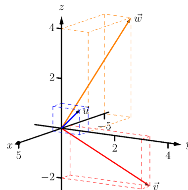
Figure 11.3.10 Vectors used in Example 11.3.9
