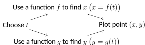
Figure 10.2.2 Plotting a curve (x(t), y(t))
