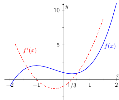
Figure 3.3.9 A graph of f(x) in Example 3.3.6, showing where f is increasing and decreasing
