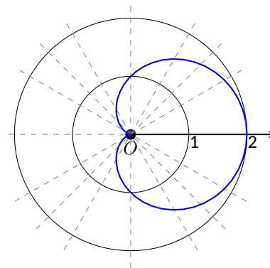
Figure 10.4.12 Using technology to graph a polar function
