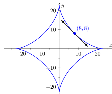
Figure 2.6.15 An astroid with a tangent line
