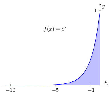
Figure 6.8.6 A graph of f(x) = e^x in Example 6.8.3
