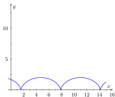
Figure 12.1.12 The cycloid in Example 12.1.10
