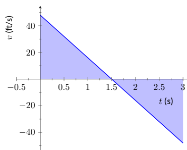
Figure 5.2.4 A graph of v(t) = -32t + 48 ; the shaded areas help determine displacement
