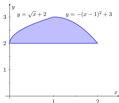
Figure 7.1.8 Graphing a region for Example 7.1.7
