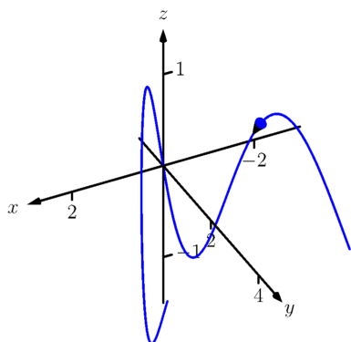
Figure 12.3.16 The path of the particle in Example 12.3.15
