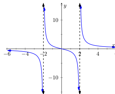
Figure 1.6.10 Graphing f(x) = \frac{3x}{x^2 - 4}
