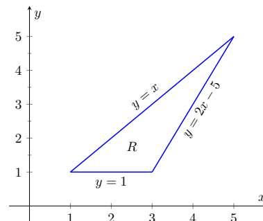
Figure 14.1.11 Calculating the area of a triangle with iterated integrals in Example 14.1.10
