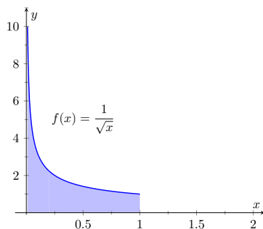
Figure 6.8.12 A graph of f(x) = \frac{1}{\sqrt{x}} in Example 6.8.11
