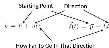
Figure 11.5.2 Understanding the vector equation of a line
