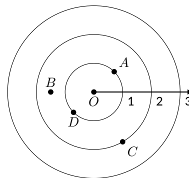
Figure 10.4.3 Plotting polar points in Example 10.4.2
