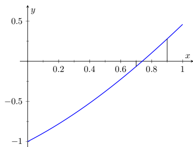
Figure 1.5.16 Graphing a root of f(x) = x - \cos(x)
