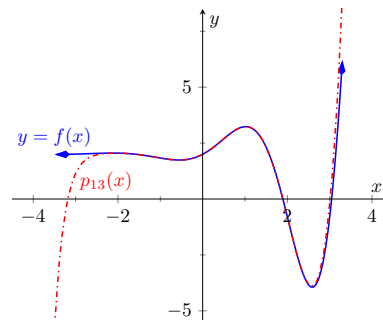
Figure 9.7.4 Plotting f and p_{13}
