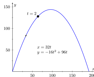
Figure 10.2.14 Graphing projectile motion in Example 10.2.13
