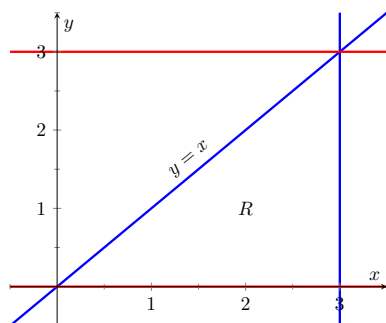
Figure 14.2.18 Determining the region R determined by the bounds of integration in Example 14.2.17
