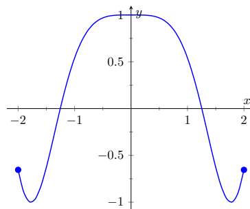
Figure 3.1.23 A graph of f(x) = \cos(x^2) on [-2, 2] as in Example 3.1.21
