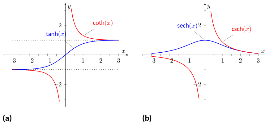
Figure 6.6.4 Graphs of \tanh(x) , \operatorname{coth}(x) , \operatorname{csch}(x) and \operatorname{sech}(x)
