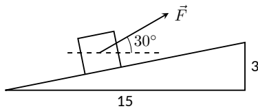
Figure 11.3.26 Computing work when sliding a box up a ramp in Example 11.3.25
