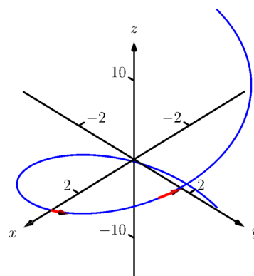
Figure 12.4.3 Plotting unit tangent vectors in Example 12.4.2
