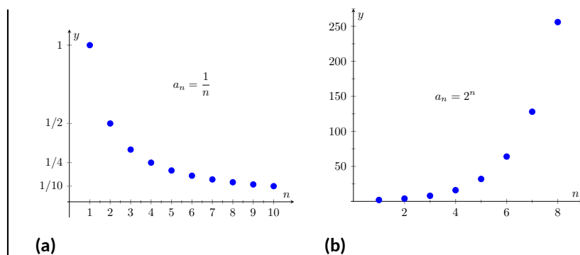
Figure 9.1.22 A plot of \{a_n\} = \{1/n\} and \{a_n\} = \{2^n\} from Example 9.1.21
