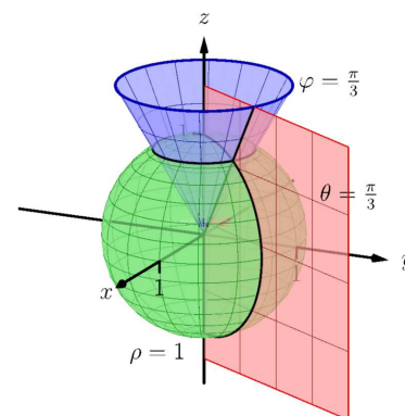
Figure 14.7.15 Graphing the canonical surfaces in spherical coordinates from Example 14.7.14
