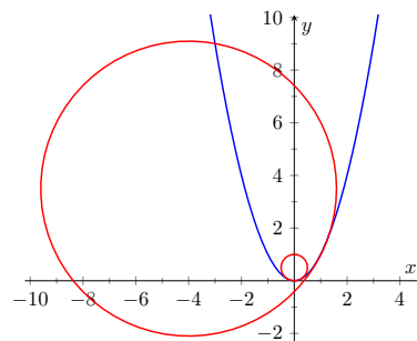
Figure 12.5.12 Examining the curvature of y = x^2
