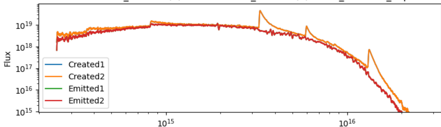
sirocco-macro_260528 (1) vs sirocco-1.3_260526 (2) for cv_standard_import
