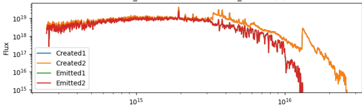
sirocco-macro_260528 (1) vs sirocco-1.3_260526 (2) for two
