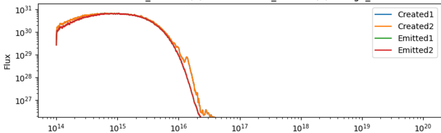
sirocco-macro_260528 (1) vs sirocco-1.3_260526 (2) for agn_macro
