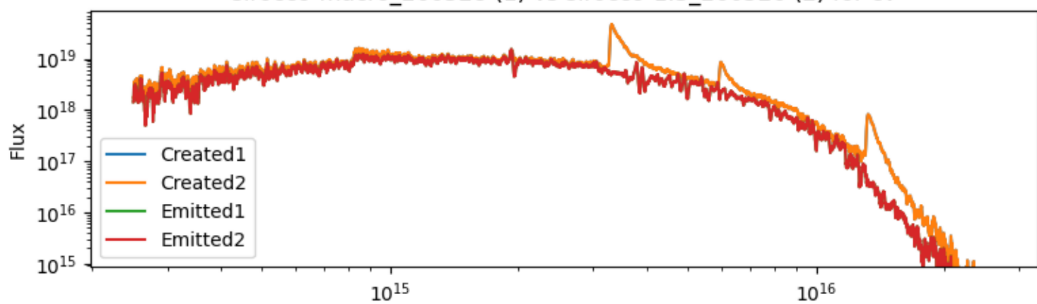
sirocco-macro_260528 (1) vs sirocco-1.3_260526 (2) for cv
