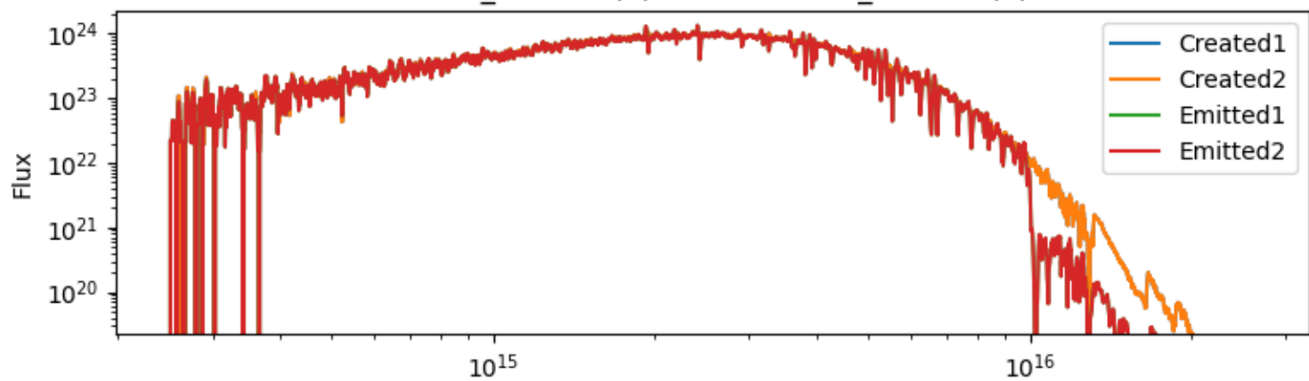
sirocco-macro_260528 (1) vs sirocco-1.3_260526 (2) for star
