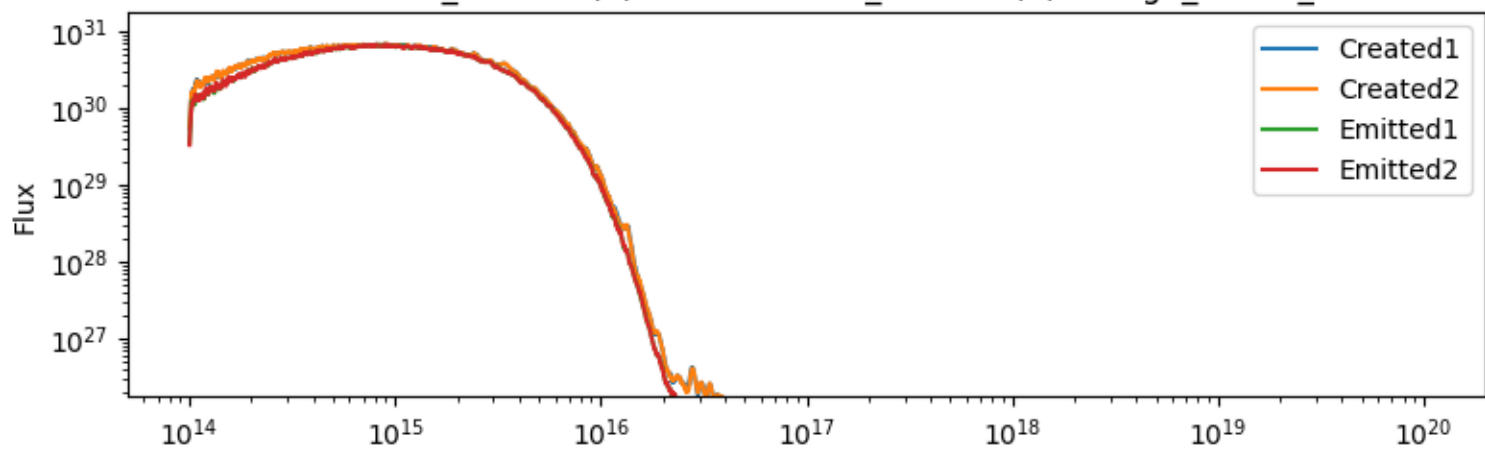
sirocco-macro_260528 (1) vs sirocco-1.3_260526 (2) for agn_macro_multi
