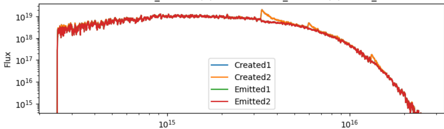
sirocco-macro_260528 (1) vs sirocco-1.3_260526 (2) for cv_vert
