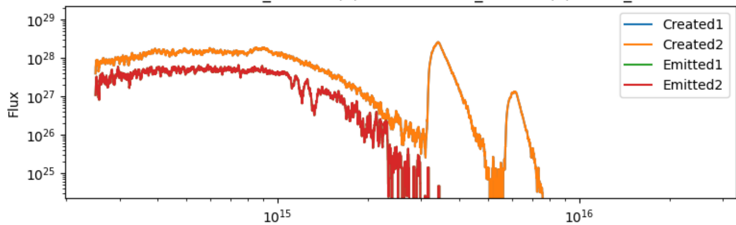
sirocco-macro_260528 (1) vs sirocco-1.3_260526 (2) for 1d_sn
