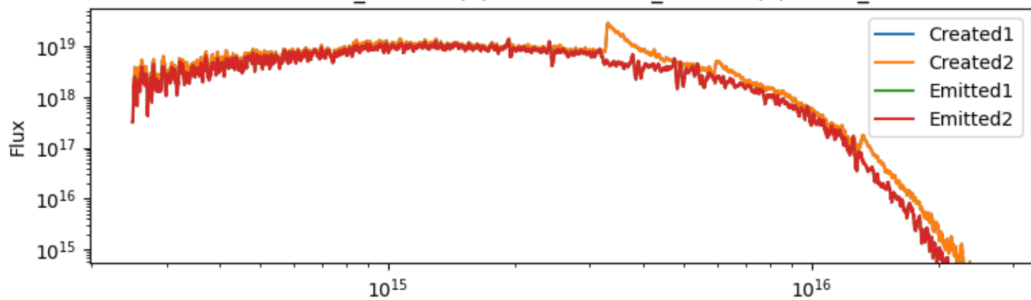
sirocco-macro_260528 (1) vs sirocco-1.3_260526 (2) for cv_multi
