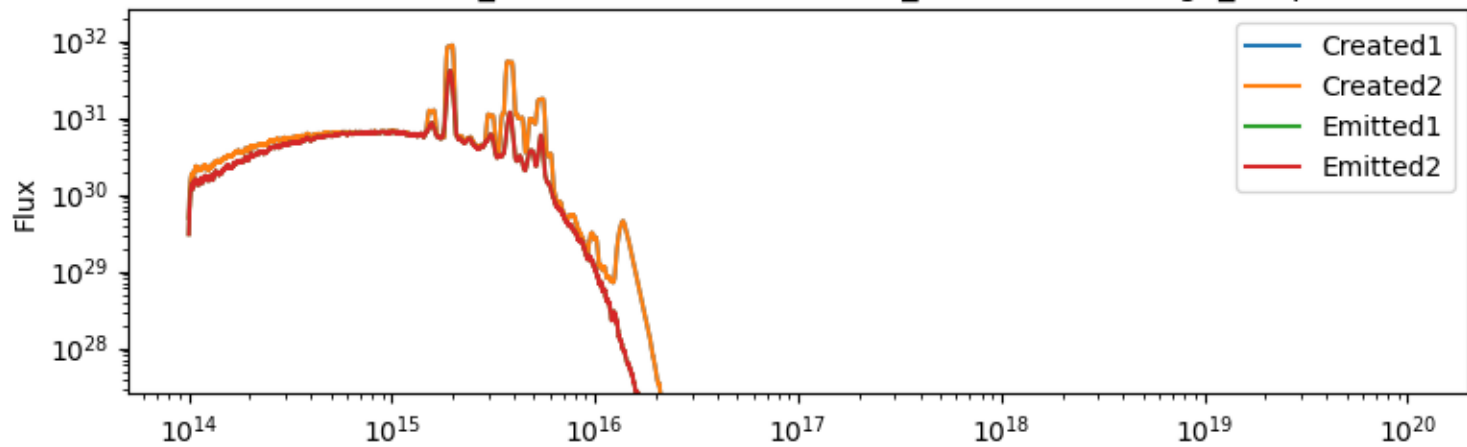
sirocco-macro_260528 (1) vs sirocco-1.3_260526 (2) for agn_simple
