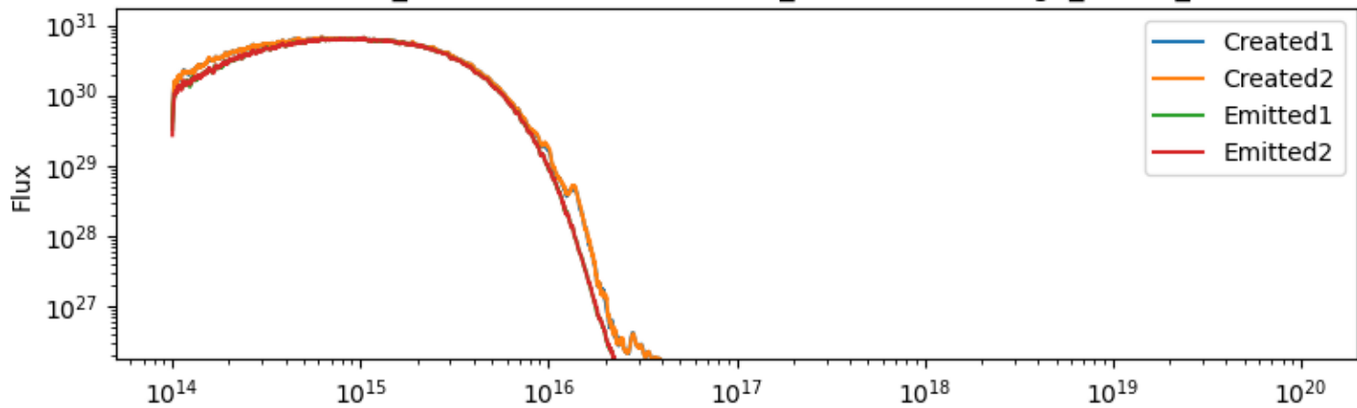
sirocco-macro_260528 (1) vs sirocco-1.3_260526 (2) for agn_macro_matrix
