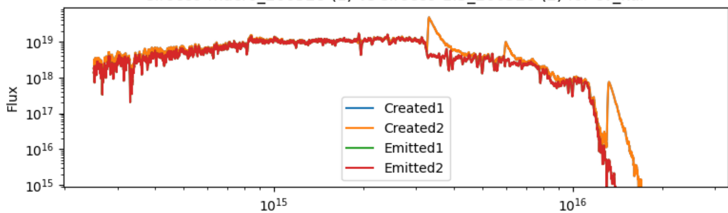
sirocco-macro_260528 (1) vs sirocco-1.3_260526 (2) for cv_kur
