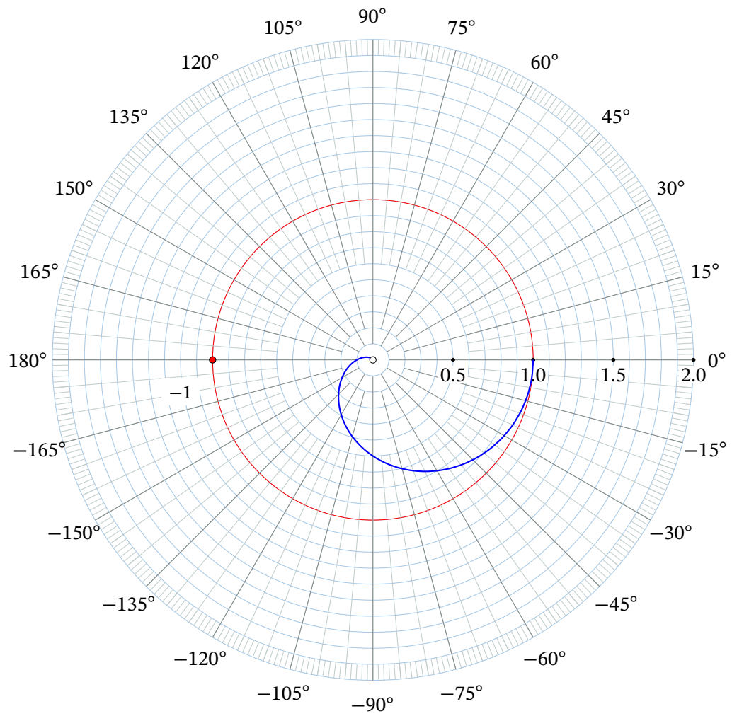
Figure 6.5.: Nyquist plot for equation (6.42)
