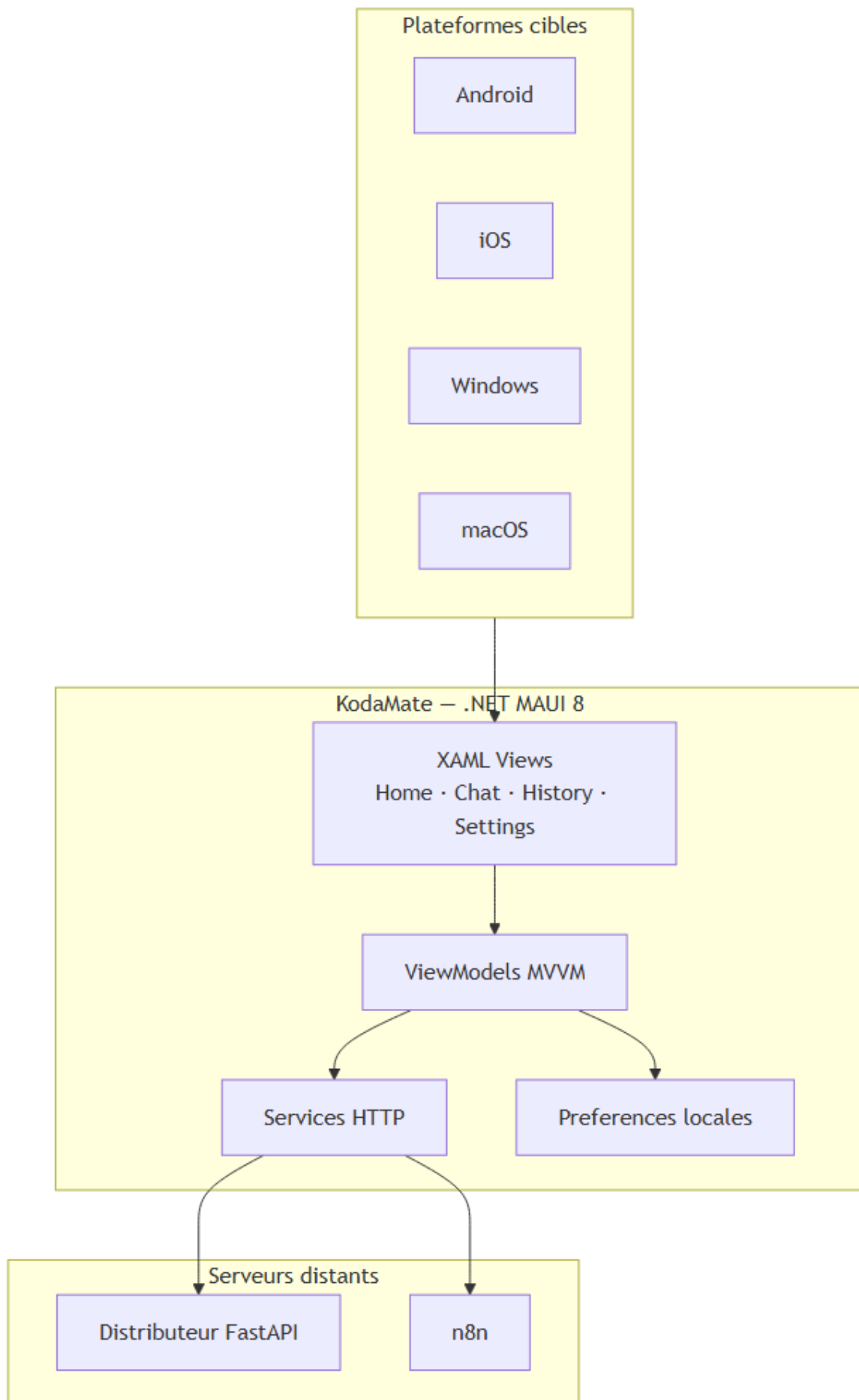
FIGURE VII.1 – Cycle 5 — pile cross-plateforme de KodaMate
