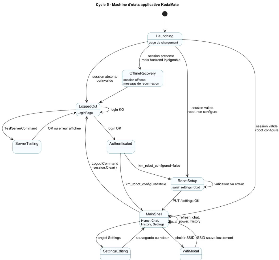
FIGURE VII.9 – Cycle 5 — machine d'états applicative KodaMate
