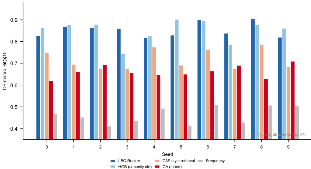
10-seed ranking performance
