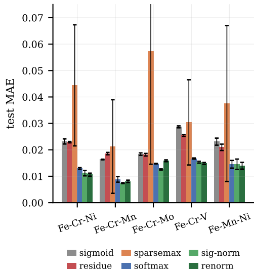
(a) neural heads (mean \pm s.d., 3 seeds)
