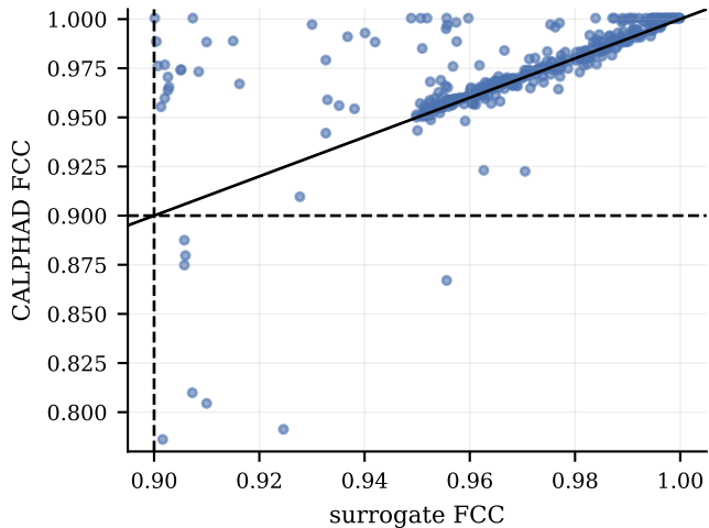
(b) parity on validated shortlist (cutoffs dashed)
