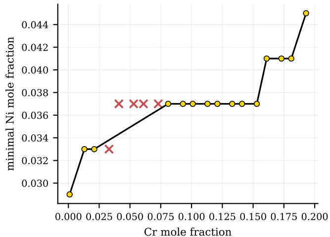
(a) quaternary frontier: Ni minimum vs Cr
