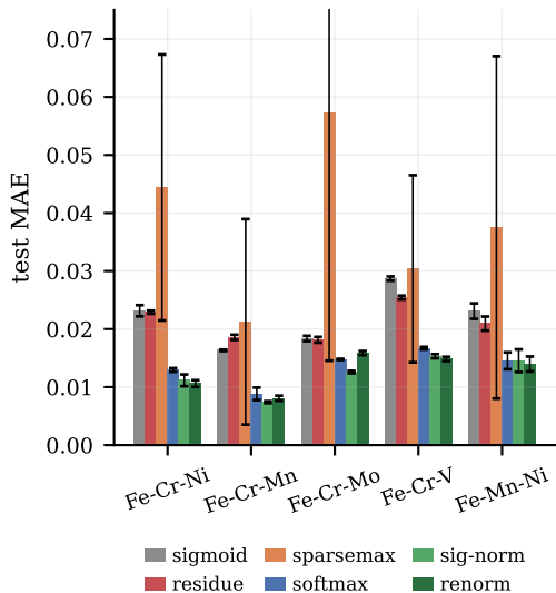
(a) neural heads (mean \pm s.d., 3 seeds)
