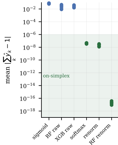
(c) simplex closure
