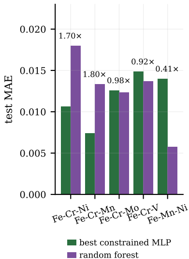
(b) MLP vs trees
