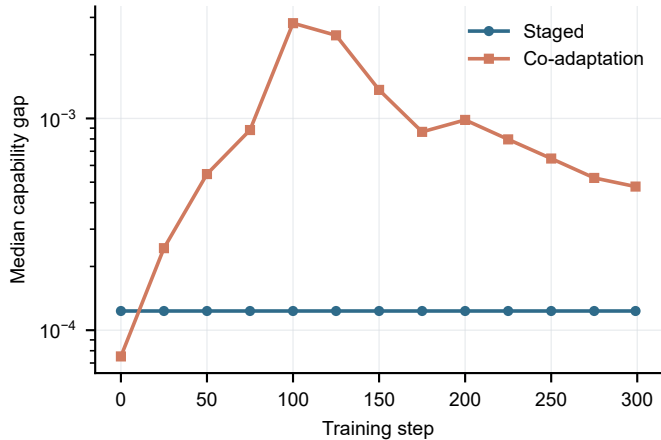
Capability terrain changes under co-adaptation
