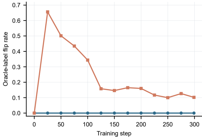
Pointwise best-expert labels keep changing
