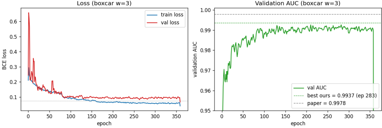
Figure 2: Model 1a 360-epoch training (boxcar-smoothed, window 3, matching the paper’s Fig. 7 convention). Left: train/validation BCE loss. Right: validation AUC; the dashed lines mark our best (0.9937, epoch 283) and the paper’s published peak (0.9978). The 5\times \text{lr} decays at epochs 80/160/240/320 produce the visible step-downs in loss variance.
