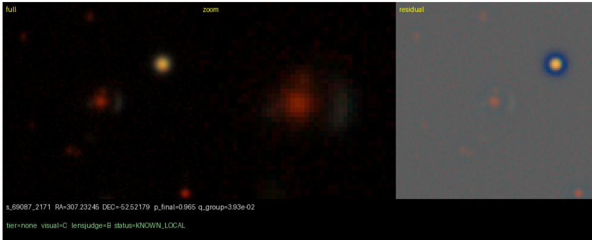
Figure 5: s_69087_2171: RA=307.23245, DEC=-52.52179, p_{\text{final}}=0.965 ; status KNOWN_LOCAL (nearest des_jacobs2019 at 0.09''); visual C, lensjudge B. Full | zoom | residual.
