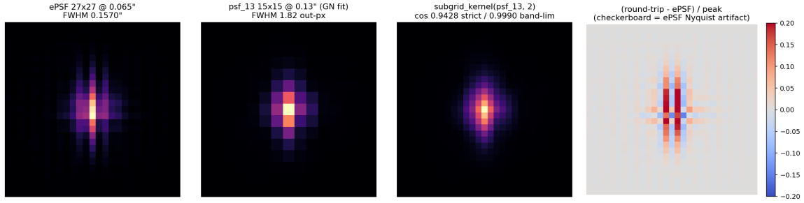
Figure 3: The PSF sampling-convention fix: the 0 '' 065-sampled empirical kernel (left) versus the 0 '' 13-sampled kernel fitted through the simulator’s own subgrid_kernel operator, and the effective PSF each produces in the forward model. The defective configuration broadens the effective PSF by 2\times in r_{50} .
