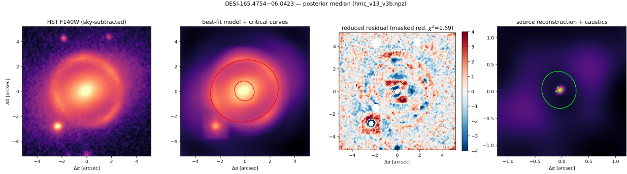
Figure 5: The binned (0.08) product at its low-basin posterior median ( \gamma_{\text{EPL}} = 1.29 ): the inner critical curve persists, but the binned likelihood retains a \Delta\chi^2_\nu = 0.078 preference for a steep-slope mode that does not survive at native scale — the sharpest expression of the open correlated-noise question.
