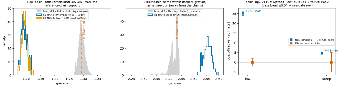
Figure 13: B5 both-basin \lambda = 1 posterior overlay on the 74-d bimodal target foundry_v3b74 , drawn before any gate math per house rule (jobs 56006049 / 56251555 / 56006052). The low basin’s two independent mutation kernels agree on location (MAMS \gamma_{\text{eqw}} = 1.0919 , MCLMC 1.0935); the steep basin sits at 2.5552. Source: data/b5_gate_eval.json .
