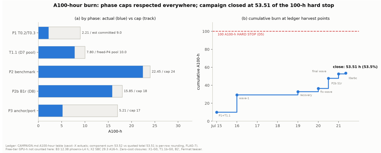
Figure 19: A100-hour burn. (a) Actual vs. cap by phase — every fence respected (P1 2.21, T1.1 7.80 of the D7-freed 10-h pool, P2 22.45/24, P2b 15.85/18, P3 5.21/17). (b) Cumulative burn at the ledger’s harvest points (events in ledger order; sub-day x -offsets are display-only), closing at 53.51 of the 100-h hard stop; the 53.52 component sum is per-row sacct rounding (flagged, not smoothed). Free-tier GPU-h (B3: 12.38 L4-h; X2: 29.3 A16-h) are additional and uncounted here. Zero-cost closures: X1-G0, T1.1b, B2’, the Fermat teaser. Source: CAMPAIGN.md A100-hour ledger (append-before-read protocol).
