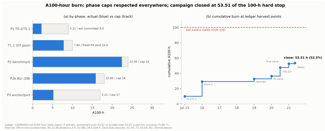
Figure 24: A100-hour burn. (a) Actual vs. cap by phase — every fence respected (P1 2.21, T1.1 7.80 of the D7-freed 10-h pool, P2 22.45/24, P2b 15.85/18, P3 5.21/17). (b) Cumulative burn at the ledger’s harvest points (events in ledger order; sub-day x -offsets are display-only), closing at 53.51 of the 100-h hard stop; the 53.52 component sum is per-row sacct rounding (flagged, not smoothed). Free-tier GPU-h (B3: 12.38 L4-h; X2: 29.3 A16-h) are additional and uncounted here. Zero-cost closures: X1-G0, T1.1b, B2’, the Fermat teaser. Source: CAMPAIGN.md A100-hour ledger (append-before-read protocol).
