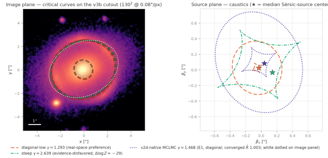
Figure 2: Compact comparison — critical curves (lens plane, over the v3b binned cutout, asinh stretch) and caustics (source plane; stars mark the median Sérsic-source centers) for the surviving posterior-median mass models on shared axes, following the critical-curve/caustic display conventions of the team’s GIGA-LENS discovery paper (Gu et al., 2022): diagonal-low \gamma = 1.293 (the real-space preference), steep \gamma = 2.639 (evidence-disfavored, \Delta \log Z \approx -29 ), and the E1 v2d-native MCLMC fit \gamma = 1.468 (violet on the source panel; neutral white dotted on the image panel). The corr-low \gamma = 1.103 curve was removed from this figure at PI direction — the model is rejected and appears only in the mechanism sections as the diagnosed artifact (§7.4.1, §7.4.3). Scale sanity: the outer critical curve’s median radius matches each model’s \theta_E to < 5\% for all three (diag-low 2.611'' vs. \theta_E = 2.603'' ; MCLMC 2.652'' vs. 2.654'' ), and the \gamma < 2 models show the expected inner radial critical curve and caustic. Deflections from the vendored scene API EPL(50)+shear at the certified conventions; source artifacts data/rfig_modeler_params.npz , data/mclmc_diag_v2d.npz , data/rfig_modeler_checks.json .
