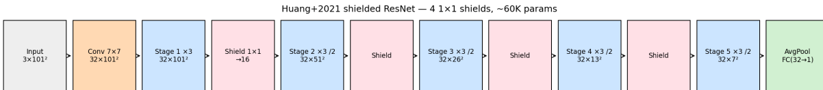
Figure 1: The reconstructed shielded RESNET: stem, then [\text{stage} \times 3 \rightarrow \text{SHIELD}] \times 4 , then a final 3-block stage and the pooled FC( 32 \rightarrow 1 ) head. Four 1\times 1 shields, ~60K parameters.
