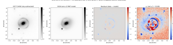
Figure 4: v2 MAP residual (data – model, in units of \sigma_{\text{bg}} ). The bright residual blob \sim 3'' southwest of the main lens is the signature of the nearby galaxy modeled in v3 onward (Figure 3).
