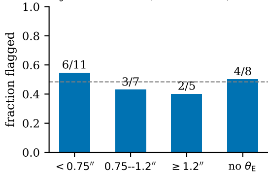
Injected controls (15/31 = 48%)
