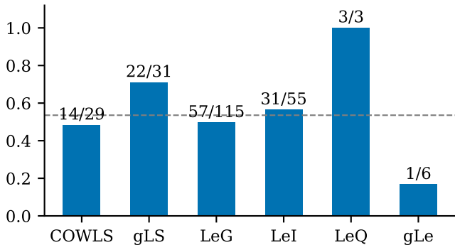
Catalogued lenses on cutouts (128/239 = 54%)
