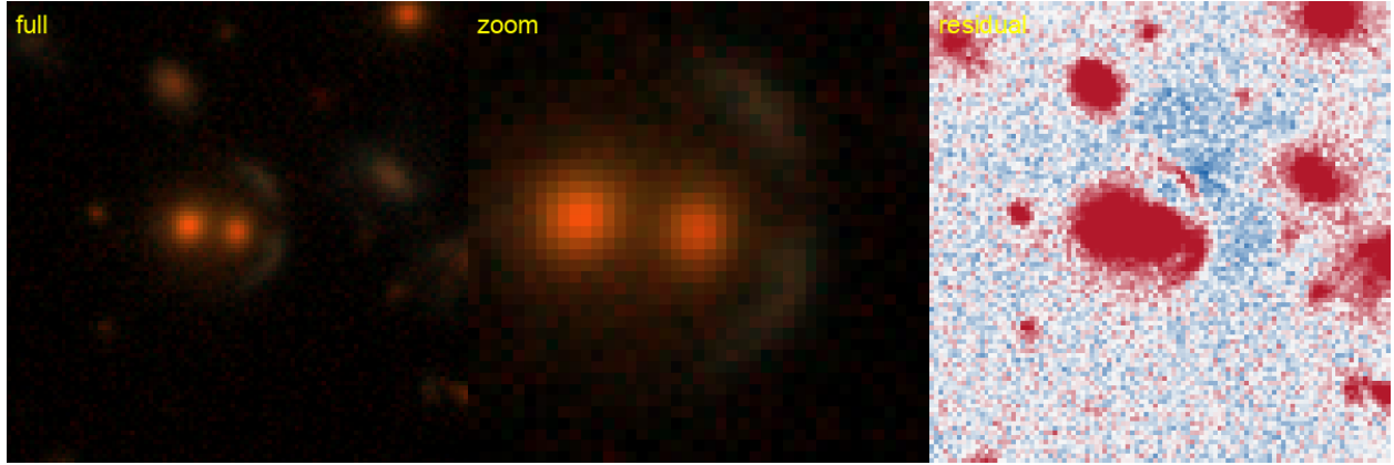
Figure 77: #52 s_266620_918 — RA 172.1320, Dec -11.3108; grade B , tier-1 p_{\text{lens}} 0.42, v3blend8 0.80. NEW — new to the DESI lens-finders, the DES/AGEL/CASSOWARY searches, and the NED/SIMBAD literature.
