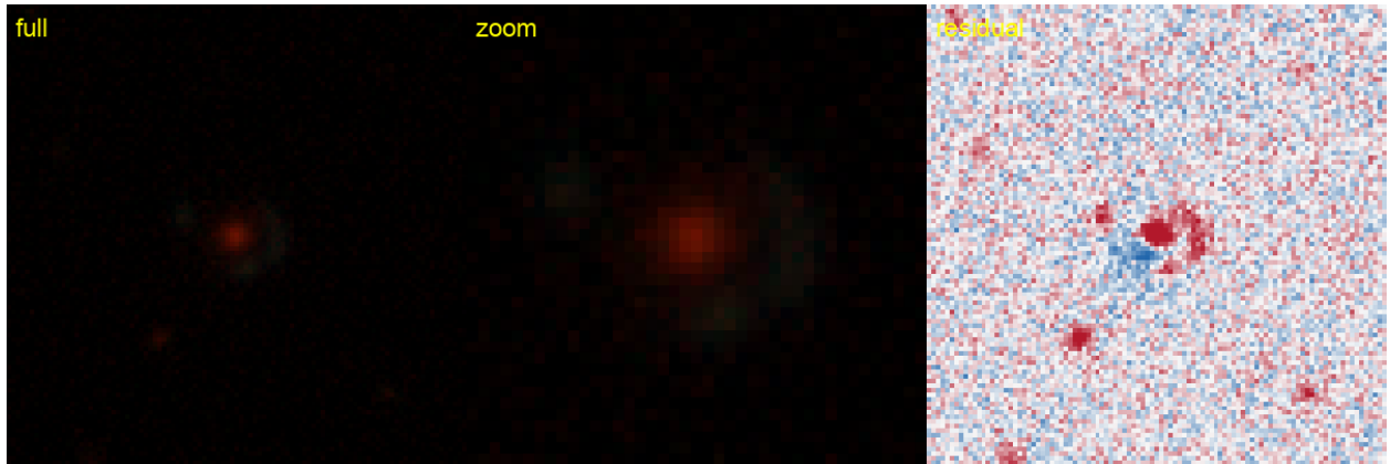
Figure 18: #10 s_180593_5604 — RA 44.0974, Dec -27.1218; grade B , tier-1 p_{\text{lens}} 0.63, v3blend8 0.88. KNOWN — DES: DES J025623.36-270718.5, 0.28'' (SIMBAD).
