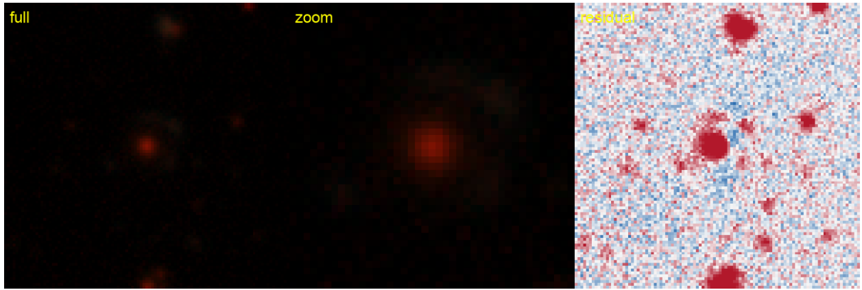
Figure 27: #23 s_50907_11900 — RA 303.5808, Dec -57.9504; grade B , tier-1 p_{\text{lens}} 0.58, v3blend8 0.74. KNOWN — DES: DES J201419.38-575701.4, 0.15'' (SIMBAD).
