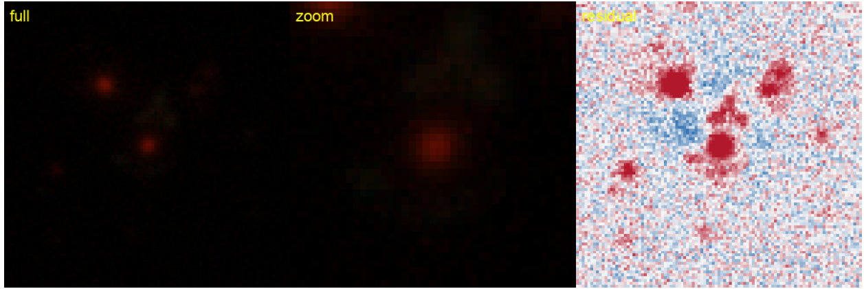
Figure 60: #75 s.94933_7964 — RA 47.5548, Dec -45.5743; grade B , tier-1 p_{\text{lens}} 0.35, v3blend8 0.78. KNOWN — DES: [DBL2017] DES J0310-4534 (A), 0.14'' (SIMBAD).
