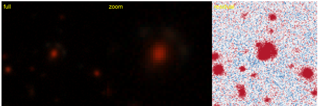
Figure 28: #24 s_34114_11363 — RA 353.7468, Dec -64.0687; grade B , tier-1 p_{\text{lens}} 0.55, v3blend8 0.90. KNOWN — DES: DES J233459.19-640406.9, 0.32'' (SIMBAD).
