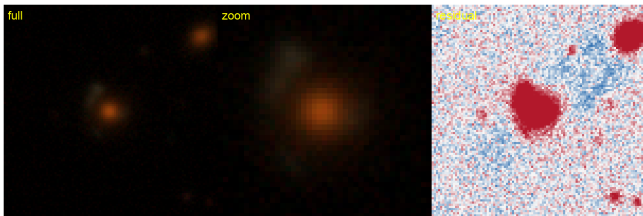
Figure 87: #76 s_250997_4626 — RA 133.2708, Dec -13.8944; grade B , tier-1 p_{\text{lens}} 0.35, v3blend8 0.77. NEW — new to the DESI lens-finders, the DES/AGEL/CASSOWARY searches, and the NED/SIMBAD literature.
