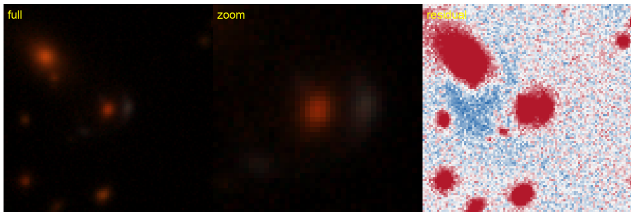
Figure 62: #78 s_90920_9419 — RA 45.9517, Dec -46.4407; grade B , tier-1 p_{\text{lens}} 0.30, v3blend8 0.85. KNOWN — DES: [DBL2017] DES J0303-4626 (A), 0.15'' (SIMBAD).
