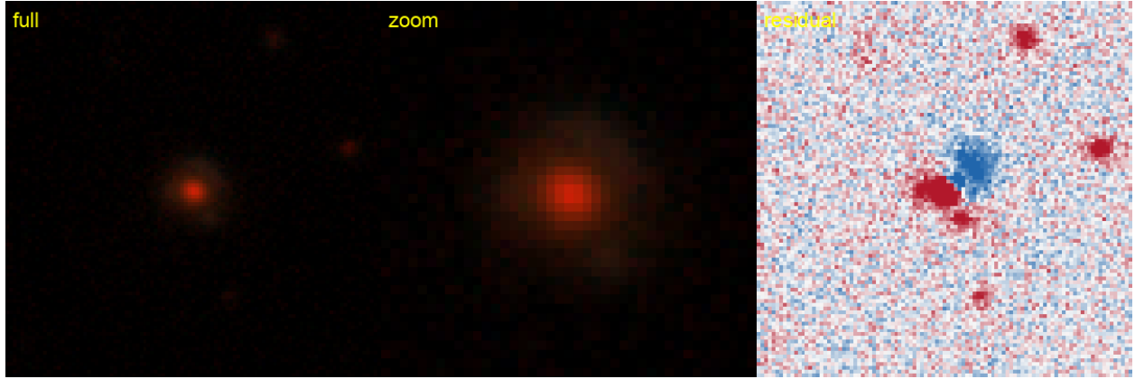
Figure 65: #15 s_205319_6061 — RA 359.9772, Dec -22.4596; grade B , tier-1 p_{\text{lens}} 0.60, v3blend8 0.88. NEW — new to the DESI lens-finders, the DES/AGEL/CASSOWARY searches, and the NED/SIMBAD literature.
