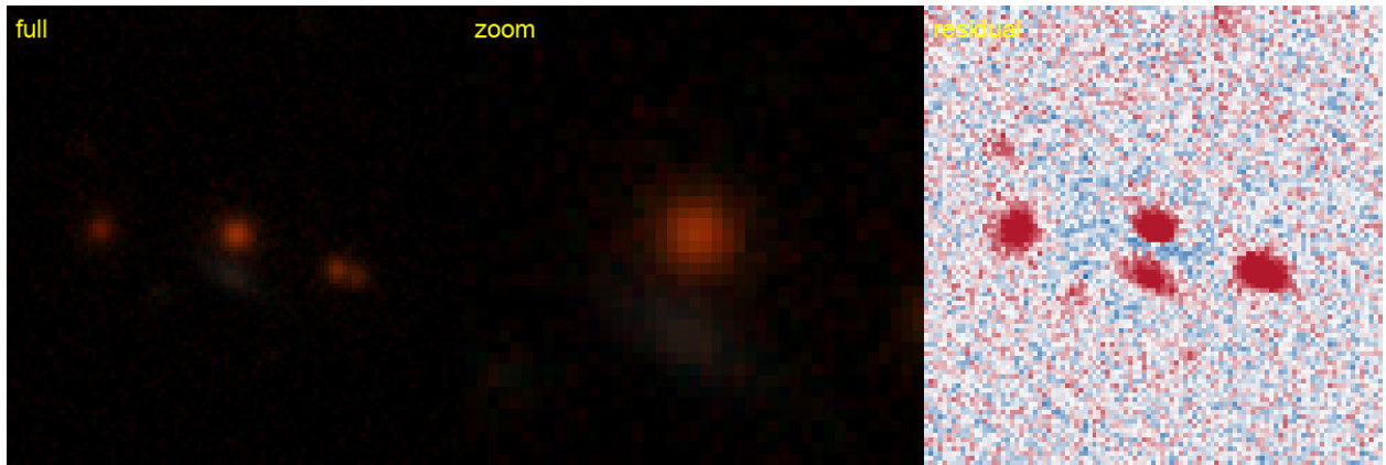
Figure 70: #35 s.289350.3716 — RA 164.8051, Dec -7.1449; grade B , tier-1 p_{\text{lens}} 0.50, v3blend8 0.81. NEW — new to the DESI lens-finders, the DES/AGEL/CASSOWARY searches, and the NED/SIMBAD literature.
