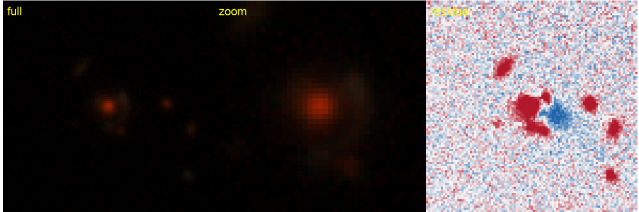
Figure 56: #68 s.209576.5226 — RA 65.5760, Dec -21.5461; grade B , tier-1 p_{\text{lens}} 0.38, v3blend8 0.86. KNOWN — DES: DES J042218.21-213245.8, 0.28'' (SIMBAD).
