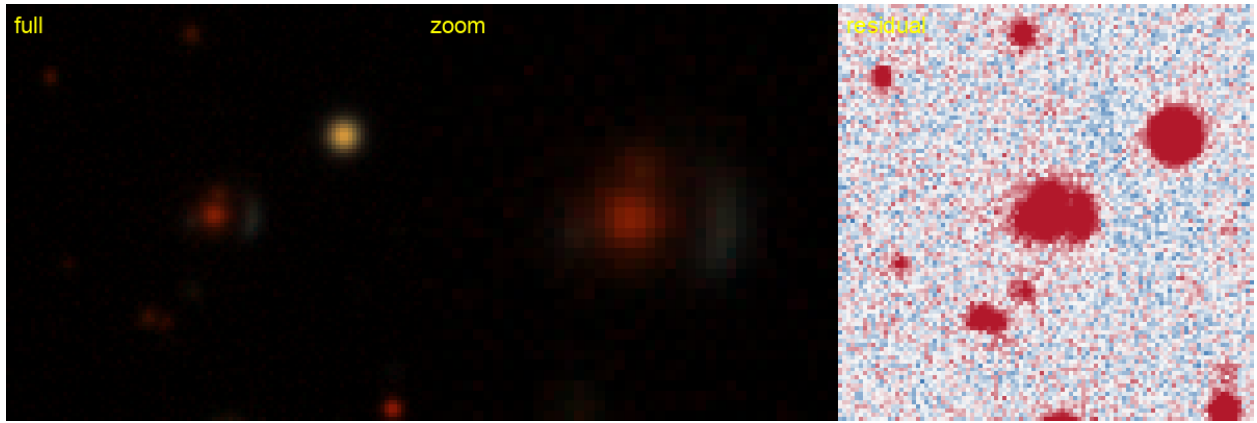
Figure 51: #60 s_69087.268 — RA 307.2325, Dec -52.5218; grade B , tier-1 p_{\text{lens}} 0.40, v3blend8 0.81. KNOWN — DES: DES J202855.79-523118.3, 0.12'' (SIMBAD).
