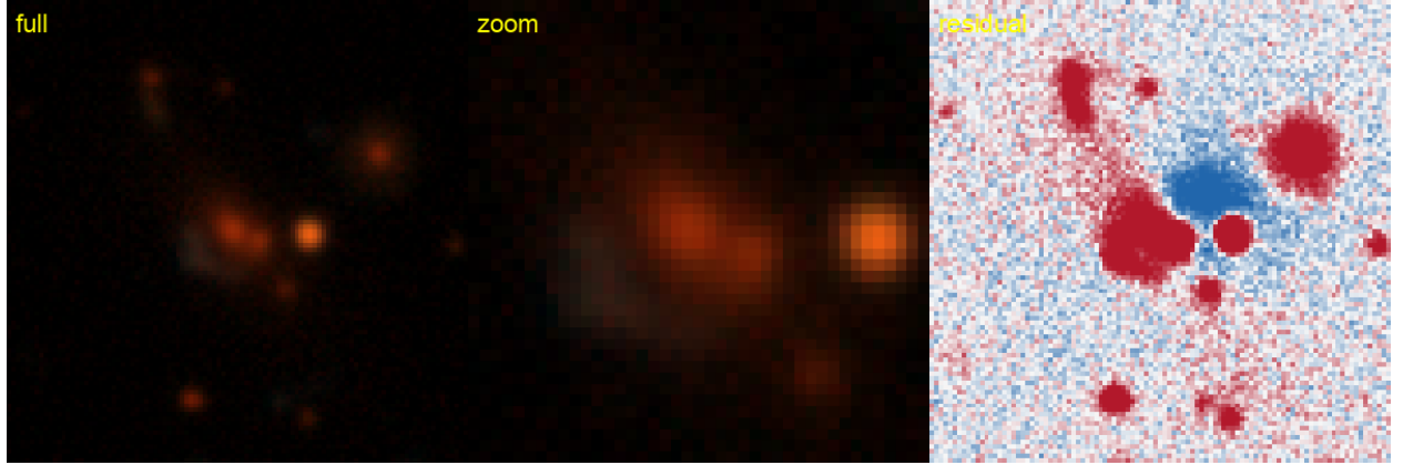
Figure 21: #14 s_42996.3467 — RA 53.7444, Dec -60.5805; grade B , tier-1 p_{\text{lens}} 0.60, v3blend8 0.90. KNOWN — DES: DES J033458.64-603450.0, 0.15'' (SIMBAD).
