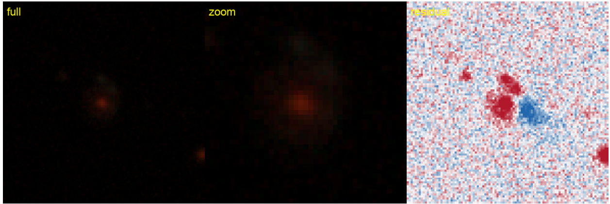
Figure 84: #70 s_250611_2161 — RA 33.7898, Dec -14.1185; grade B , tier-1 p_{\text{lens}} 0.38, v3blend8 0.77. NEW — new to the DESI lens-finders, the DES/AGEL/CASSOWARY searches, and the NED/SIMBAD literature.
