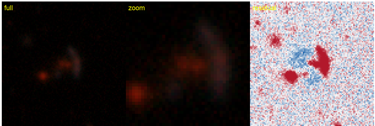
Figure 73: #43 s_502450_1680 — RA 161.1145, Dec +31.2344; grade B , tier-1 p_{\text{lens}} 0.45, v3blend8 0.79. NEW — new to the DESI lens-finders, the DES/AGEL/CASSOWARY searches, and the NED/SIMBAD literature.
