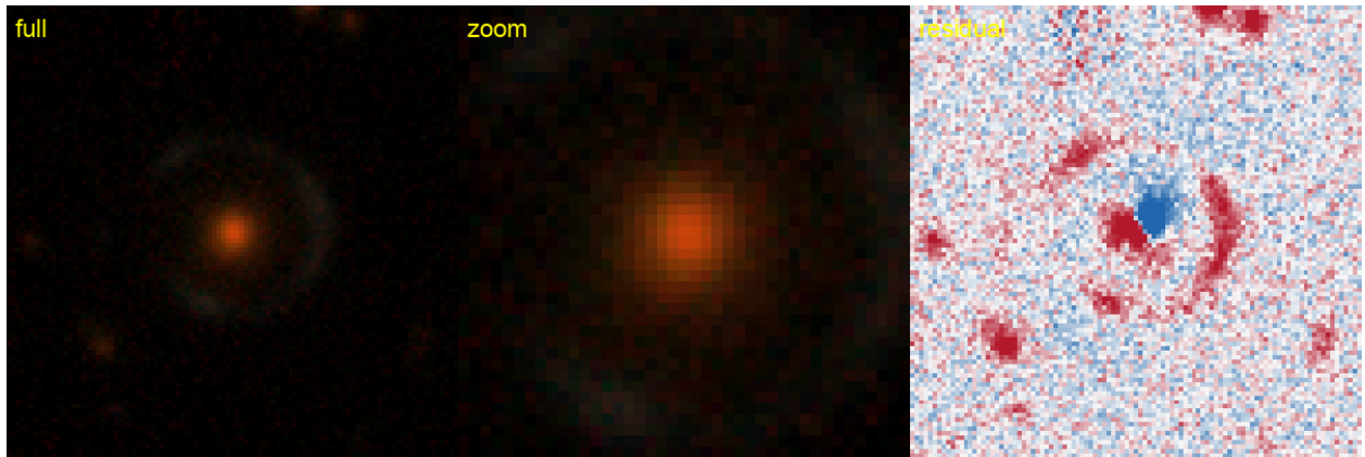
Figure 13: #4 s_441355.1188 — RA 177.1381, Dec +19.5009; grade A , tier-1 p_{\text{lens}} 0.87, v3blend8 0.83. KNOWN — CASSOWARY: CSWA 1, 0.01'' (lineage).
