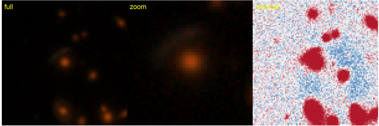
Figure 41: #42 s_82090.1248 — RA 14.4037, Dec -48.8040; grade B , tier-1 p_{\text{lens}} 0.45, v3blend8 0.81. KNOWN — DES: [DBL2017] DES J0057-4848 (A), 0.19'' (SIMBAD).
