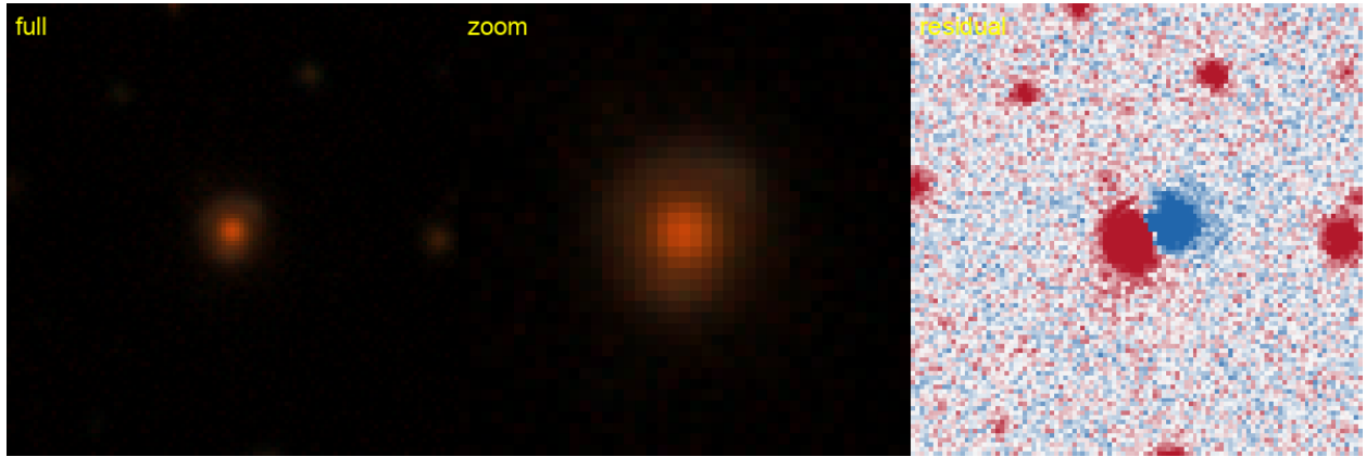
Figure 66: #18 s_218895_5088 — RA 32.7525, Dec -19.6362; grade B , tier-1 p_{\text{lens}} 0.60, v3blend8 0.81. NEW — new to the DESI lens-finders, the DES/AGEL/CASSOWARY searches, and the NED/SIMBAD literature.
