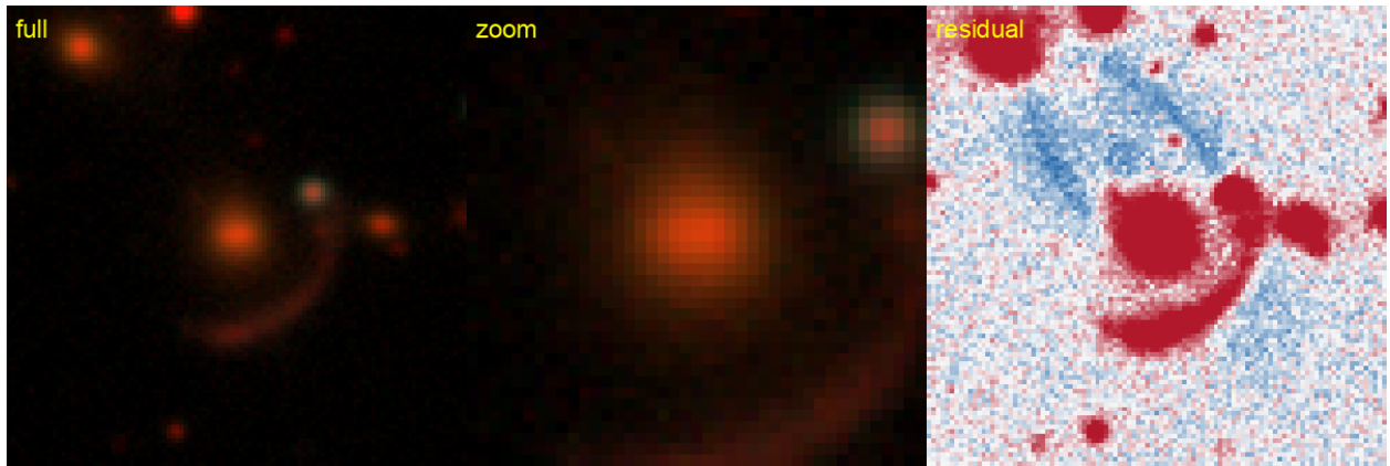
Figure 67: #22 s_194300_2796 — RA 242.6052, Dec -24.4155; grade B , tier-1 p_{\text{lens}} 0.58, v3blend8 0.74. NEW — new to the DESI lens-finders, the DES/AGEL/CASSOWARY searches, and the NED/SIMBAD literature.
