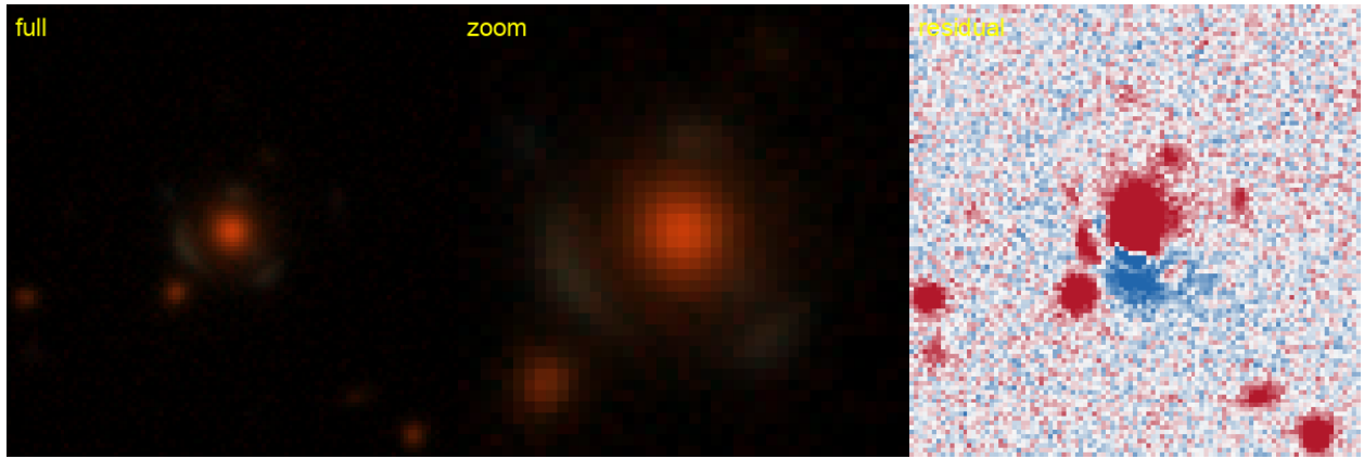
Figure 15: #6 s_124958_7349 — RA 58.1768, Dec -38.4292; grade A , tier-1 p_{\text{lens}} 0.81, v3blend8 0.89. KNOWN — DES: DES J035242.40-382544.9, 0.01'' (lineage).
