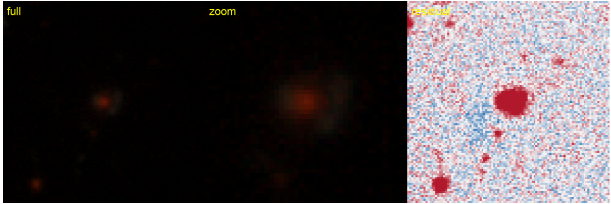
Figure 36: #34 s_257579.1725 — RA 23.3422, Dec -12.8670; grade B , tier-1 p_{\text{lens}} 0.50, v3blend8 0.82. KNOWN — DES: DES J013322.10-125201.2, 0.27'' (SIMBAD).
