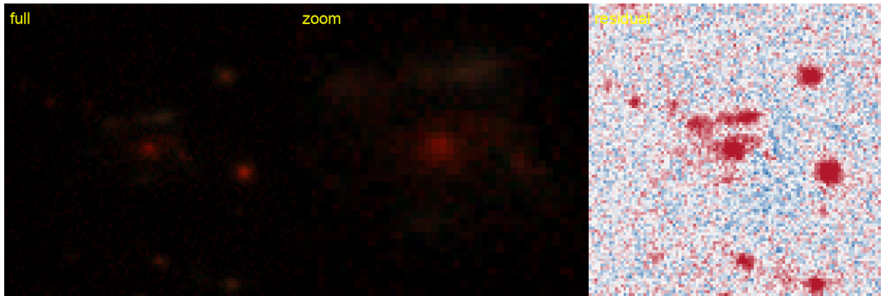
Figure 79: #56 s_262449_2840 — RA 188.7861, Dec -11.9798; grade B , tier-1 p_{\text{lens}} 0.40, v3blend8 0.87. NEW — new to the DESI lens-finders, the DES/AGEL/CASSOWARY searches, and the NED/SIMBAD literature.
