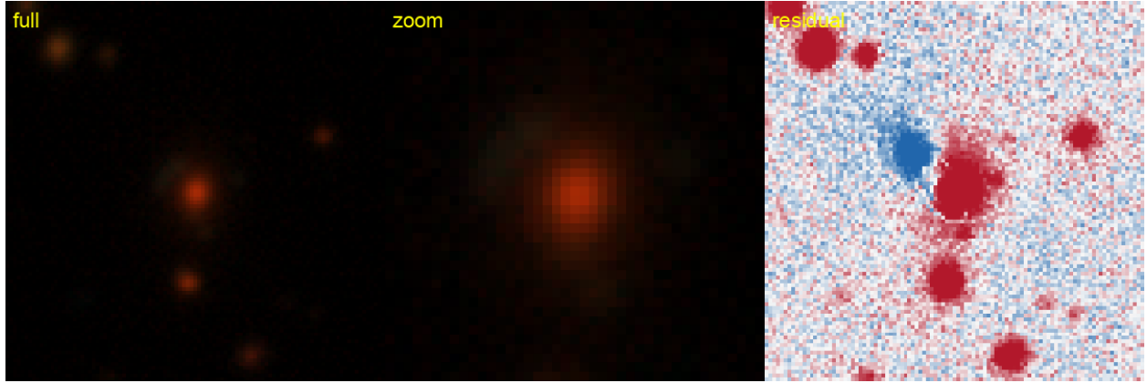
Figure 59: #74 s.238185_2253 — RA 58.5761, Dec -16.1645; grade B , tier-1 p_{\text{lens}} 0.35, v3blend8 0.82. KNOWN — AGEL: AGEL J035418-160952 system, 0.51'' (SIMBAD).
