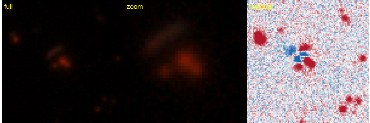
Figure 23: #17 s_38835_314 — RA 56.6543, Dec -61.9792; grade B , tier-1 p_{\text{lens}} 0.60, v3blend8 0.84. KNOWN — DES: [DBL2017] DES J0346-6158 (A), 0.23'' (SIMBAD).
