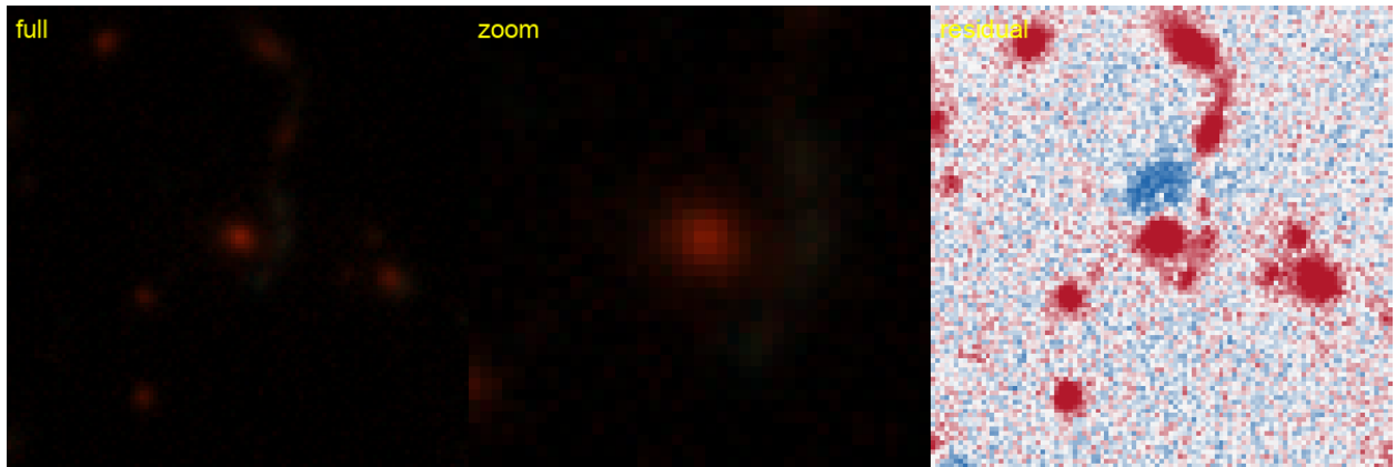
Figure 40: #40 s_280236.3353 — RA 25.8623, Dec -8.8393; grade B , tier-1 p_{\text{lens}} 0.45, v3blend8 0.84. KNOWN — AGEL: AGEL J014327-085021 system, 0.93'' (SIMBAD).
