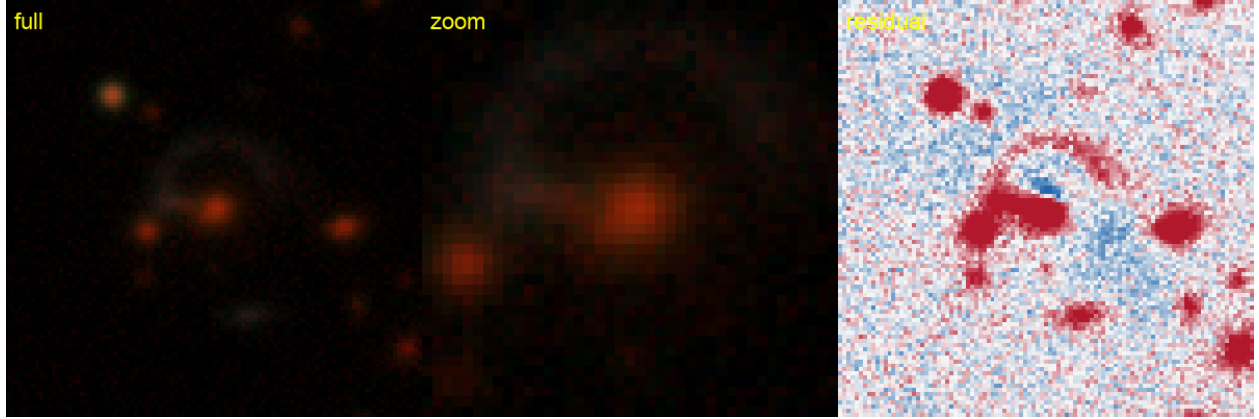
Figure 63: #9 s_230539_4159 — RA 222.0715, Dec -17.8489; grade B , tier-1 p_{\text{lens}} 0.72, v3blend8 0.84. NEW — new to the DESI lens-finders, the DES/AGEL/CASSOWARY searches, and the NED/SIMBAD literature.
