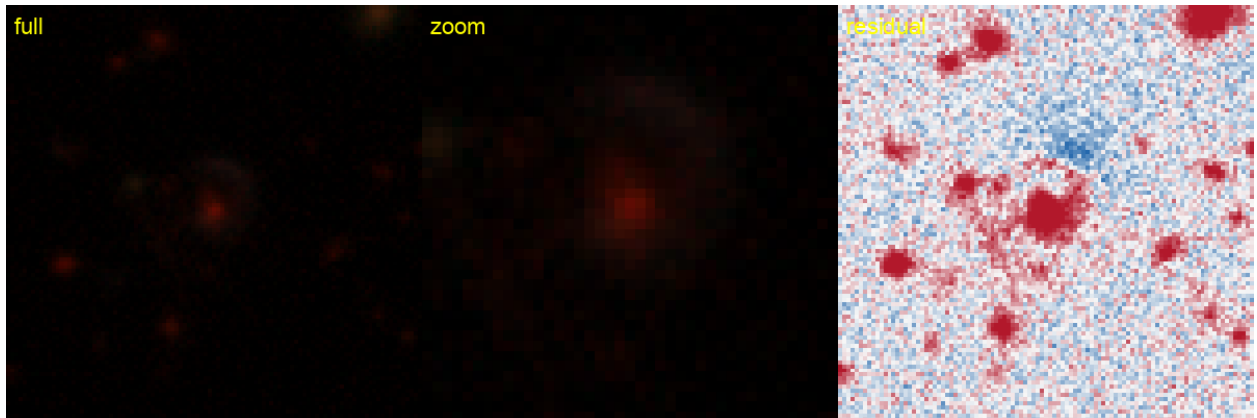
Figure 55: #66 s_119342_4136 — RA 50.7164, Dec -39.7694; grade B , tier-1 p_{\text{lens}} 0.38, v3blend8 0.90. KNOWN — DES: DES J032251.91-394609.6, 0.17'' (SIMBAD).
