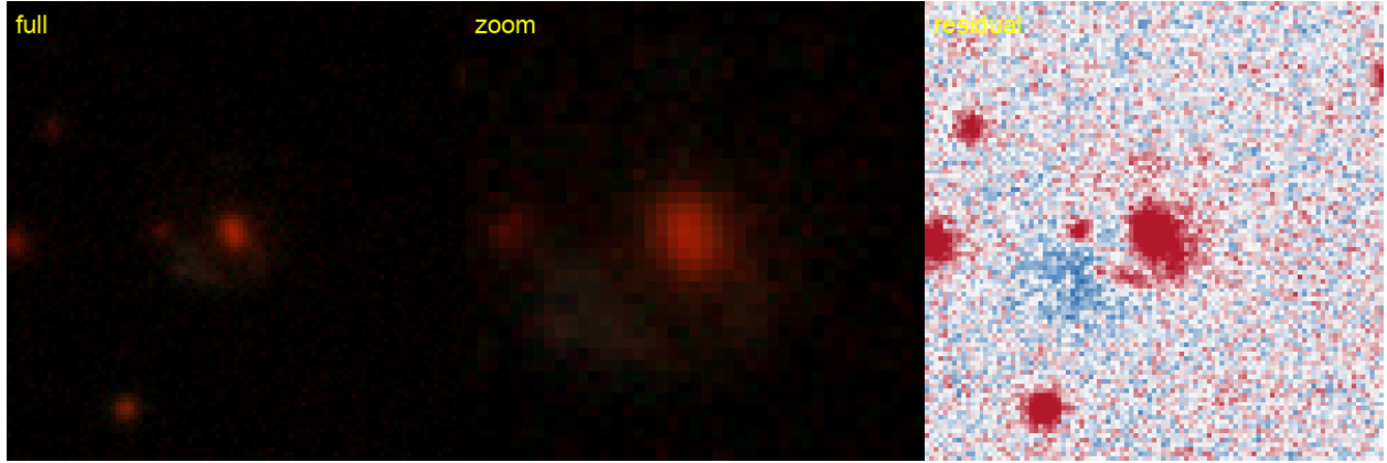
Figure 83: #67 s_405220_1292 — RA 136.4655, Dec +13.0307; grade B , tier-1 p_{\text{lens}} 0.38, v3blend8 0.89. NEW — new to the DESI lens-finders, the DES/AGEL/CASSOWARY searches, and the NED/SIMBAD literature.
