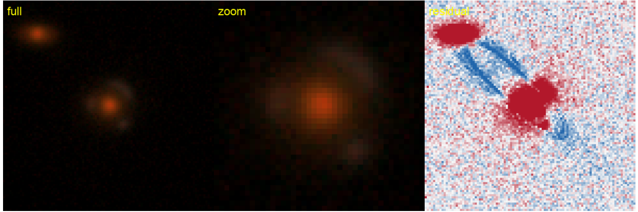
Figure 64: #13 s_234689_542 — RA 227.0427, Dec -16.8771; grade B , tier-1 p_{\text{lens}} 0.62, v3blend8 0.80. NEW — new to the DESI lens-finders, the DES/AGEL/CASSOWARY searches, and the NED/SIMBAD literature.
