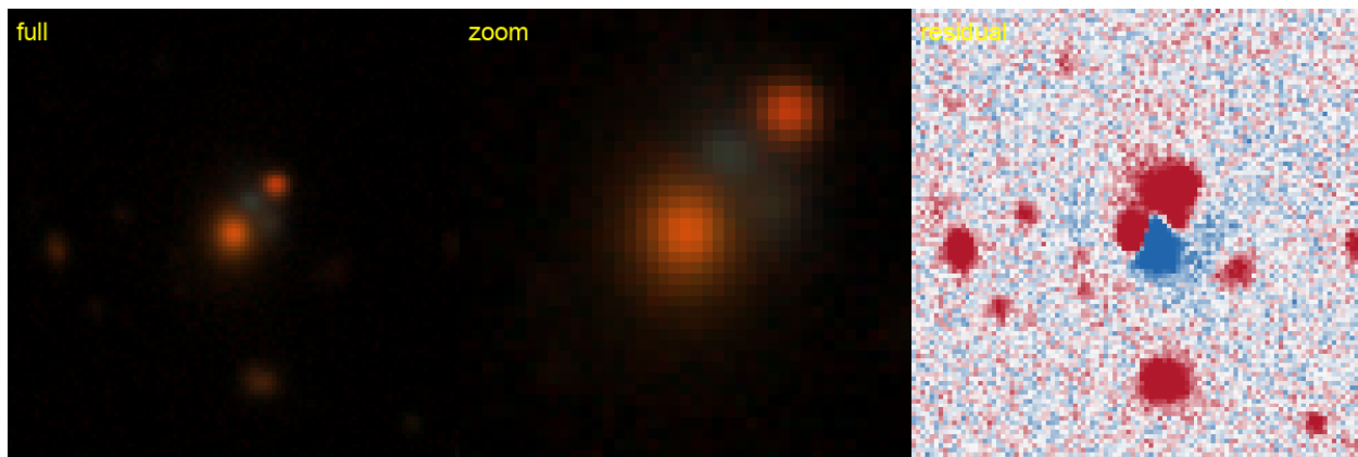
Figure 86: #72 s_210799_616 — RA 33.4979, Dec -21.2827; grade B , tier-1 p_{\text{lens}} 0.38, v3blend8 0.75. NEW — new to the DESI lens-finders, the DES/AGEL/CASSOWARY searches, and the NED/SIMBAD literature.
