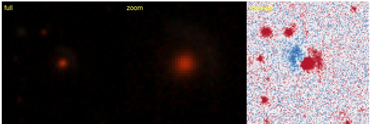
Figure 16: #7 s_191004_9637 — RA 56.9356, Dec -24.9088; grade A , tier-1 p_{\text{lens}} 0.80, v3blend8 0.88. KNOWN — DES: DES J034744.53-245431.4, 0.20'' (SIMBAD).
