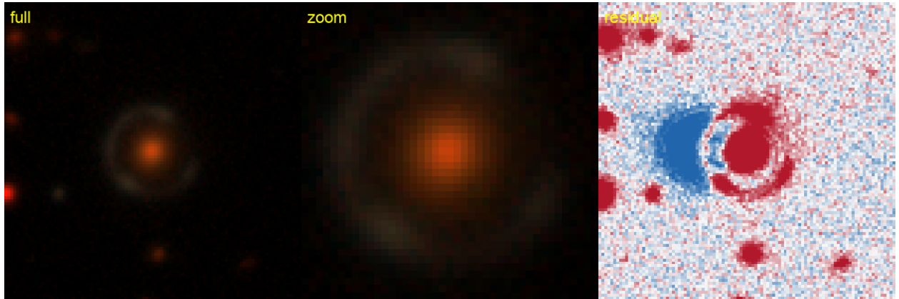
Figure 10: #1 s_310364_6388 — RA 38.2078, Dec -3.3906; grade A , tier-1 p_{\text{lens}} 0.90, v3blend8 0.82. KNOWN — Huang+2020: DESI-038.2078-03.3906, 0.16'' (lineage).
