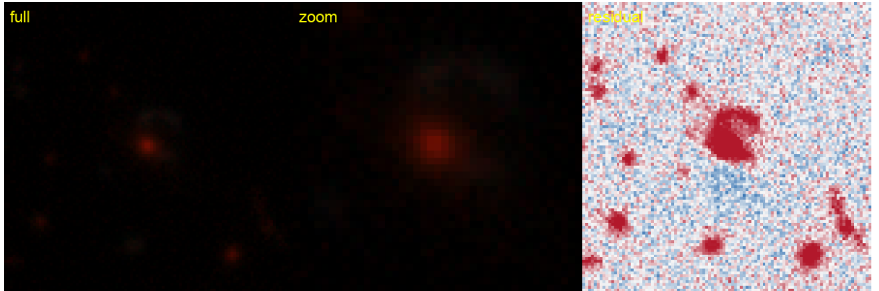
Figure 22: #16 s_188493.9685 — RA 83.4556, Dec -25.6151; grade B , tier-1 p_{\text{lens}} 0.60, v3blend8 0.88. KNOWN — DES: DES J053349.32-253654.3, 0.15'' (SIMBAD).
