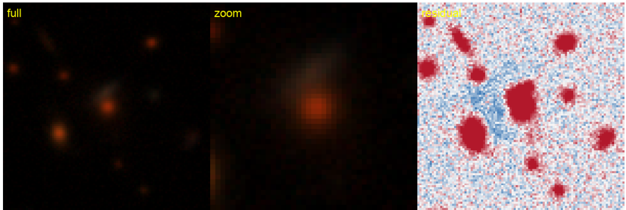
Figure 85: #71 s_161725_5181 — RA 61.4085, Dec -30.6887; grade B , tier-1 p_{\text{lens}} 0.38, v3blend8 0.76. NEW — new to the DESI lens-finders, the DES/AGEL/CASSOWARY searches, and the NED/SIMBAD literature.
