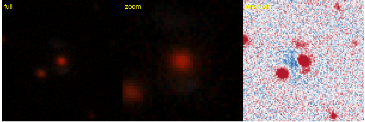
Figure 47: #54 s_381188_1199 — RA 144.1511, Dec +8.8633; grade B , tier-1 p_{\text{lens}} 0.40, v3blend8 0.90. KNOWN — Huang+2020: DESI-144.1511+08.8633, 0.20'' (lineage).
