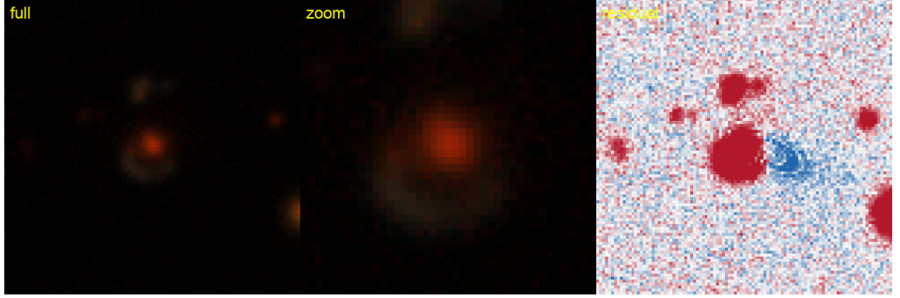
Figure 20: #12 s_232538.8716 — RA 25.2755, Dec -17.2232; grade B , tier-1 p_{\text{lens}} 0.62, v3blend8 0.85. KNOWN — Huang+2020: DESI-025.2755-17.2232, 0.19'' (lineage).
