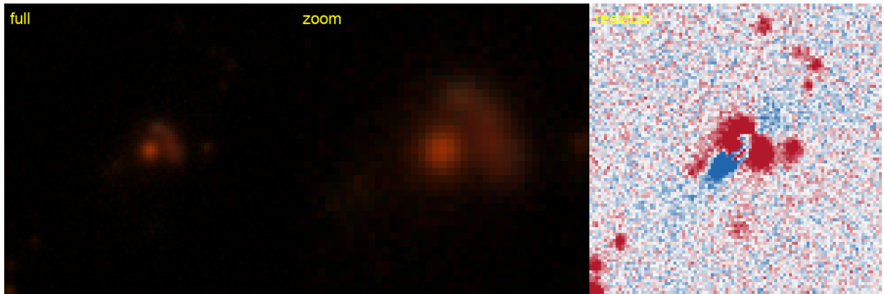
Figure 58: #73 s.129372.3768 — RA 16.4504, Dec -37.4286; grade B , tier-1 p_{\text{lens}} 0.35, v3blend8 0.82. KNOWN — DES: DES J010548.04-372542.4, 0.71'' (SIMBAD).
