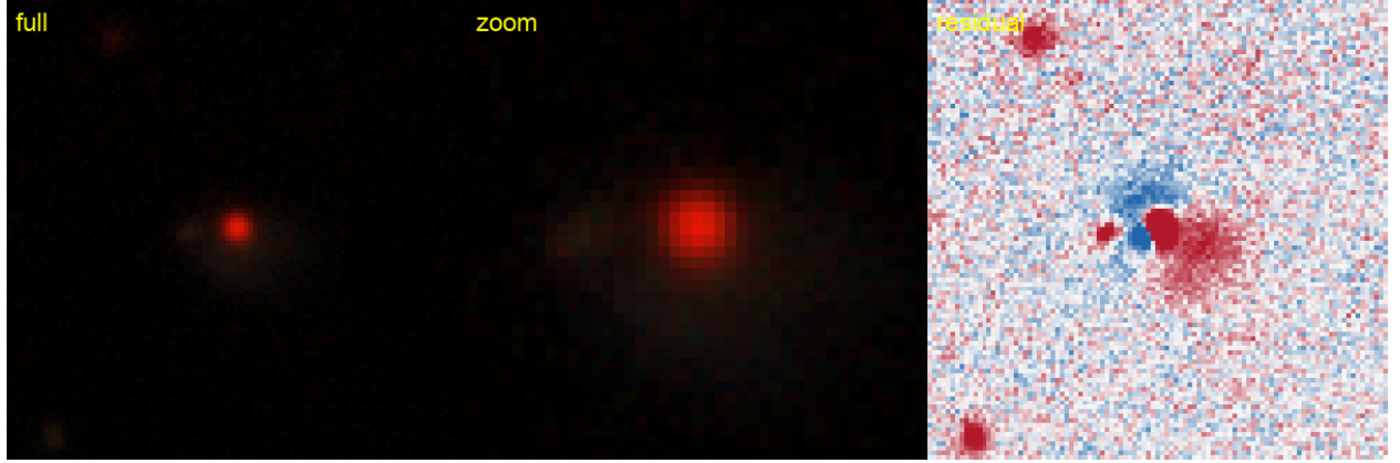
Figure 75: #45 s_369309_653 — RA 30.4465, Dec +6.6551; grade B , tier-1 p_{\text{lens}} 0.45, v3blend8 0.74. NEW — new to the DESI lens-finders, the DES/AGEL/CASSOWARY searches, and the NED/SIMBAD literature.
