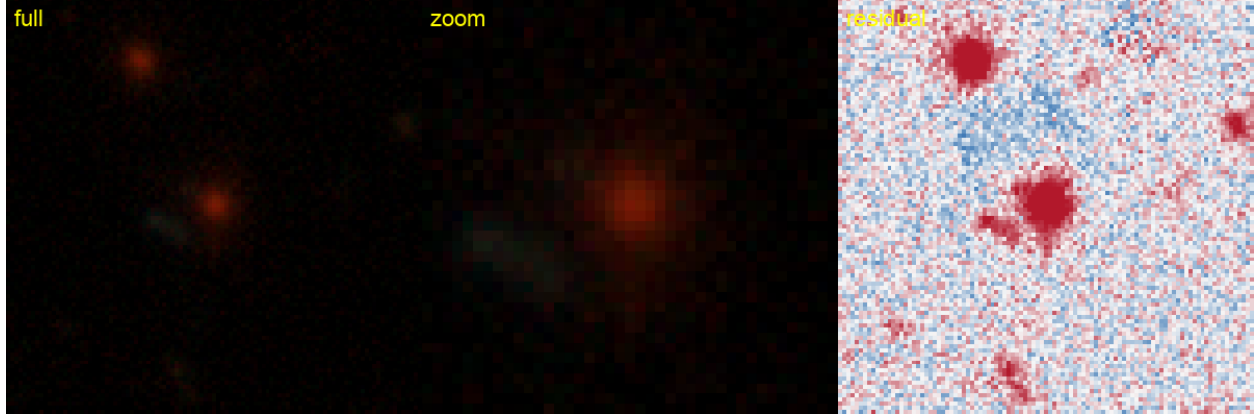
Figure 80: #58 s_360639_3636 — RA 13.4868, Dec +5.3590; grade B , tier-1 p_{\text{lens}} 0.40, v3blend8 0.85. NEW — new to the DESI lens-finders, the DES/AGEL/CASSOWARY searches, and the NED/SIMBAD literature.
