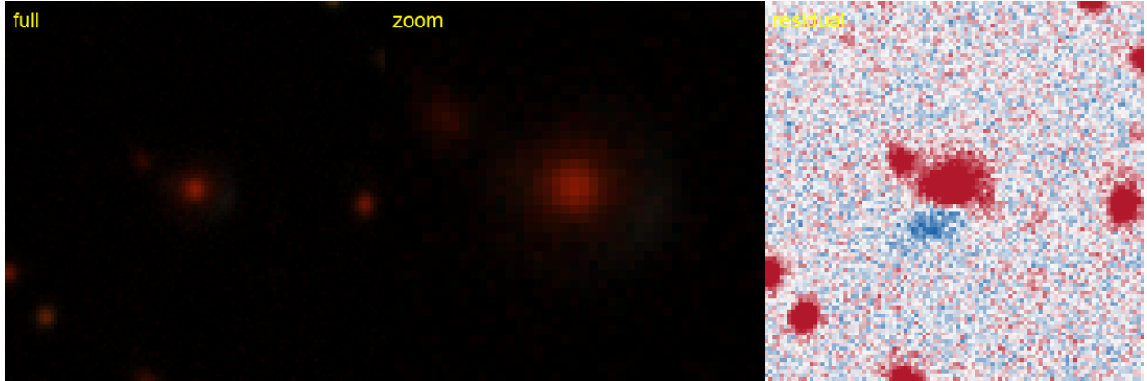
Figure 38: #38 s_58263.3751 — RA 42.7179, Dec -55.4032; grade B , tier-1 p_{\text{lens}} 0.45, v3blend8 0.88. KNOWN — DES: DES J025052.27-552411.7, 0.22'' (SIMBAD).
