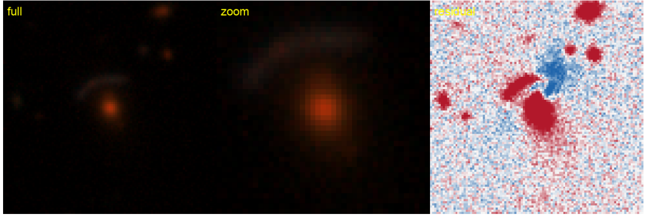
Figure 11: #2 s_137502.1047 — RA 26.4450, Dec -35.6910; grade A , tier-1 p_{\text{lens}} 0.90, v3blend8 0.80. KNOWN — DES: DES J014546.78-354127.3, 0.20'' (SIMBAD).
