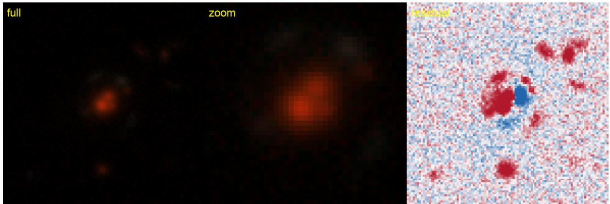
Figure 31: #27 s_197474_9756 — RA 30.7668, Dec -23.6341; grade B , tier-1 p_{\text{lens}} 0.55, v3blend8 0.81. KNOWN — DES: DES J020304.01-233802.5, 0.22'' (SIMBAD).
