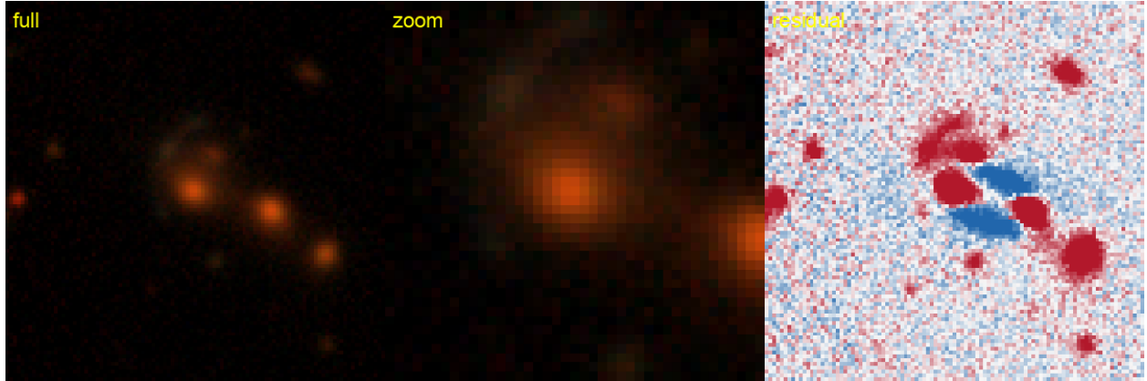
Figure 71: #36 s_148704_6732 — RA 183.8176, Dec -33.6006; grade B , tier-1 p_{\text{lens}} 0.50, v3blend8 0.80. NEW — new to the DESI lens-finders, the DES/AGEL/CASSOWARY searches, and the NED/SIMBAD literature.
