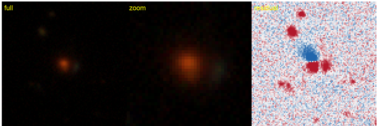
Figure 82: #65 s_188754_2468 — RA 155.4695, Dec -25.5029; grade B , tier-1 p_{\text{lens}} 0.40, v3blend8 0.74. NEW — new to the DESI lens-finders, the DES/AGEL/CASSOWARY searches, and the NED/SIMBAD literature.
