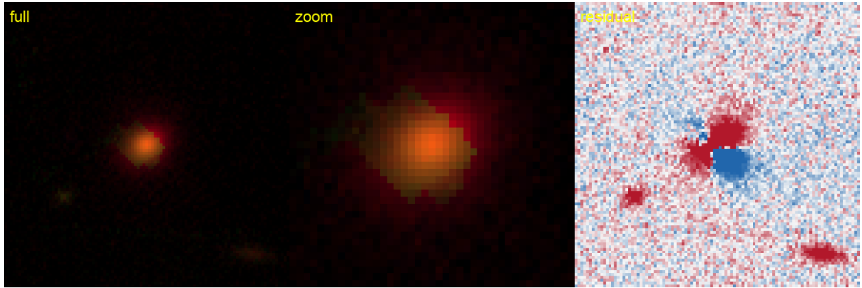
Figure 69: #32 s.353585.141 — RA 45.8222, Dec +3.9613; grade B , tier-1 p_{\text{lens}} 0.50, v3blend8 0.84. NEW — new to the DESI lens-finders, the DES/AGEL/CASSOWARY searches, and the NED/SIMBAD literature.
