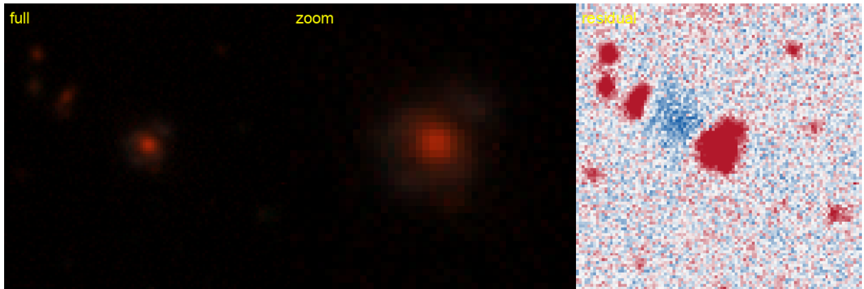
Figure 43: #48 s_94861.9433 — RA 21.9716, Dec -45.5428; grade B , tier-1 p_{\text{lens}} 0.42, v3blend8 0.87. KNOWN — DES: DES J012753.17-453233.8, 0.17'' (SIMBAD).
