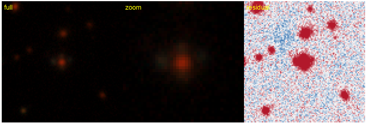
Figure 48: #55 s_235296_3732 — RA 25.6457, Dec -16.8049; grade B , tier-1 p_{\text{lens}} 0.40, v3blend8 0.88. KNOWN — AGEL: AGEL J014235-164818 system, 0.86'' (SIMBAD).
