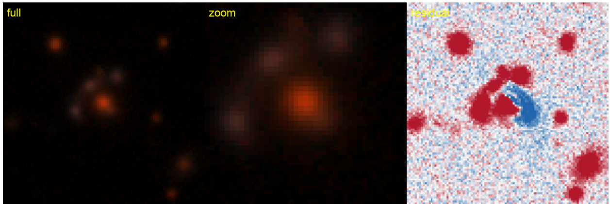
Figure 46: #51 s_71042_1653 — RA 20.1760, Dec -51.7314; grade B , tier-1 p_{\text{lens}} 0.42, v3blend8 0.82. KNOWN — DES: [DBL2017] DES J0120-5143 (A), 0.19'' (SIMBAD).
