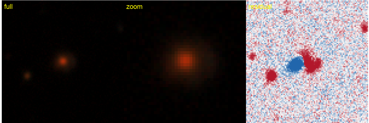
Figure 32: #29 s_310225_1602 — RA 3.2923, Dec -3.5960; grade B , tier-1 p_{\text{lens}} 0.52, v3blend8 0.75. KNOWN — DES: DES J001310.13-033545.4, 0.18'' (SIMBAD).
