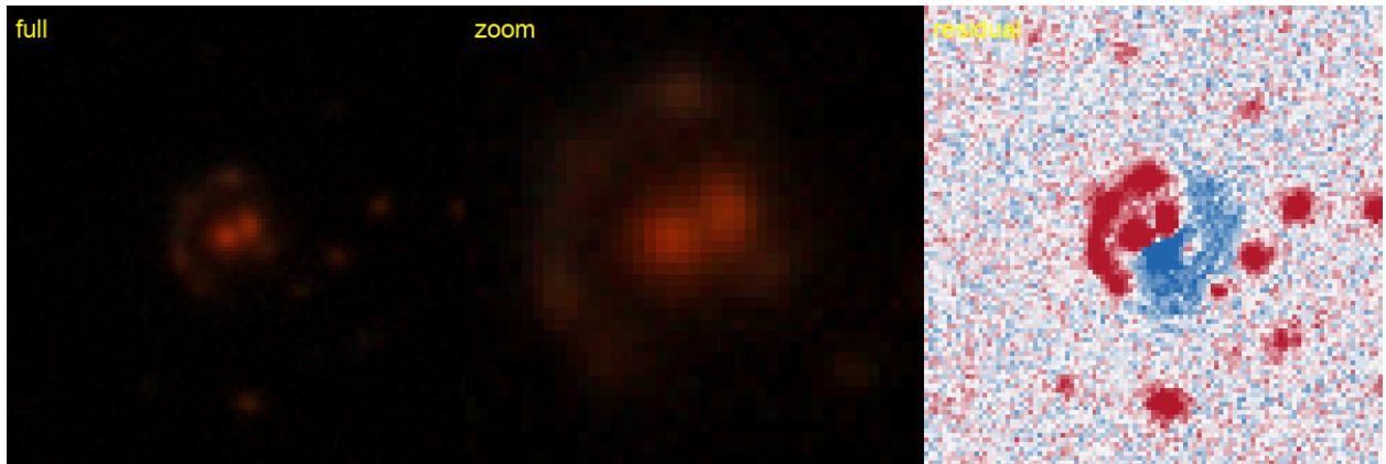
Figure 49: #57 s_91761_4679 — RA 350.3683, Dec -46.5138; grade B , tier-1 p_{\text{lens}} 0.40, v3blend8 0.86. KNOWN — DES: DES J232128.37-463049.3, 0.25'' (SIMBAD).
