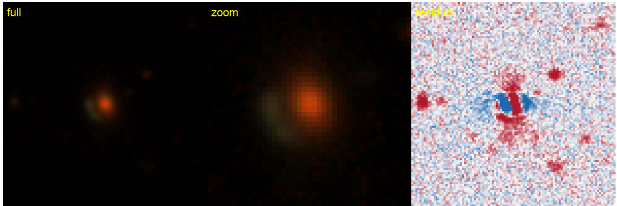
Figure 24: #19 s_240846_8850 — RA 30.2832, Dec -15.8547; grade B , tier-1 p_{\text{lens}} 0.60, v3blend8 0.80. KNOWN — Huang+2020: DESI-030.2832-15.8547, 0.15'' (lineage).
