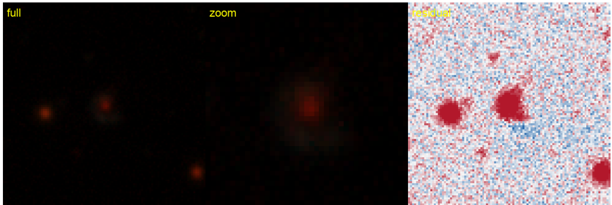
Figure 52: #61 s_165468.9648 — RA 64.7771, Dec -29.9937; grade B , tier-1 p_{\text{lens}} 0.40, v3blend8 0.78. KNOWN — DES: DES J041906.50-295937.7, 0.49'' (SIMBAD).
