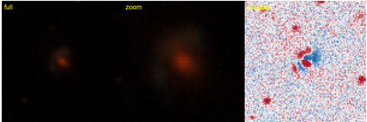
Figure 37: #37 s_301694.7426 — RA 26.2679, Dec -4.9310; grade B , tier-1 p_{\text{lens}} 0.48, v3blend8 0.85. KNOWN — Huang+2020: DESI-026.2679-04.9310, 0.13'' (lineage).
