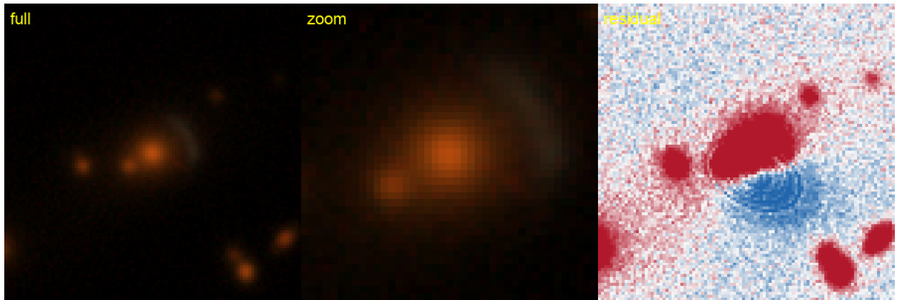
Figure 34: #31 s_137518_1133 — RA 31.3588, Dec -35.6632; grade B , tier-1 p_{\text{lens}} 0.50, v3blend8 0.84. KNOWN — DES: DES J020526.09-353947.4, 0.14'' (SIMBAD).
