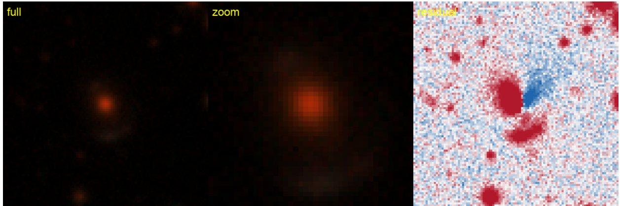
Figure 61: #77 s.71871_246 — RA 353.9664, Dec -51.8716; grade B , tier-1 p_{\text{lens}} 0.35, v3blend8 0.76. KNOWN — AGEL: AGEL J233552-515218 system, 0.95'' (SIMBAD).
