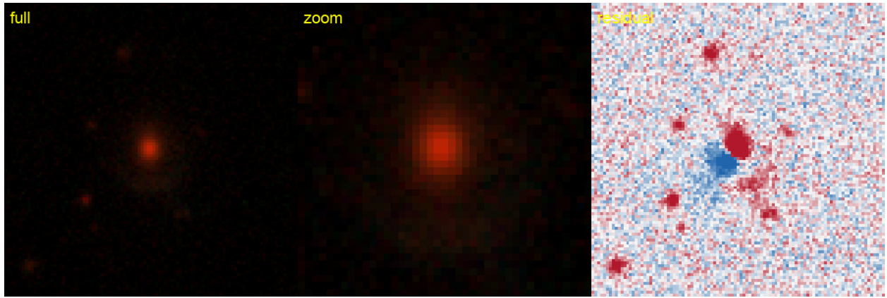
Figure 54: #63 s_364017_5199 — RA 141.0626, Dec +5.7690; grade B , tier-1 p_{\text{lens}} 0.40, v3blend8 0.77. KNOWN — Huang+2020: DESI-141.0626+05.7690, 0.11'' (lineage).
