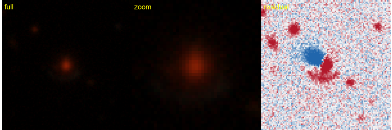
Figure 44: #49 s_102952_10164 — RA 334.8017, Dec -43.8098; grade B , tier-1 p_{\text{lens}} 0.42, v3blend8 0.85. KNOWN — DES: DES J221912.39-434835.1, 0.01'' (lineage).
