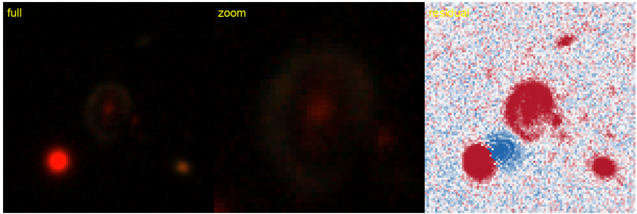
Figure 33: #30 s_61472_9399 — RA 359.5200, Dec -54.6765; grade B , tier-1 p_{\text{lens}} 0.50, v3blend8 0.88. KNOWN — DES: DES J235804.95-544034.4, 1.73'' (SIMBAD).
