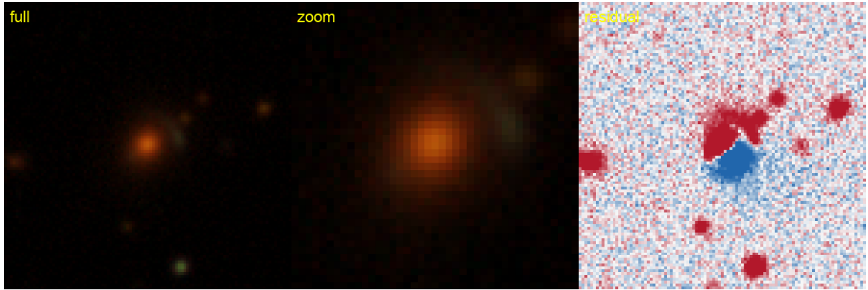
Figure 72: #41 s_90098_8002 — RA 107.1696, Dec -46.7832; grade B , tier-1 p_{\text{lens}} 0.45, v3blend8 0.83. NEW — new to the DESI lens-finders, the DES/AGEL/CASSOWARY searches, and the NED/SIMBAD literature.
