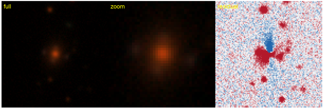
Figure 45: #50 s_90804_9850 — RA 3.9284, Dec -46.6031; grade B , tier-1 p_{\text{lens}} 0.42, v3blend8 0.84. KNOWN — DES: DES J001542.79-463610.9, 0.16'' (SIMBAD).
