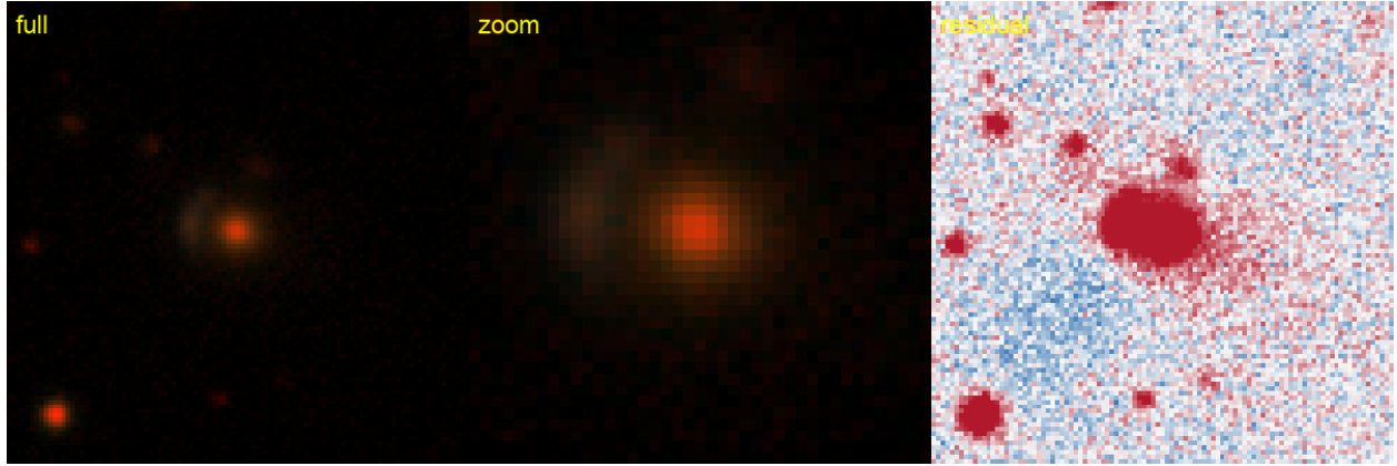
Figure 68: #28 s.23764.4161 — RA 132.6603, Dec -68.1876; grade B , tier-1 p_{\text{lens}} 0.55, v3blend8 0.79. NEW — new to the DESI lens-finders, the DES/AGEL/CASSOWARY searches, and the NED/SIMBAD literature.
