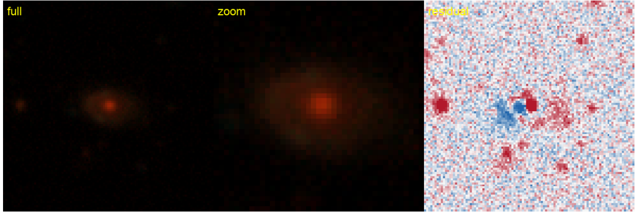
Figure 81: #64 s_188312_3322 — RA 33.2537, Dec -25.3945; grade B , tier-1 p_{\text{lens}} 0.40, v3blend8 0.76. NEW — new to the DESI lens-finders, the DES/AGEL/CASSOWARY searches, and the NED/SIMBAD literature.
