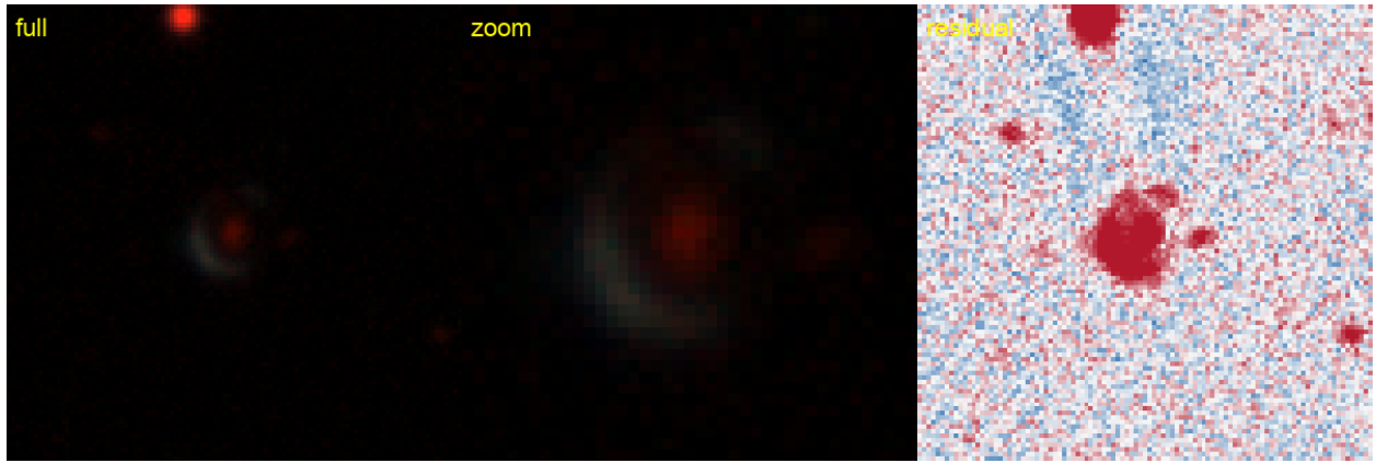
Figure 12: #3 s_181942.4122 — RA 61.6016, Dec -26.7733; grade A , tier-1 p_{\text{lens}} 0.87, v3blend8 0.86. KNOWN — DES: DES J040624.49-264625.0, 1.74'' (SIMBAD).
