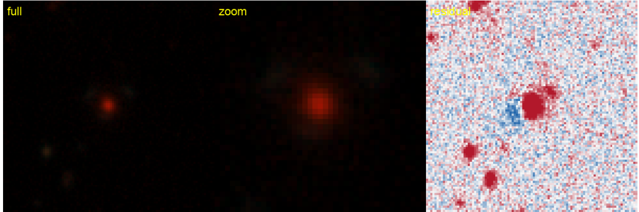
Figure 17: #8 s_80200_6872 — RA 15.4919, Dec -49.2940; grade A , tier-1 p_{\text{lens}} 0.78, v3blend8 0.88. KNOWN — DES: DES J010158.03-491738.1, 0.12'' (SIMBAD).
