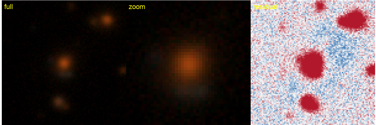
Figure 26: #21 s_290988_3355 — RA 217.1429, Dec -7.0963; grade B , tier-1 p_{\text{lens}} 0.58, v3blend8 0.75. KNOWN — Huang+2020: DESI-217.1429-07.0963, 0.15'' (lineage).
