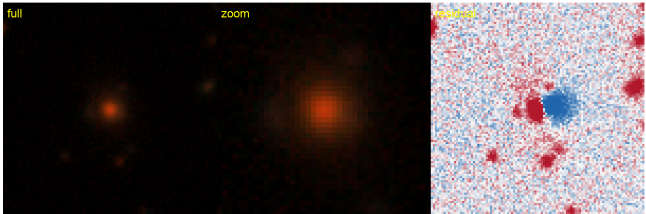
Figure 25: #20 s_111542_5062 — RA 4.8181, Dec -41.6141; grade B , tier-1 p_{\text{lens}} 0.60, v3blend8 0.77. KNOWN — DES: DES J001916.32-413650.5, 0.22'' (SIMBAD).
