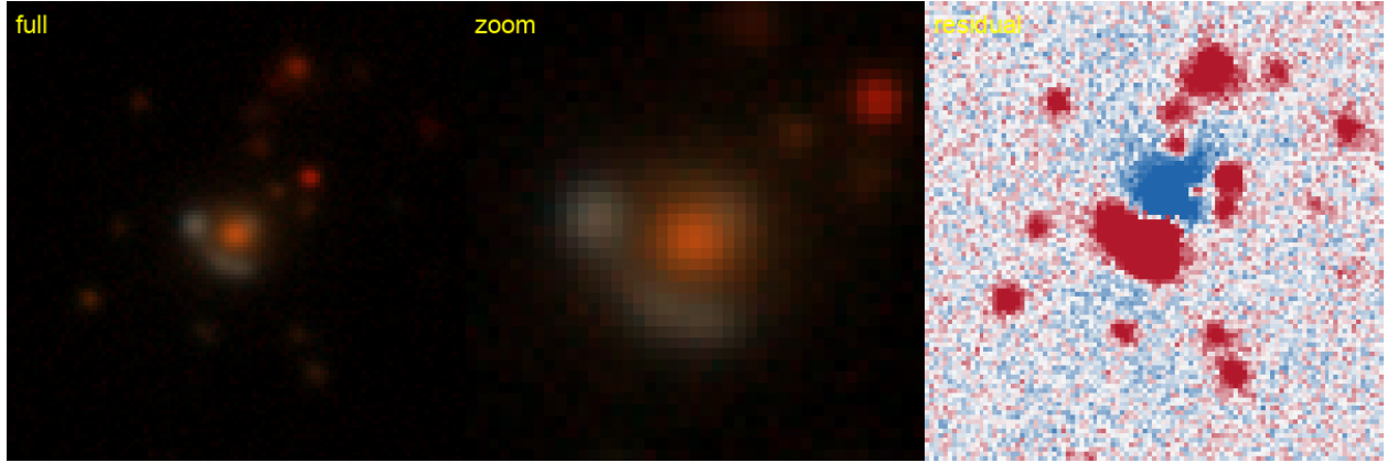
Figure 50: #59 s_107312.5223 — RA 23.8451, Dec -42.5398; grade B , tier-1 p_{\text{lens}} 0.40, v3blend8 0.85. KNOWN — DES: [DBL2017] DES J0135-4232 (A), 0.18'' (SIMBAD).
