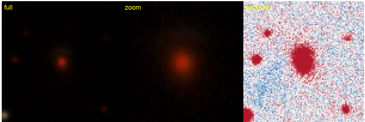
Figure 57: #69 s.225679.7025 — RA 25.7203, Dec -18.5211; grade B , tier-1 p_{\text{lens}} 0.38, v3blend8 0.79. KNOWN — AGEL: AGEL J014253-183116 system, 0.94'' (SIMBAD).
