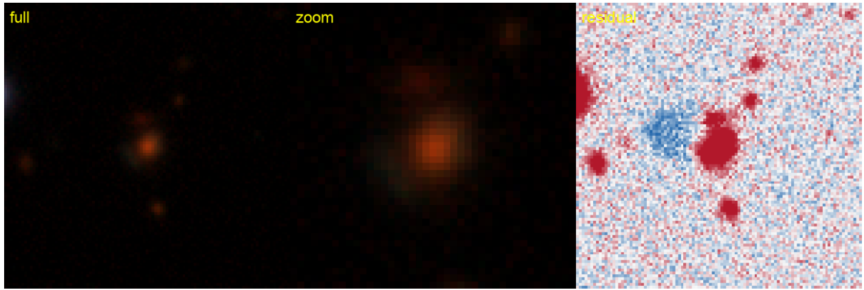
Figure 30: #26 s_159172_8702 — RA 37.5699, Dec -31.3669; grade B , tier-1 p_{\text{lens}} 0.55, v3blend8 0.82. KNOWN — DES: DES J023016.77-312200.8, 0.07'' (SIMBAD).
