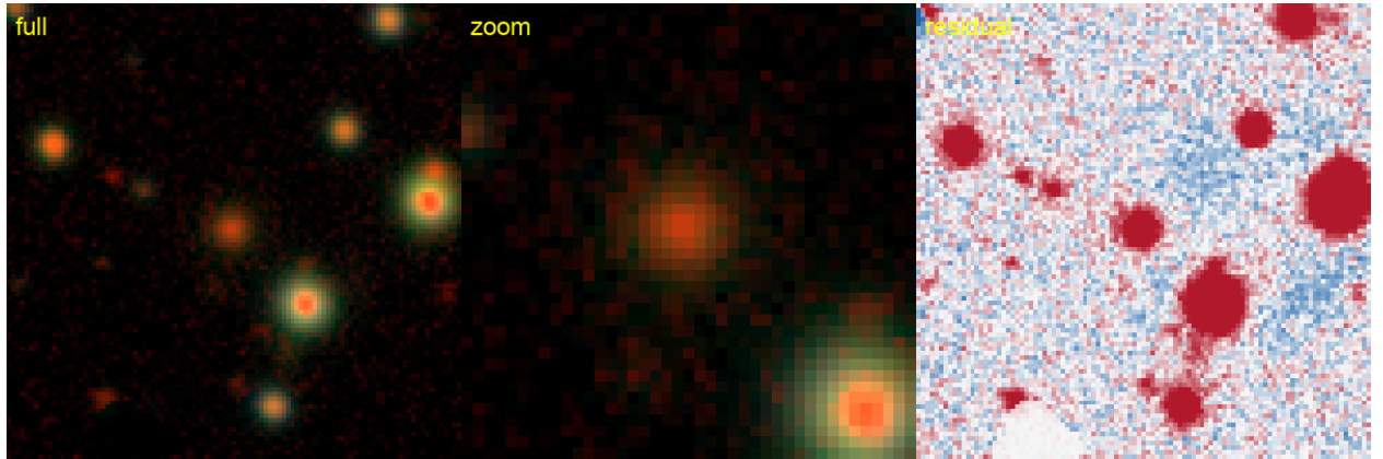
Figure 76: #46 s_32666_26056 — RA 248.6090, Dec -64.5569; grade B , tier-1 p_{\text{lens}} 0.45, v3blend8 0.73. NEW — new to the DESI lens-finders, the DES/AGEL/CASSOWARY searches, and the NED/SIMBAD literature.
