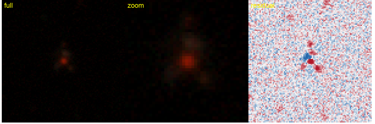
Figure 74: #44 s_426295_4804 — RA 182.0229, Dec +16.6326; grade B , tier-1 p_{\text{lens}} 0.45, v3blend8 0.79. NEW — new to the DESI lens-finders, the DES/AGEL/CASSOWARY searches, and the NED/SIMBAD literature.
