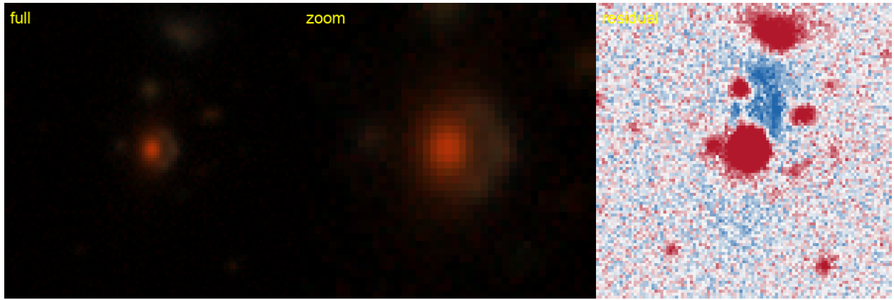
Figure 42: #47 s_156771.3446 — RA 54.3219, Dec -31.8704; grade B , tier-1 p_{\text{lens}} 0.42, v3blend8 0.89. KNOWN — AGEL: AGEL J033717-315214 system, 0.99'' (SIMBAD).
