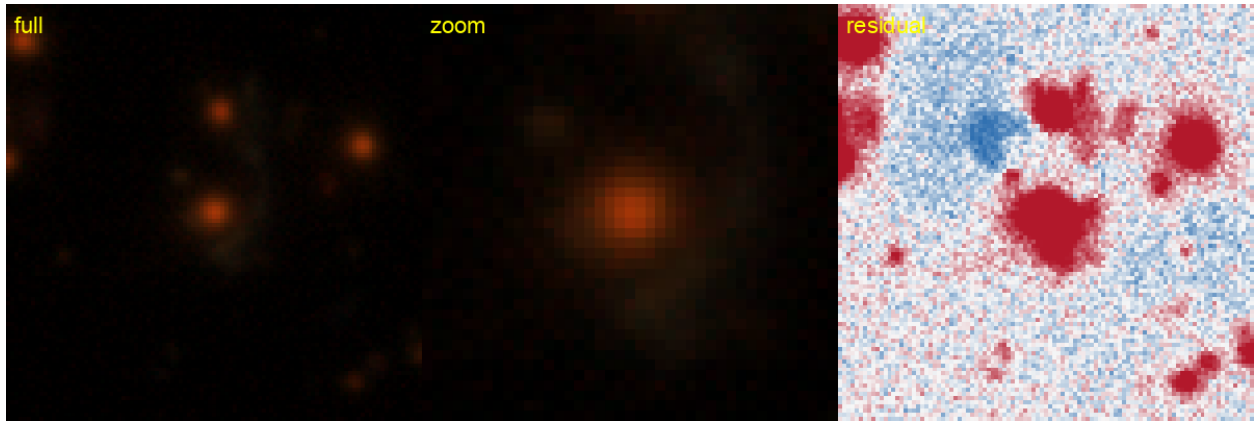
Figure 39: #39 s_194944.4494 — RA 59.2045, Dec -24.1447; grade B , tier-1 p_{\text{lens}} 0.45, v3blend8 0.85. KNOWN — DES: DES J035649.05-240841.1, 0.28'' (SIMBAD).
