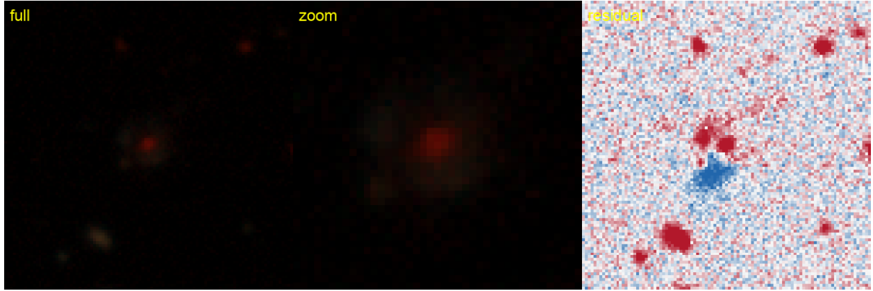
Figure 35: #33 s_43736.6056 — RA 67.3945, Dec -60.1905; grade B , tier-1 p_{\text{lens}} 0.50, v3blend8 0.83. KNOWN — DES: DES J042934.66-601126.3, 0.35'' (SIMBAD).
