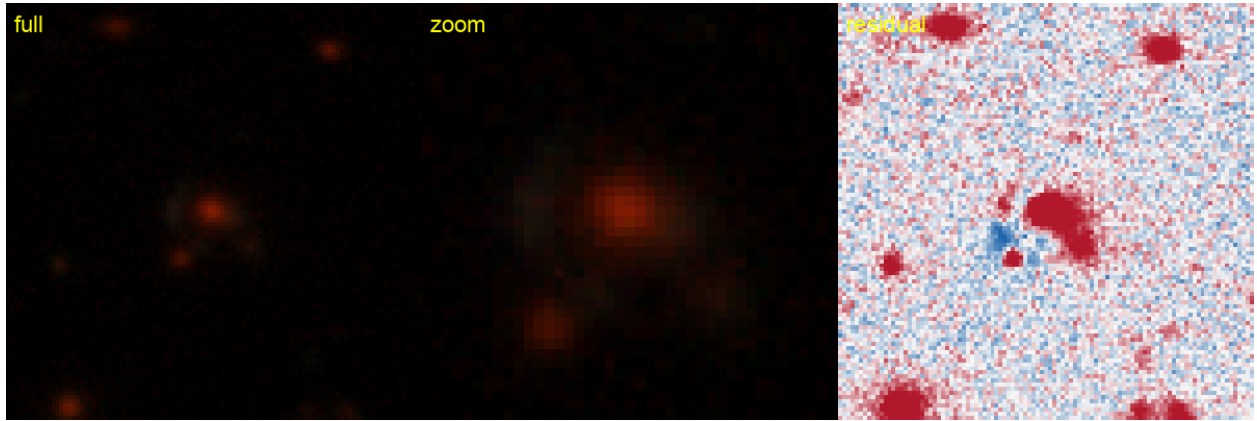
Figure 78: #53 s_242312_4967 — RA 50.3567, Dec -15.5010; grade B , tier-1 p_{\text{lens}} 0.40, v3blend8 0.90. NEW — new to the DESI lens-finders, the DES/AGEL/CASSOWARY searches, and the NED/SIMBAD literature.
