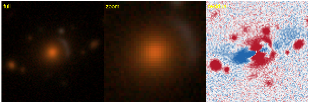
Figure 19: #11 s_292418_3907 — RA 216.8280, Dec -6.7541; grade B , tier-1 p_{\text{lens}} 0.62, v3blend8 0.89. KNOWN — Huang+2020: DESI-216.8280-06.7541, 0.15'' (lineage).
