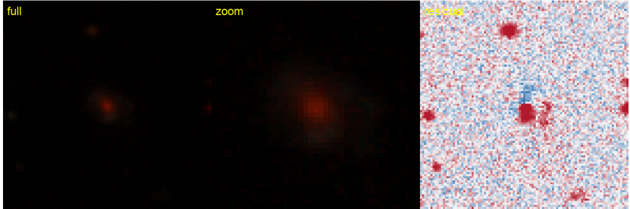
Figure 29: #25 s_61626_1035 — RA 65.1782, Dec -54.3770; grade B , tier-1 p_{\text{lens}} 0.55, v3blend8 0.87. KNOWN — DES: DES J042042.76-542237.4, 0.18'' (SIMBAD).
