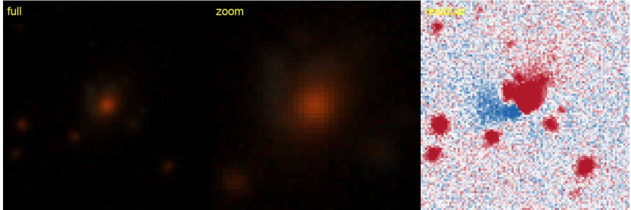
Figure 53: #62 s_256199_9097 — RA 29.6819, Dec -13.0258; grade B , tier-1 p_{\text{lens}} 0.40, v3blend8 0.78. KNOWN — DES: DES J015843.66-130132.8, 0.18'' (SIMBAD).
