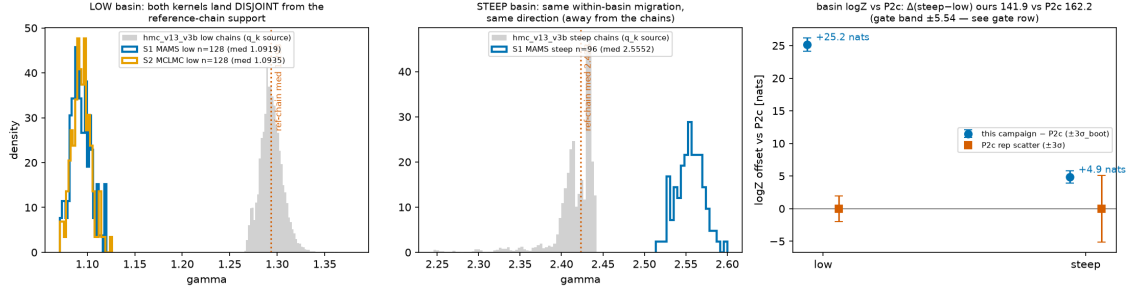
Figure 15: B5 both-basin \lambda = 1 posterior overlay on the 74-d bimodal target foundry_v3b74 , drawn before any gate math per house rule (jobs 56006049 / 56251555 / 56006052). The low basin’s two independent mutation kernels agree on location (MAMS \gamma_{\text{eqw}} = 1.0919 , MCLMC 1.0935); the steep basin sits at 2.5552. Source: data/b5_gate_eval.json .
