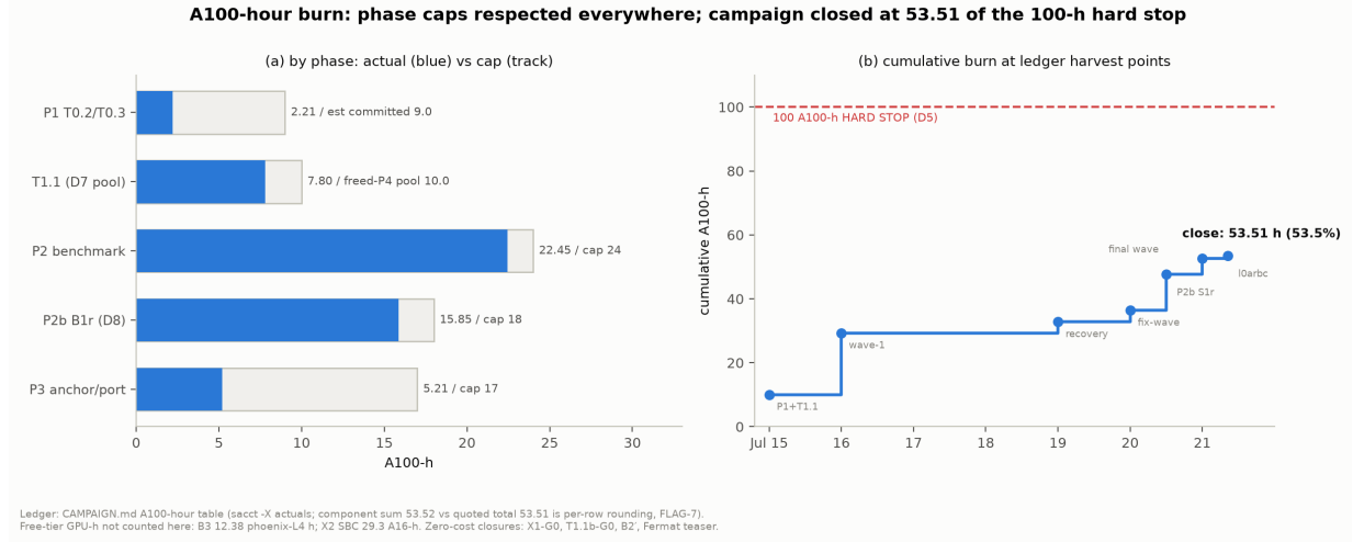
Figure 21: A100-hour burn. (a) Actual vs. cap by phase — every fence respected (P1 2.21, T1.1 7.80 of the D7-freed 10-h pool, P2 22.45/24, P2b 15.85/18, P3 5.21/17). (b) Cumulative burn at the ledger’s harvest points (events in ledger order; sub-day x -offsets are display-only), closing at 53.51 of the 100-h hard stop; the 53.52 component sum is per-row sacct rounding (flagged, not smoothed). Free-tier GPU-h (B3: 12.38 L4-h; X2: 29.3 A16-h) are additional and uncounted here. Zero-cost closures: X1-G0, T1.1b, B2’, the Fermat teaser. Source: CAMPAIGN.md A100-hour ledger (append-before-read protocol).
