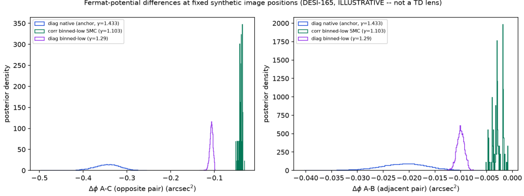
Figure 12: Fermat-potential difference posteriors for an opposite and an adjacent synthetic image pair under the three noise-model posteriors (diagonal-native anchor, diagonal-binned-low, correlated-binned-low). Illustrative only (see the triple disclaimer): the noise-model choice moves \Delta\phi by 61–88% where \sim 1\% is the TDCOSMO-relevant scale. Source: data/fermat_dt_teaser.json .
