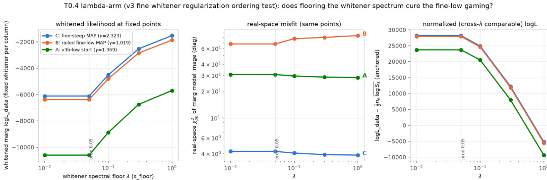
Figure 8: T0.4-2 \lambda -arm: whitened and normalized likelihoods of the three frozen points vs. spectrum floor \lambda . The gaming inversion is flat in \lambda (flooring does not cure it) while the normalized likelihood rejects the floored kernels by 3.2k–33k nats per point. Source: data/t04_lambda_arm.json .
