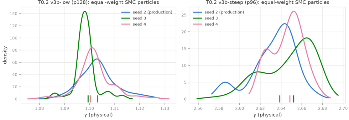
Figure 4: T0.2 seed-repeat certification: low- and steep-basin \gamma posteriors for seeds \{2, 3, 4\} (production tempered SMC, v3b correlated likelihood). The money number is \gamma = 1.1032 \pm 0.0086 ( \sigma_{\text{tot}} , seed scatter folded in); the basin preference \Delta \log Z(\text{steep} - \text{low}) \approx -29 to -32 nats is seed-stable. Source: data/t02_t03_gate_eval.json .
