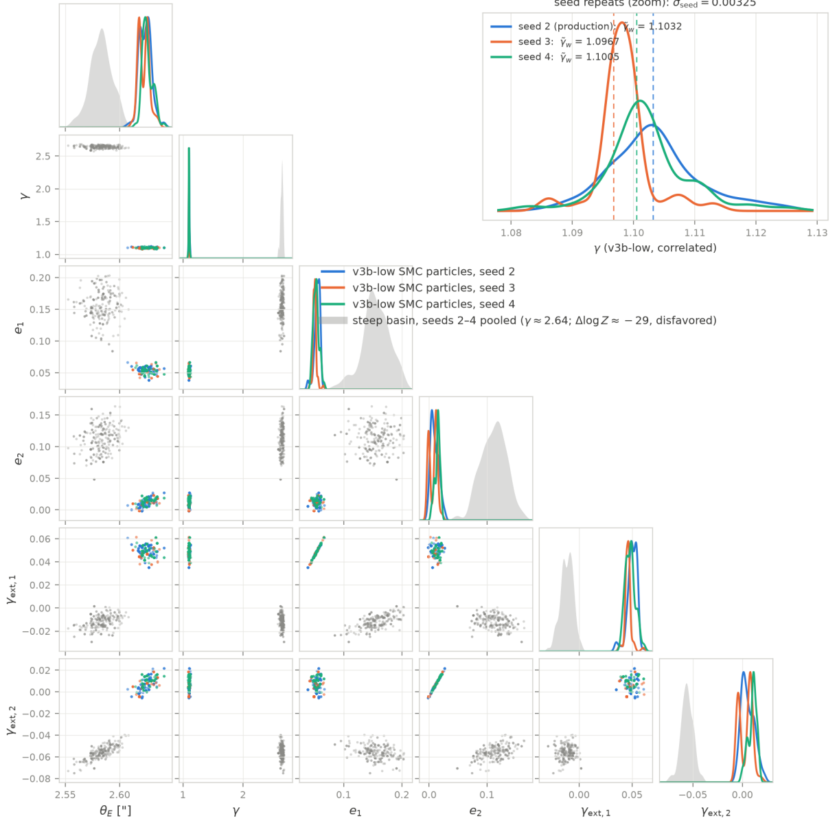
Figure 2: Posterior corner of the six mass parameters ( \theta_E , \gamma , e_1 , e_2 , \gamma_{\text{ext},1} , \gamma_{\text{ext},2} ) from the stored equal-weight v3b-low correlated SMC particles, seeds \{2, 3, 4\} overlaid — the SMC convergence visual (SMC has no \hat{R} ; the seed-repeat spread \sigma_{\text{seed}} = 0.00325 plus the per-stage ESS/acceptance diagnostics of Table 2 are the analogues). Grey: the steep basin (seeds 2–4 pooled, \gamma \approx 2.64 ; evidence-disfavored by \approx 29 –32 nats). Inset: \gamma zoom with the per-seed weighted medians of record \{1.1032, 1.0967, 1.1005\} ; the equal-weight particle medians reproduce them to \leq 0.0027 , well inside \sigma_{\text{stat}} = 0.008 . Source artifacts: companion data/results/e2.v3b.low-smc.canary.fix.json (+ seed-3/4 repeats), data/t02.t03_gate_eval.json , data/rfig_modeler_params.npz .
