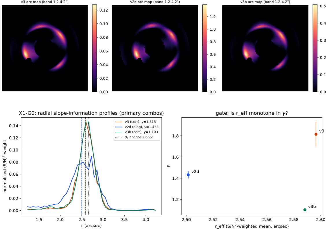
Figure 5: X1-G0 entry-gate kill. Top: arc-brightness \times (S/N)^2 slope-information weight maps for the three products. Bottom: radial (S/N)^2 slope-information profiles (left) and the \gamma -vs- r_{\text{eff}} gate panel (right): no monotone ordering exists (24/24 variants), and the fine/binning pair constrains the slope at the same radius ( \Delta r_{\text{eff}} \approx 0.008'' ) while disagreeing by \Delta\gamma = 0.71 . Source: data/x1_g0_effective_radii.json .
