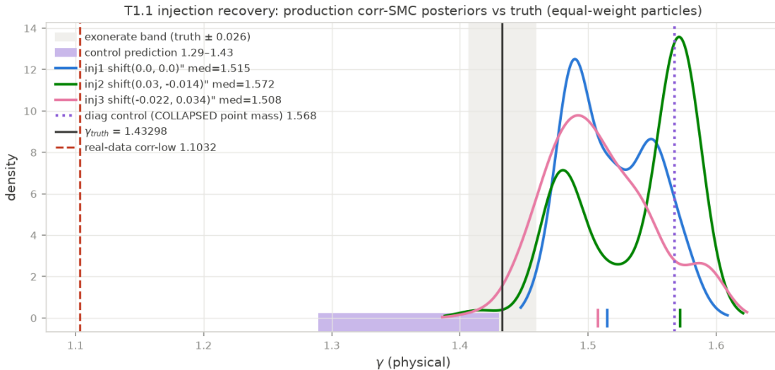
Figure 10: T1.1 injection-recovery: recovered \gamma posteriors for the three correlated injections and the diagonal control vs. the injected truth 1.4330 and the pre-registered zones. All arms land high (scene residue absorption); the control is both out-of-window and degenerate. Source: data/t11_gate_eval.json .
