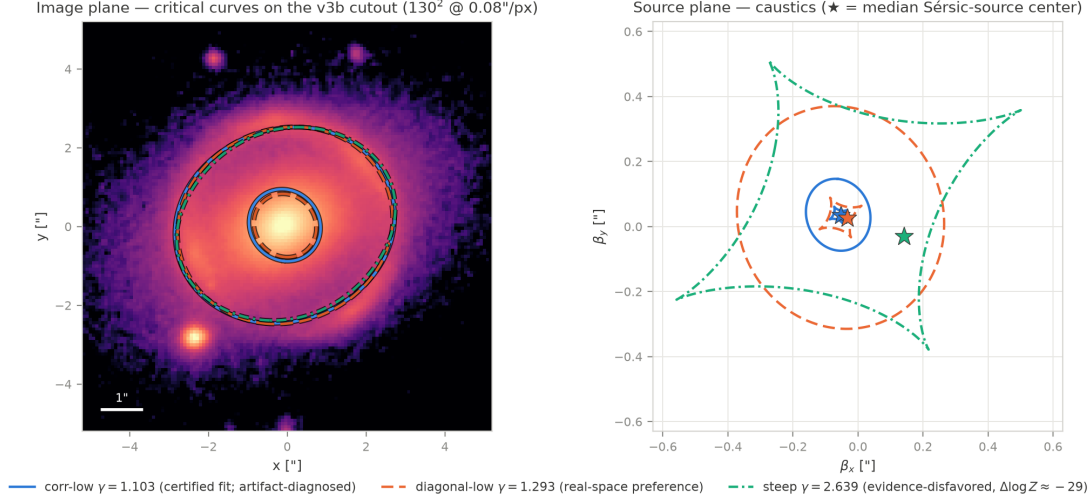
Figure 1: Critical curves (lens plane, over the v3b binned cutout, asinh stretch) and caustics (source plane; stars mark the median Sérsic-source centers) for the three posterior-median mass models, following the critical-curve/caustic display conventions of the team’s GIGA-LENS discovery paper (Gu et al., 2022): corr-low \gamma = 1.103 (the certified but artifact-diagnosed correlated fit), diagonal-low \gamma = 1.293 (the real-space preference), and steep \gamma = 2.639 (evidence-disfavored, \Delta \log Z \approx -29 ). Scale sanity: the outer critical curve’s median radius matches each model’s \theta_E to < 5\% (money model: 2.632'' vs. \theta_E = 2.624'' ), and the two shallow ( \gamma < 2 ) models show the expected inner radial critical curve and caustic. Deflections from the vendored scene API EPL(50)+shear at the certified conventions; source artifact data/rfig_modeler.params.npz .
