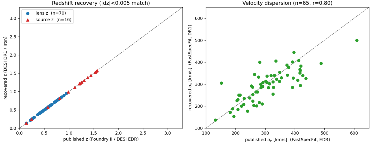
DESI Strong Lens Foundry II - DR1 reproduction of Table 2
