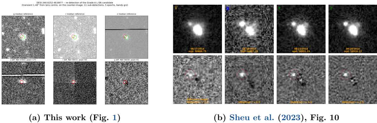
Figure 4: Re-detection of the Grade-A L-SN on the counter-image. (a) This work: g/r/z median references (top) and from-scratch B08 difference-image stamps (bottom) with the re-detected transient (group 26517) circled — an 11-sub-detection, 5-epoch, grz source 1.48'' from the lens centre. (b) The published detection exposures for the same system (top: single-pass images; bottom: SFFT difference images, red circle on the detected transient). Both isolate the transient on the \theta_E \approx 1.5'' counter-image. Panel (b) reproduced from Sheu et al. (2023) , their Fig. 10, for comparison.
