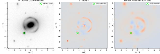
Figure 3. Detection of the nearby galaxy on the v2 residual map. A clear point-like positive residual at (\Delta\alpha, \Delta\delta) \approx (-2''.34, -2''.86) from the main-lens centroid is the signature of an unmodeled companion; including its light as two additional Sérsic components (v3→v4 onward) removes this feature.
