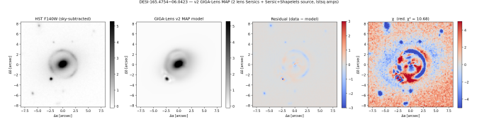
Figure 4. v2 MAP residual (data — model, in units of \sigma_{\text{bg}} ). The bright residual blob \sim 3'' southwest of the main lens is the signature of the nearby galaxy modeled in v3 onward (Figure 3).
