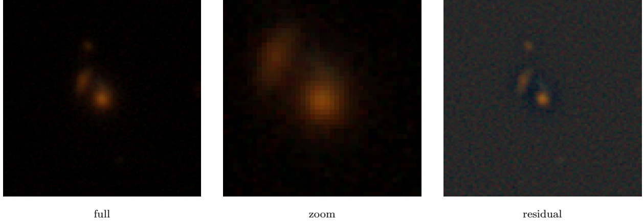
Figure 9: Views the agent inspected for DESI-124.2632+17.1177 (consensus D; this episode: agent grade D, p_{\text{lens}} = 0.05 , contaminant merger). A close pair of red galaxies that the CNN scored p_{\text{meta}} = 0.91 .
