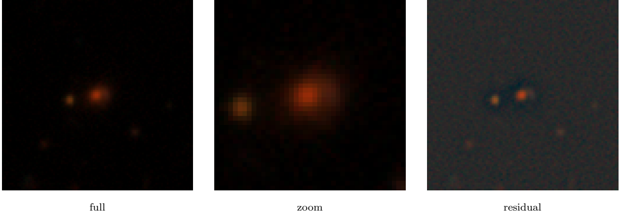
Figure 10: DESI grz views (1.3" seeing) rendered for DESI-029.0755–01.1297: a red core with a red companion that both DESI stages read as an LRG+companion (grade D). The blue arc is blended into the lens light at this resolution.
