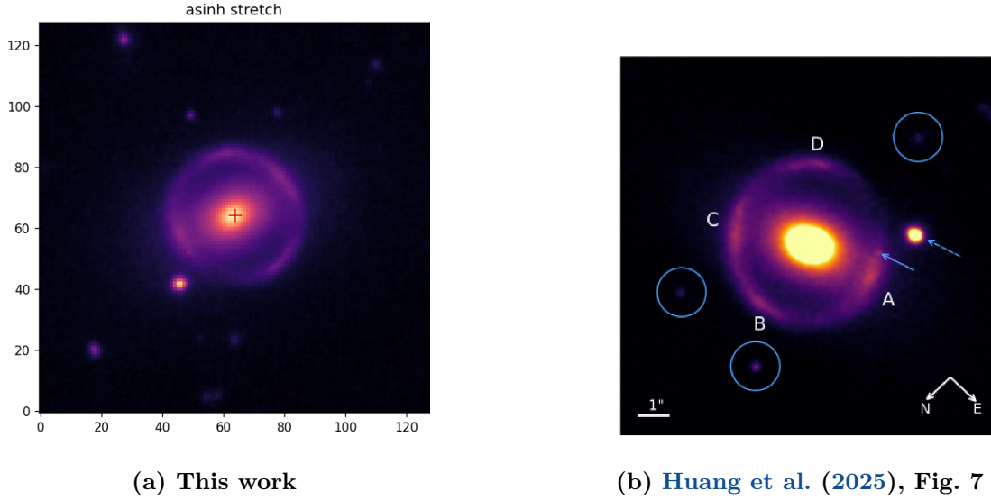
Figure 10: HST WFC3/F140W cutout of DESI-165.4754-06.0423. (a) This work: the asinh-stretched science cutout at 0.13 \text{ pix}^{-1} (the centre panel of report Figure 1), showing the tangential arc system, the bright central deflector, and the nearby companion at lower-left. (b) The published F140W image of the same system with the four lensed images labelled A–D and the companion arrowed. We reprocess the same GO-15867 exposure from MAST; the arc geometry, deflector, and companion position match. Panel (b) reproduced from Huang et al. (2025), their Fig. 7, for comparison.
