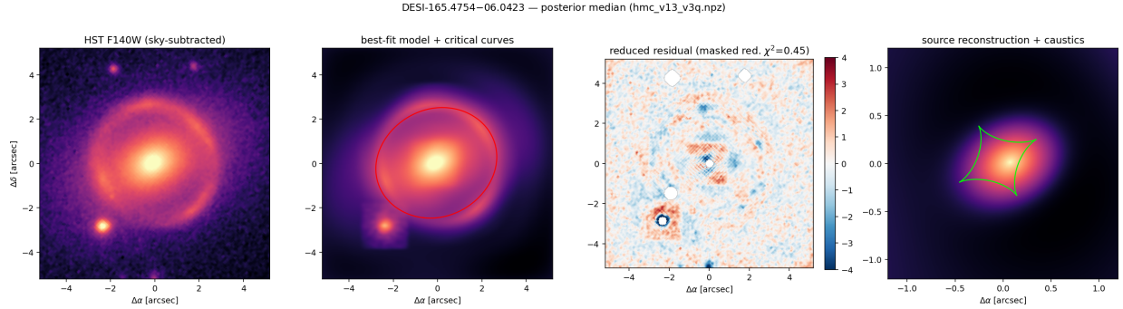
Figure 7: Same, from the fine-scale (v3, 0.004) posterior median ( \gamma_{\text{EPL}} = 2.585 ): the masked residual is structureless, and the nominal \chi^2_\nu = 0.45 later proved to be a noise-calibration artifact — under the recalibrated (honest) noise, this same model evaluates to \chi^2 \simeq 0.92 (§8.5). The steep-slope mode has a single (tangential-only) critical curve; the \gamma_{\text{EPL}} difference between the two panels persists at 0.008 as an explicit bimodality (§8.5).
