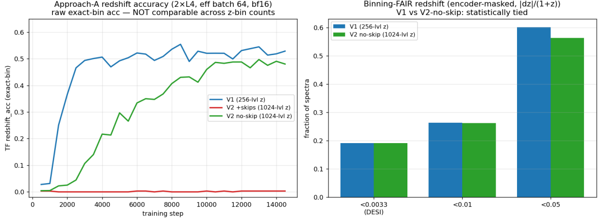
Figure 2: Left: TF redshift-accuracy trajectories (V2+skips flat at zero from codebook collapse; raw exact-bin, not comparable across redshift-bin counts). Right: binning-fair honest |\Delta z|/(1+z) fractions—V1 and skip-free V2 are tied.
