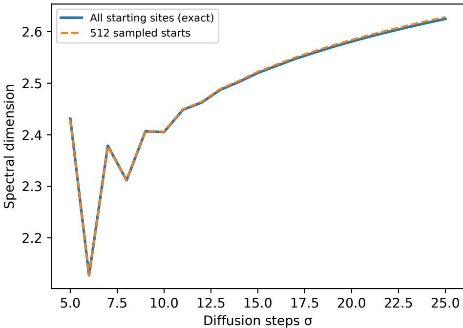
Short-time sampling precision
