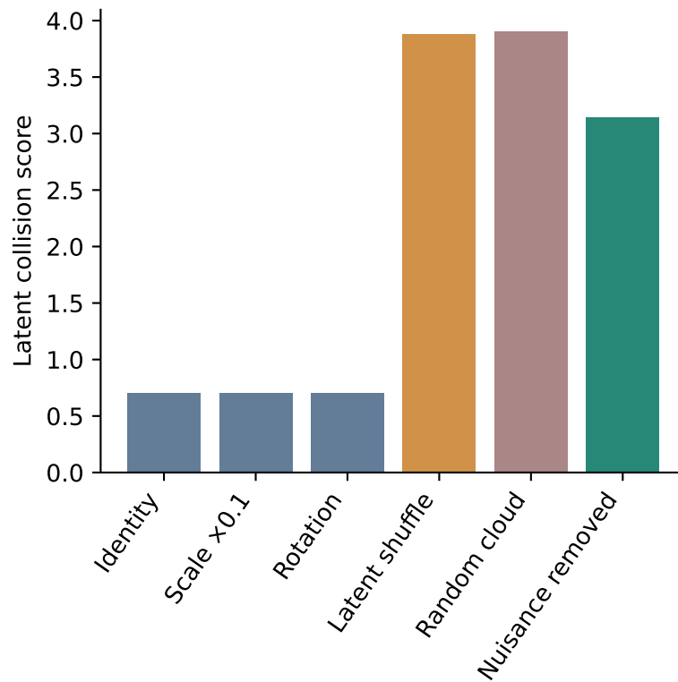
Known controls separate geometric structure from latent correspondence PH: 200 points, 3 subsamples, RMS normalized; these are untrained controls
