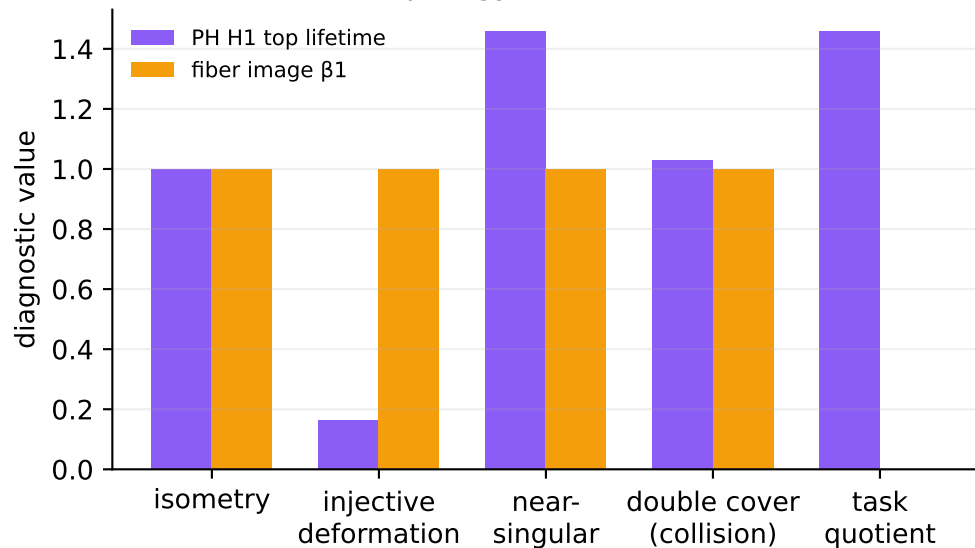
D. Metric topology vs. fiber identification
