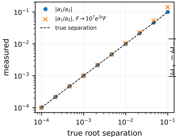
(a) scale-free diagnostic
