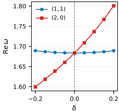
(a) m_1+m_2=2 multiplet
