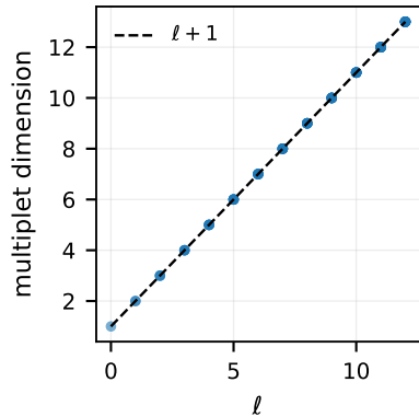
(c) dimension is \ell + 1 for every m
