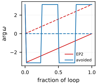
(c) monodromy
