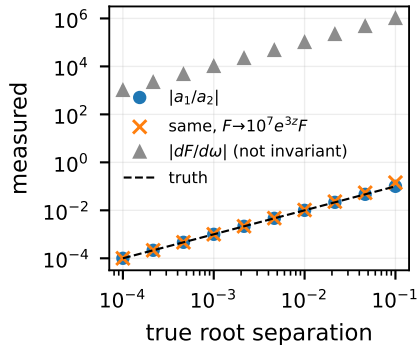
(a) invariance
