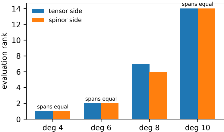
evaluation rank on common samples
