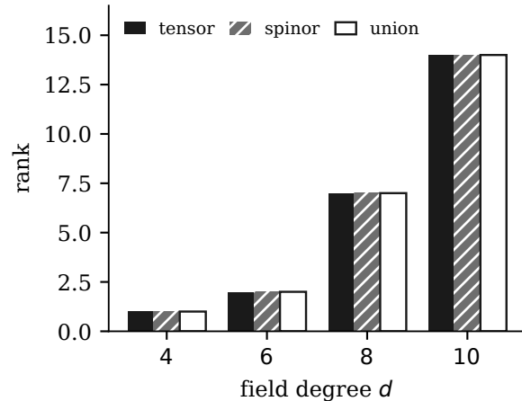
(c) tensor vs spinor
