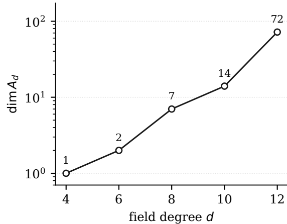
(a) invariant dimension
