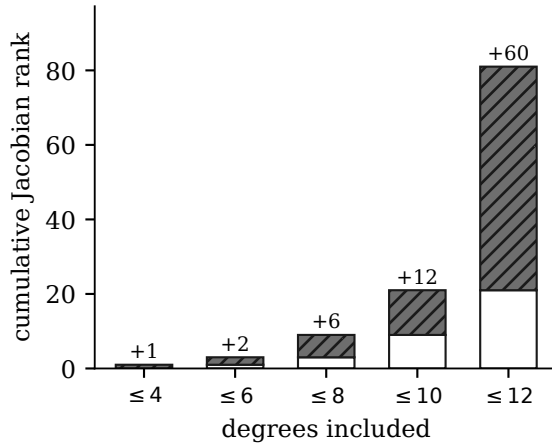
(b) rank growth to 81
