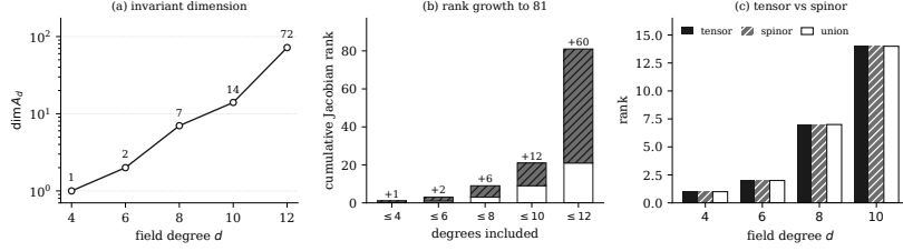
Figure 1. Degree-resolved tensor, spinor and union ranks. At every degree shown the three agree, so neither formulation sees an invariant the other misses.
