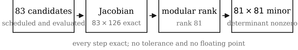
Figure 6. The certification pipeline, from the candidate family to a fixed explicit minor. No step uses floating point and no step uses a tolerance.
