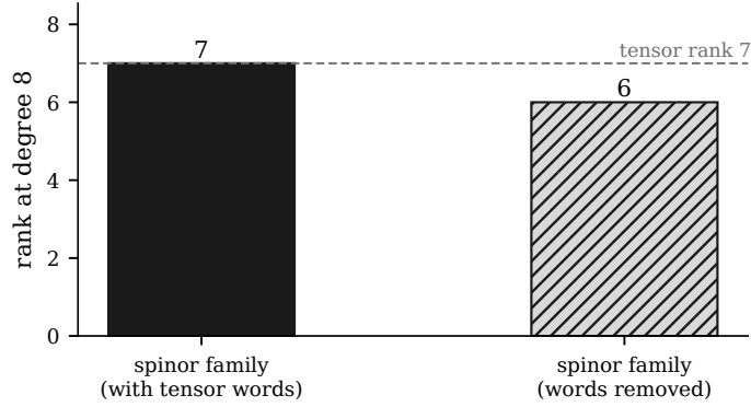
Figure 5. Degree-eight family ablation. Removing the tensor words from the spinor candidate family lowers the rank by one, so within this decomposition they are indispensable.
