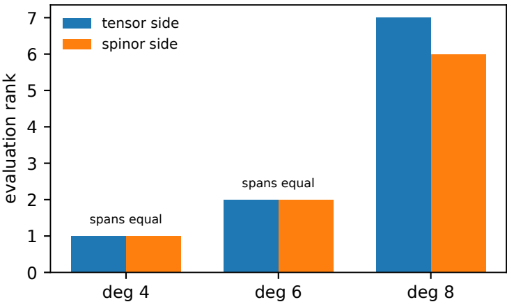
evaluation rank on common samples
