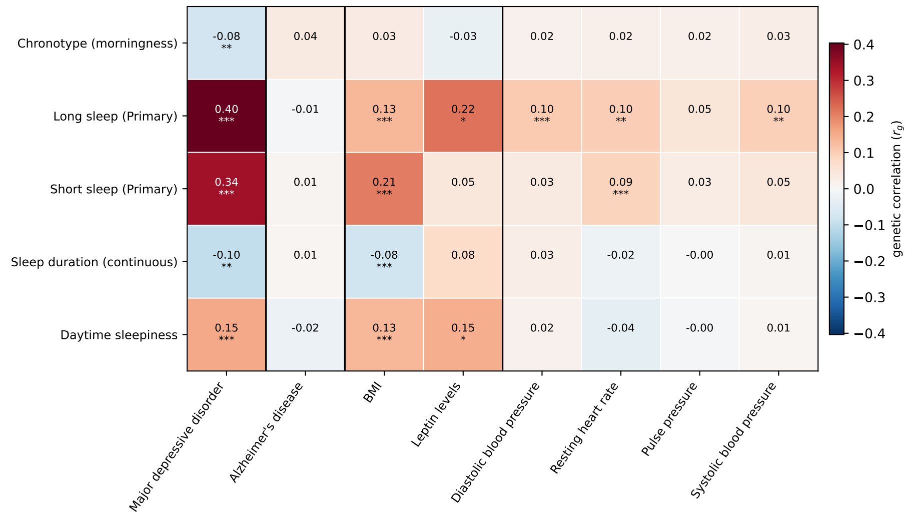
Sleep/circadian × disease genetic correlation (LDSC) * FDR<0.05 ** FDR<0.01 *** FDR<0.001
