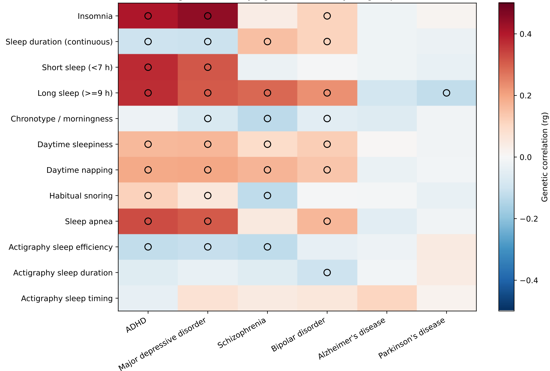
Original 396-family significance overlay (ring = q < 0.05 )
