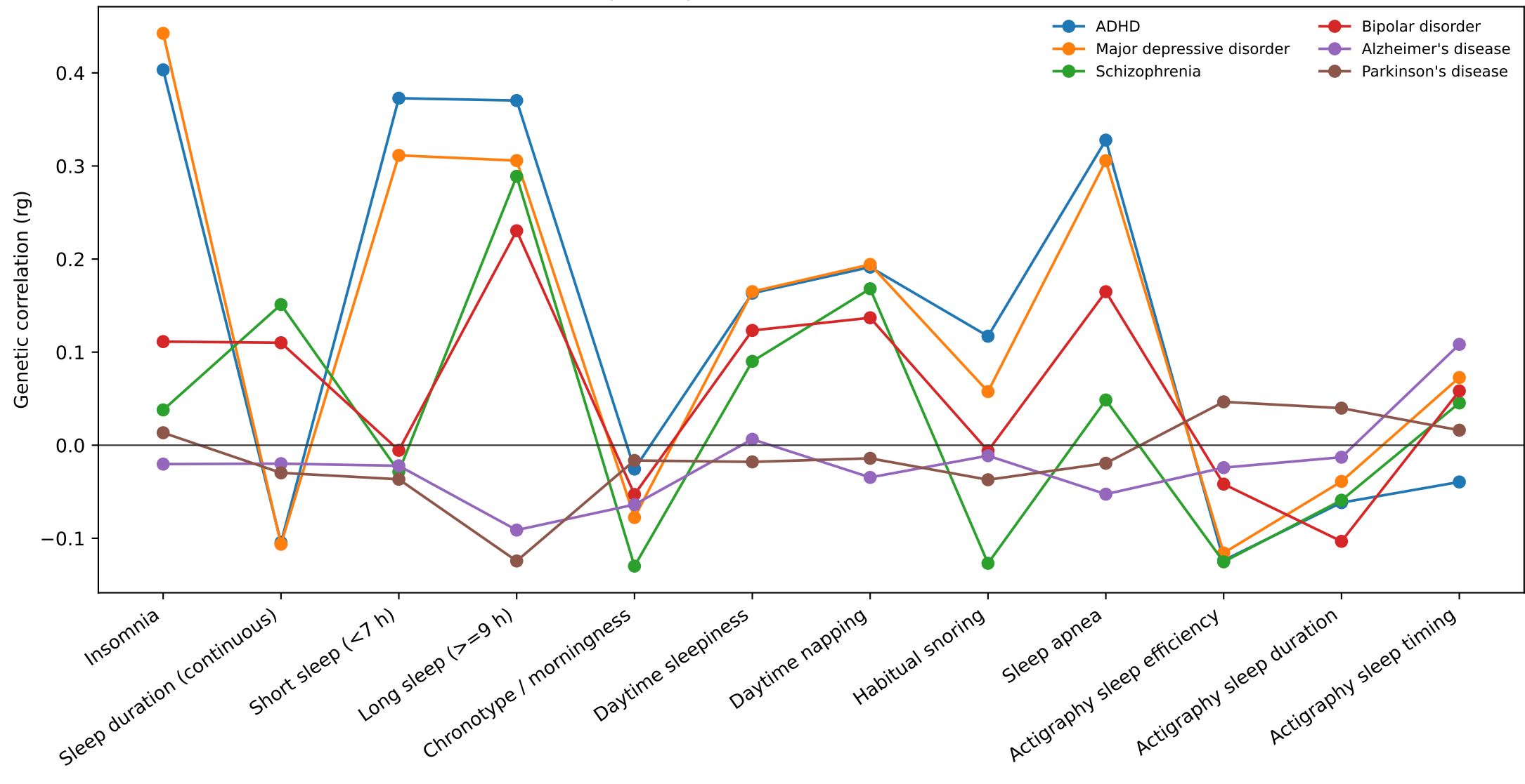
Sleep-trait profiles across six brain disorders
