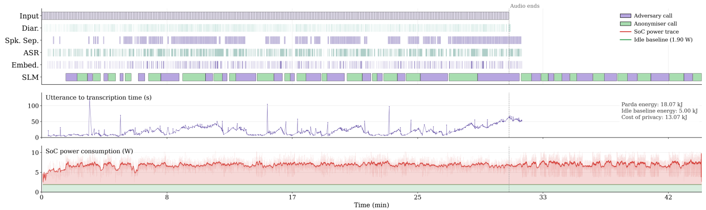
Fig. 11. Concurrent audio and SLM execution on Raspberry Pi 5. Top: per-stage execution timeline; middle: utterance-to-transcription delay; bottom: SoC power consumption.
