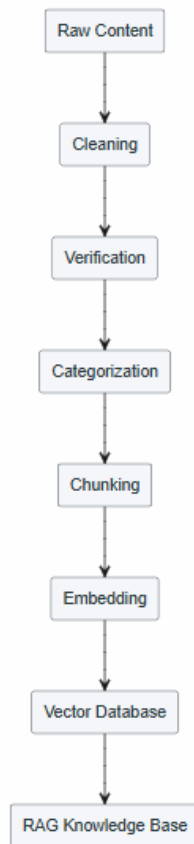
RAG Knowledge Base Ingestion Pipeline
