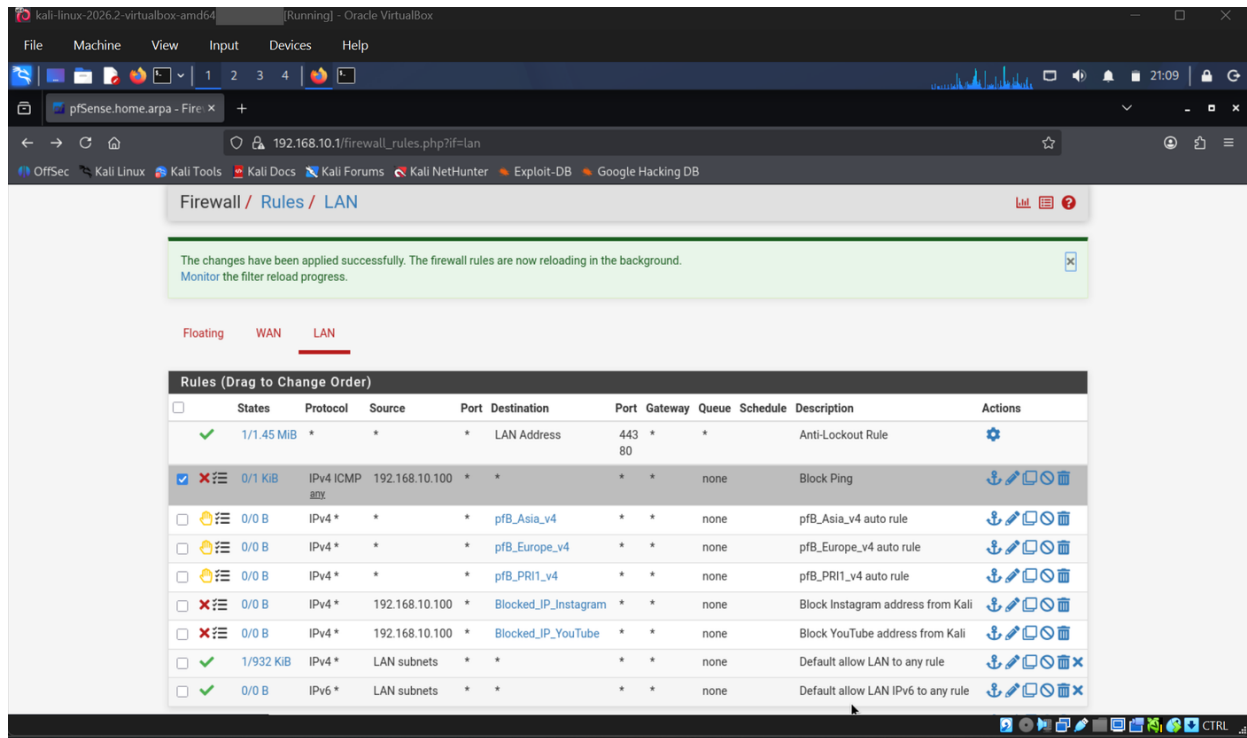
Figure 35: The full rule list on the inner interface, showing the hand-written rules, the new rule, and the rules generated by the filtering package
