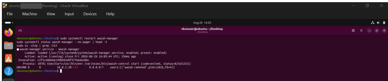
Figure 23: The system log listener confirmed bound, with wazuh-remoted holding port 514 on the manager's own address
