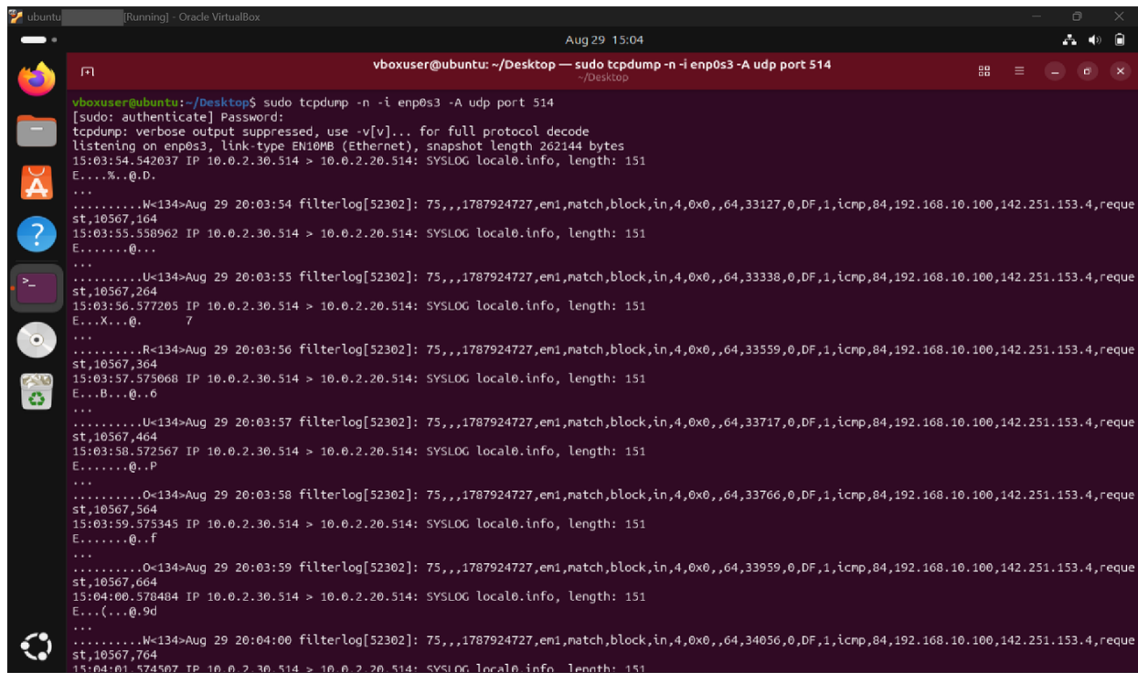
Figure 24: Firewall messages captured arriving at the manager on port 514, each one a single comma separated line
