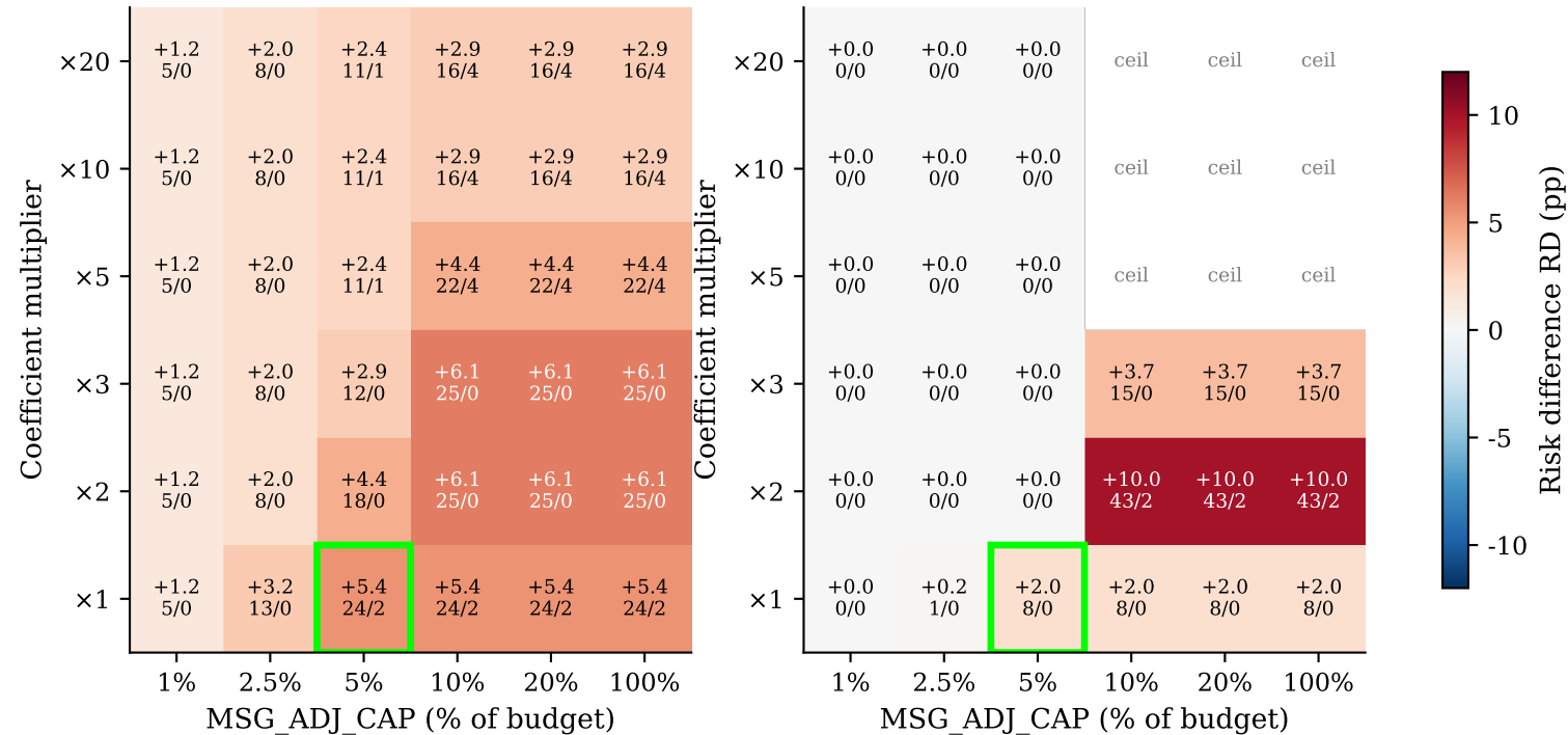
Figure 1. Cross-family behavioral steering phase diagram (original – factual, cell format: RD / discord + /discord - )
