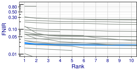
Neurotechnology+0122 is highlighted in blue, alongside all other algorithms in gray (lower is better).
