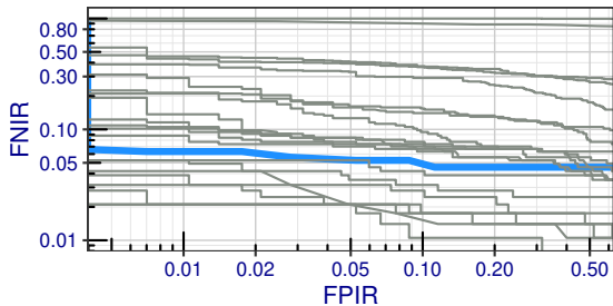
Neurotechnology+0128 is highlighted in blue, alongside all other algorithms in gray (algorithms target the lower-left).
