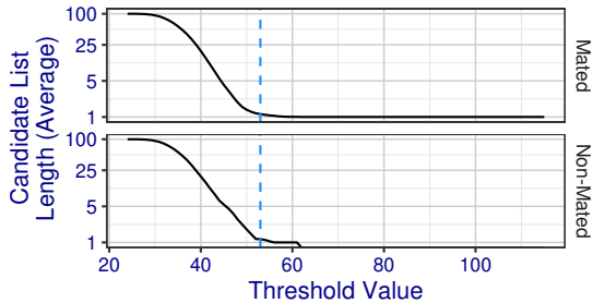
The similarity score indicated in blue is the threshold at which Neurotechnology+0128 achieves 10% FPIR.
