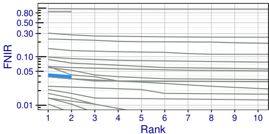
Neurotechnology+0128 is highlighted in blue, alongside all other algorithms in gray (lower is better).
